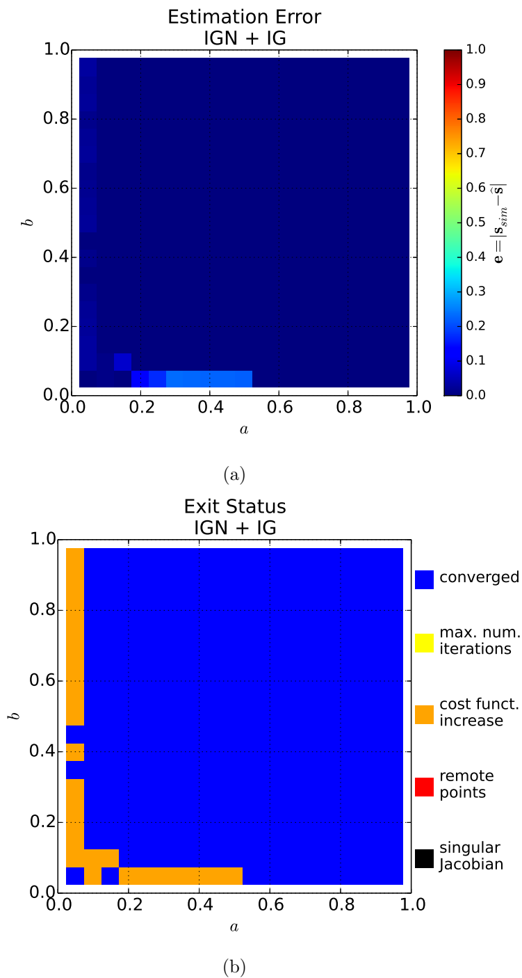
Figure 3.20: Simulation results for the improved Gauss-Newton algorithm without initial guess (IGN + IG). (a) the feature vector estimation error is represented in color scale. (b) the algorithm exit status is depicted in color code.
