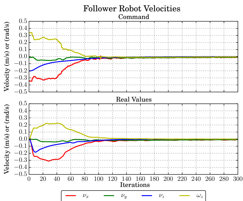
Figure 4.18: Simulation results for a control law using full 3 \times 4 interaction matrix. (a) tether shape and (b) follower robot velocity evolution. The tether desired shape is given by H_2^* = 0.15 m, \alpha_2^* = 30^\circ and \Delta H_2^* = 0.20 m.
