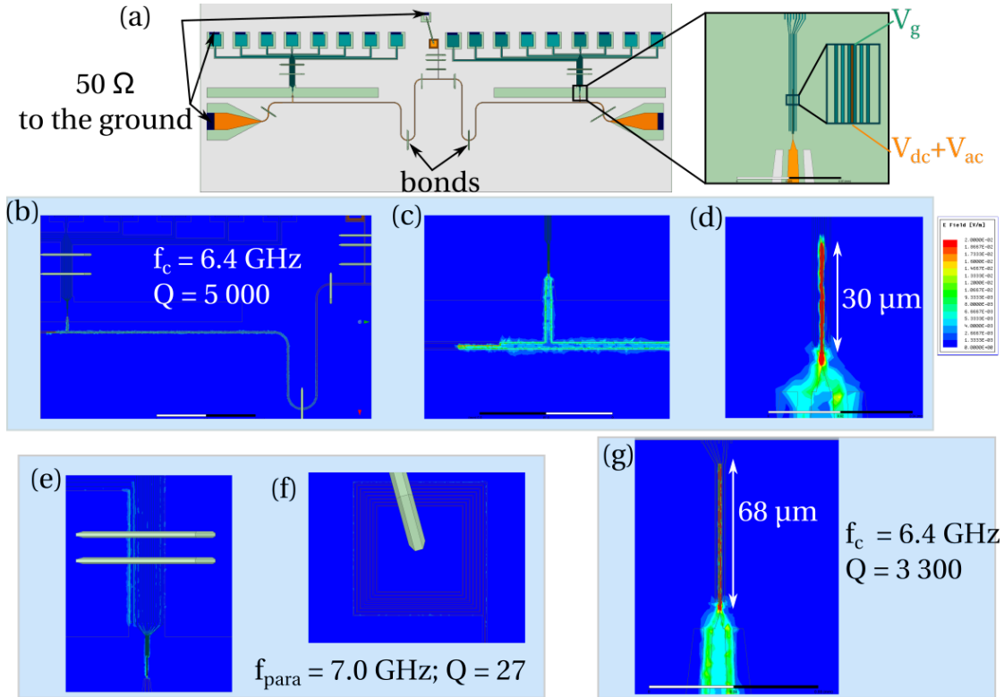
FIGURE 3.5: Simulations of the influence of a galvanic DC pad on the cavity mode: (a) Large-scale drawing of the best cavity geometry tested. The ground plane are represented in light green, the SiO 2 in light green, the DC lines in green and the cavity central conductor and input/output ports in orange. (b) Electric field magnitude for the CPW mode ( f_c = 6.4\text{GHz} , Q = 5000 ), on several regions : the center of the cavity, the input capacitance and the CNT circuit. (e, f) Parasitic mode at f_{\text{para}} = 7\text{GHz} , oscillating in the DC lines. (g) CPW mode for the same geometry, with a larger coupling capacitance between the DC circuit and the cavity.
