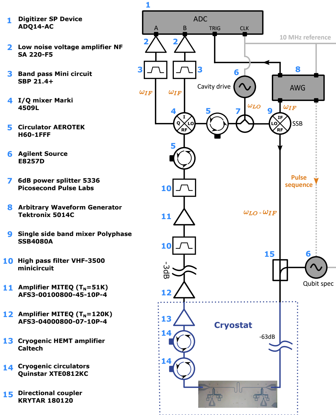
FIGURE 3.6: Schematic of the RF measurement setup
