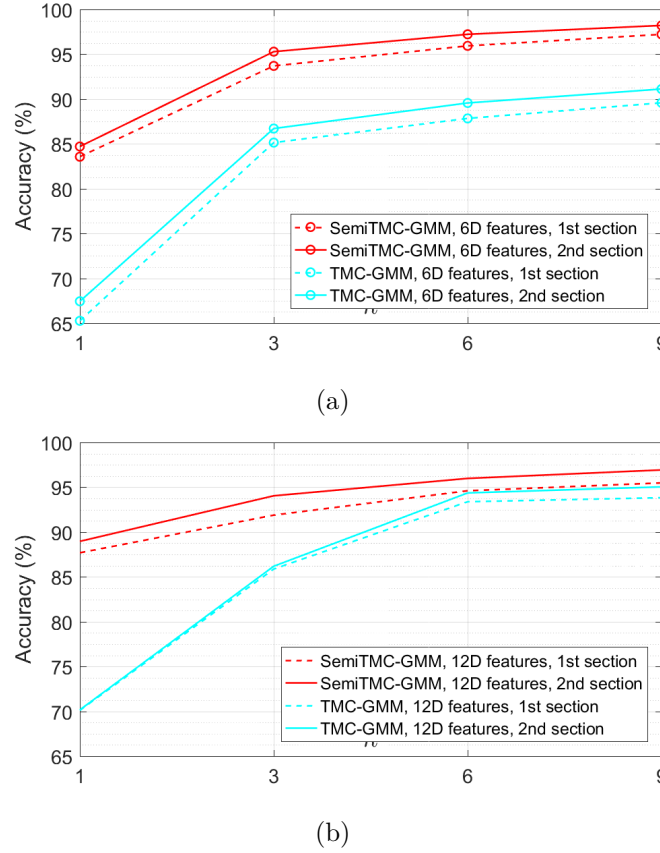
Figure 5.8: The on-line mode recognition accuracy of the two experiment sections in our own dataset, according to different GMM mixture number \kappa . (a): using 6D features; (b): using 12D features.
