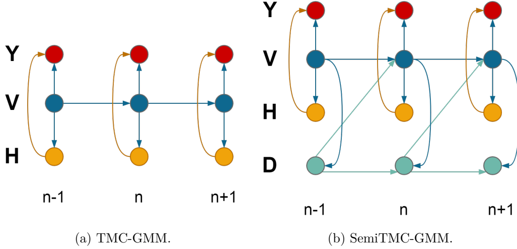
Figure 5.1: Dependency graph.
