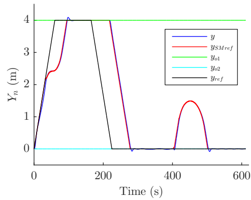
FIGURE 4.19 – Surge movement as a function of time.
