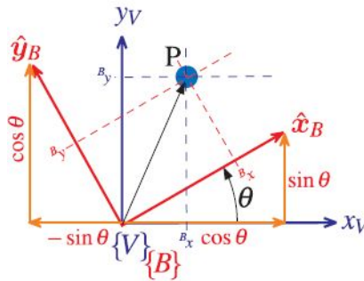
FIGURE 2.4 – Auxiliary coordinate frame
