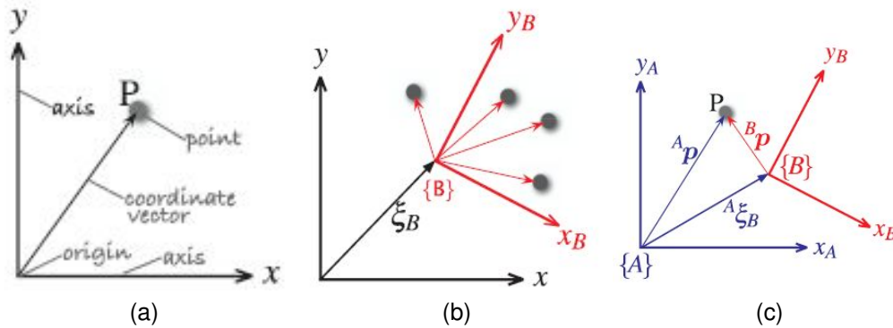
FIGURE 2.1 – Coordinate vectors
