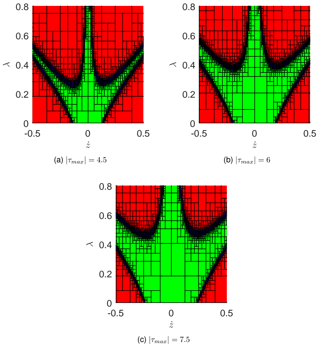
FIGURE 6.2 – SM subpaving analysis for an exact modeling of the system. Green : satisfaction of SM conditions, Red : no satisfaction, Blue : not determined
