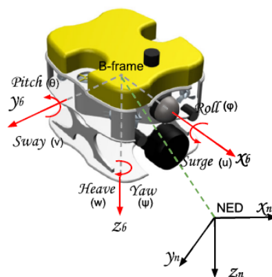
FIGURE 3.2 – Ciscrea's coordinate systems
