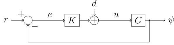
FIGURE 5.2 – Control scheme
