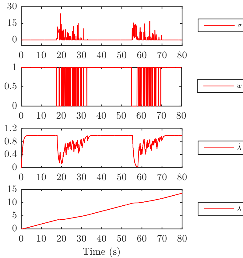
FIGURE 3.18 – Experimental SMRC signals
