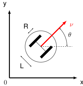
FIGURE 4.4 – Reference frame
