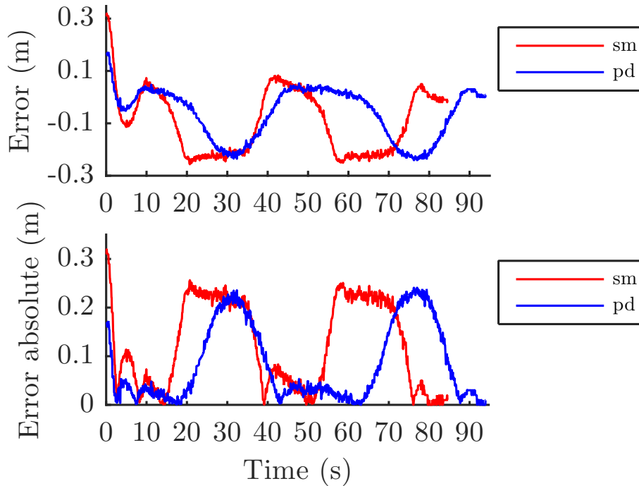
FIGURE 3.17 – Experimental path error with (red) and without (blue) SMRC constraint mitigation
