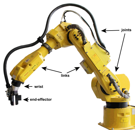
FIGURE 1.2 – Manipulator
