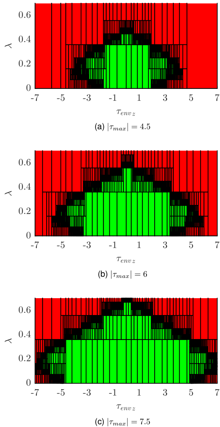
FIGURE 6.8 – SM subpaving analysis considering \tau_{envz} effects
