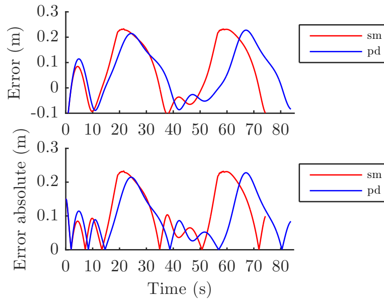
FIGURE 3.12 – Error comparison simulation.
