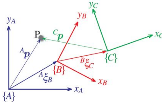
FIGURE 2.2 – Relative poses
