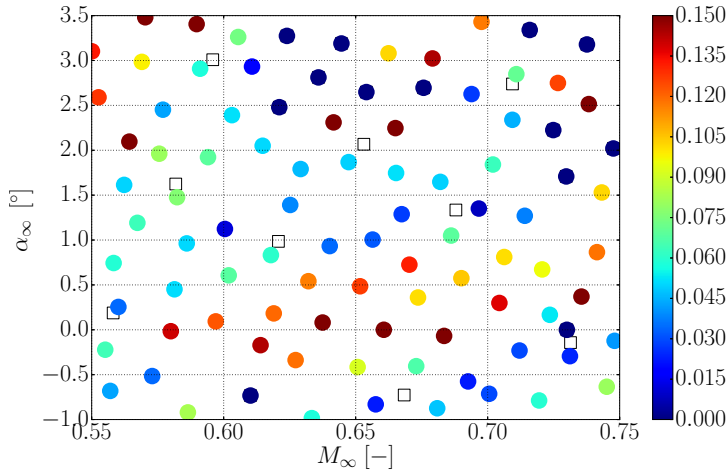
Figure 5.9: GPOD high-fidelity projection error \sqrt{\frac{\|\mathcal{IP}_g(\mathbf{s}) - \mathbf{I}\mathbf{s}\|^2}{\|\mathbf{I}\mathbf{s}\|^2}} after 12 iterations of PBI^+ enrichment.
