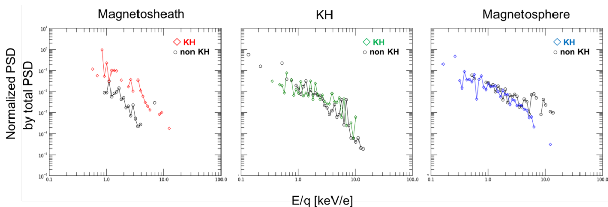
Figure 6.18 The average of the normalized \text{Na}^+ PSD behavior for 5 event sets. Similarly, the \text{Na}^+ PSD behavior in the magnetosphere shows differences in high energy region.
