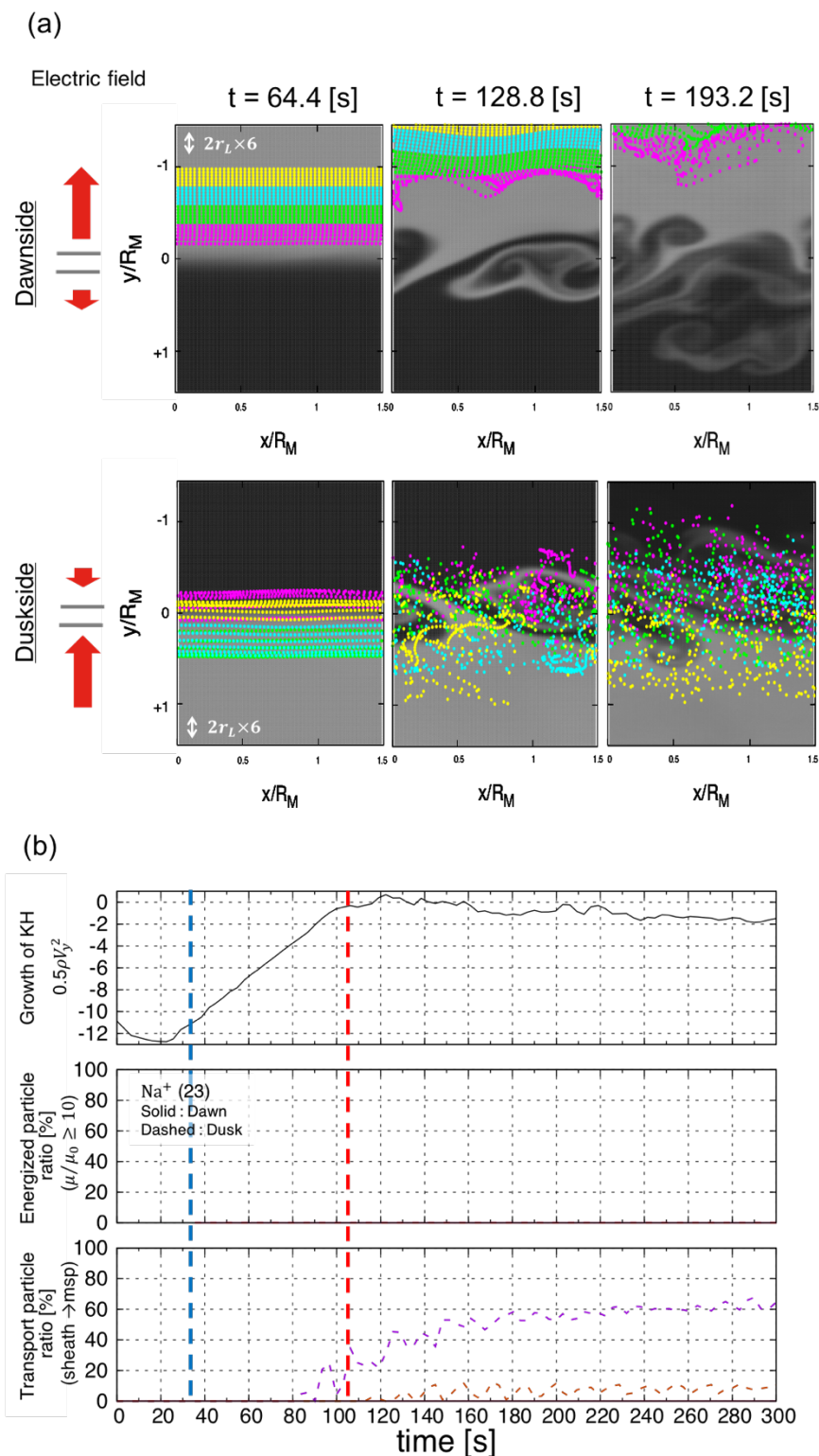
Figure 5.8 Energization and transport of sodium ions picked up in the magnetosheath. The format is the same as that of Figure 5.3 but transport is considered to be moving in the opposite direction.
