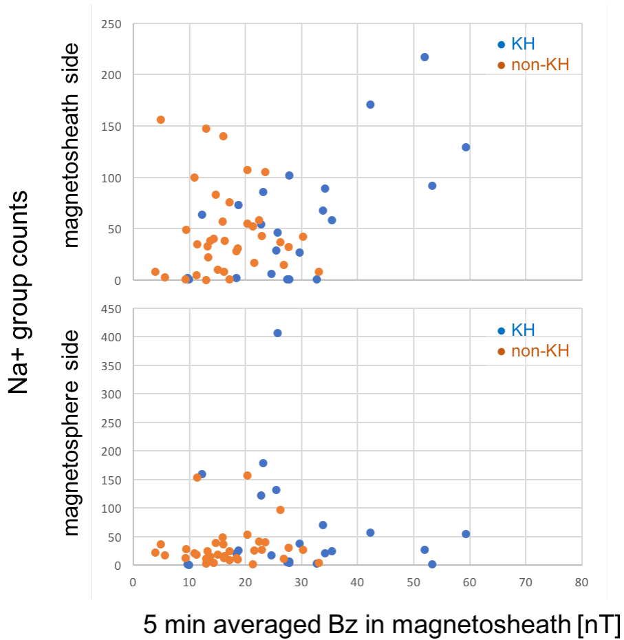
Figure 6.16 Count distribution of \text{Na}^+ -group ions as a function of 5 min averaged Bz in the magnetosheath. The format is the same as Figure 6.6.
