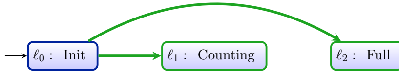
Figure 8.9: We add transitions (\ell_0, \ell_1) and (\ell_0, \ell_2) .
