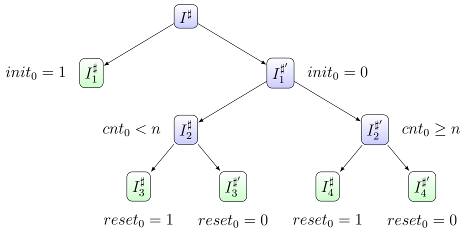
Figure 8.4: Partitioning of I^{\#} .
