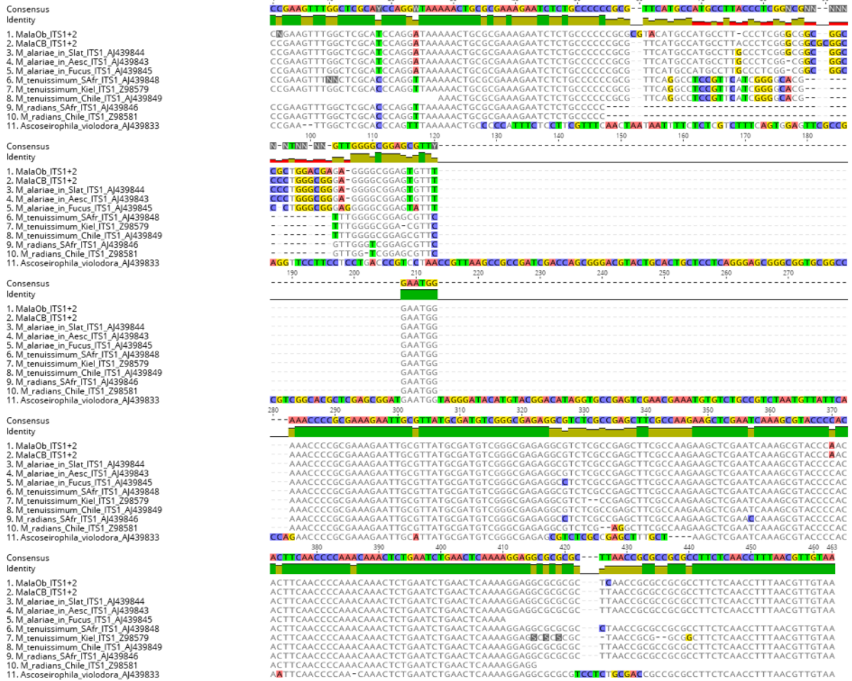
Supplemental Figure S1: Alignment of ITS1 used for M. alariae phylogeny reconstruction (Geneious view). Alignment was deposited at figshare.org ( https://doi.org/10.6084/m9.figshare.5962567.v1 ).
