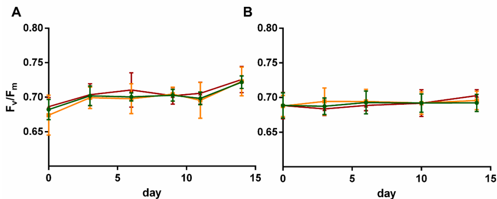
Figure 6: Maximum quantum yield of photosystem II ( F_v/F_m ) in A. S. latissima and B. L. digitata in control conditions (green), in presence of the non-endophytic M. tenuissimum (yellow) and the endophyte L. elsbetiae (red). The presented values are mean values with standard deviation (N=5).
