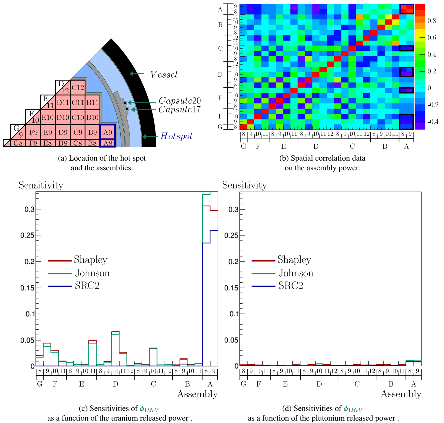
Figure V.17: Sensitivity analysis - Interest output: the fast flux \phi_{1MeV} at the hot spot, Perturbed variables: the power P_{ass} released from ^{235}\text{U} and ^{239}\text{Pu} .
