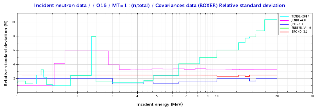
Figure 46: Relative standard deviation of the total cross section for the isotope ^{16}\text{O} Evaluation from JANIS Books
