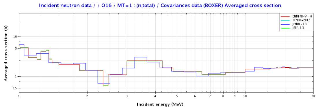
Figure 45: Multigroup cross section of the total cross section for the isotope ^{16}\text{O} Evaluation from JANIS Books
