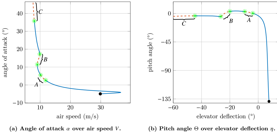
Fig. 7 Trim conditions of unthrottled longitudinal motion with the unstable regimes ( A , B , C ) of equilibria dashed (---); Hopf bifurcations marked by * ; starting point marked by \bullet .
