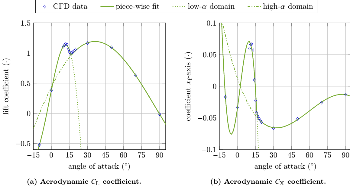
Fig. 2 Piecewise model of aerodynamic coefficients with polynomial segments [21].
