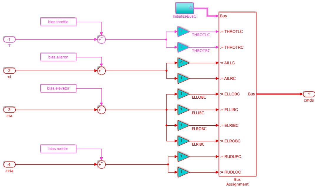
Figure C.9: Assignment of control inputs onto the aircraft actuator commands (throttle was chosen to be constantly zero).
