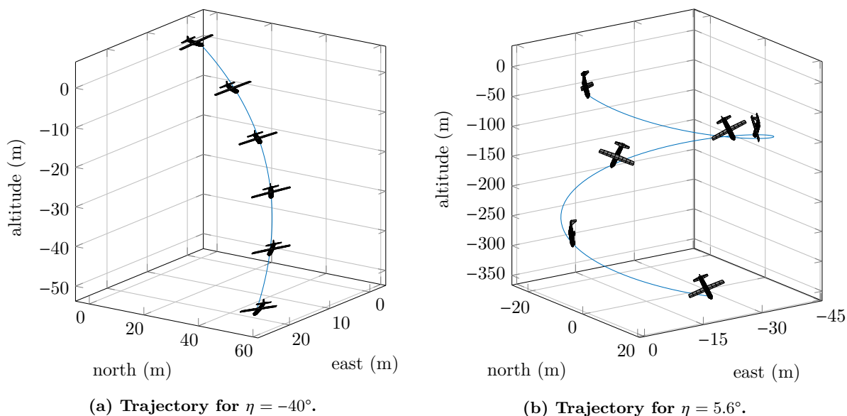
Fig. 20 Comparison of descent modes: (a) deep-stall descent; (b) steep descent.
