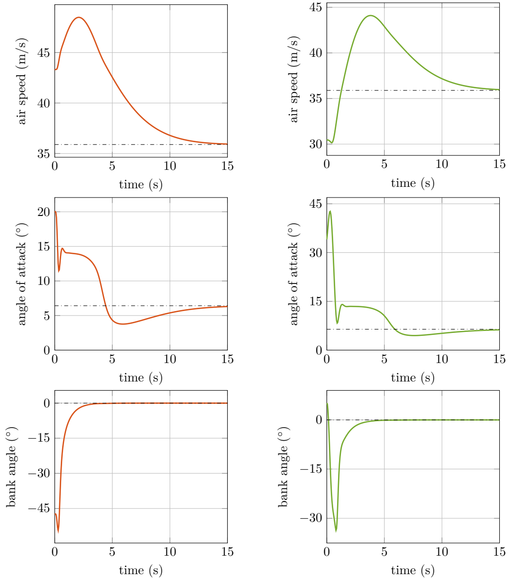
(a) Recovery from steep spiral.
