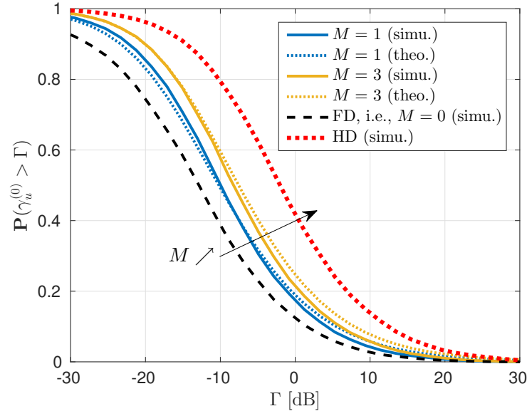
(a) v^* = 0 .
