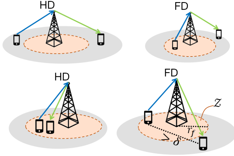
Fig. 3.1 Representation of a cellular network based on the proposed DS policy.
