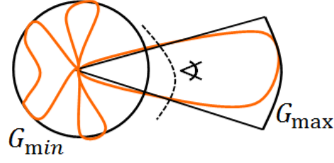
Fig. 2.7 Antenna gain pattern model used for MC deployments consisting of a main lobe of gain G_{\max} , that is considered for the intended links, and a secondary lobe of gain G_{\min} that affects interfering links. The orange line represents a more realistic antenna model and the bold-black line the approximation considered.
