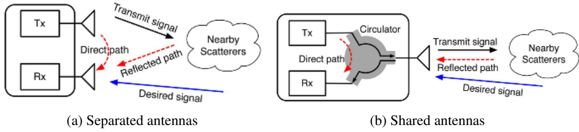
Fig. 1.5 Representation of the architecture of separated and shared antennas in a FD transceiver. (Figure taken from [20])
