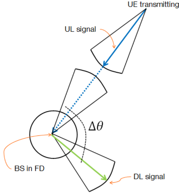
Fig. 4.1 Representation of the receiving and transmitting lobes of a beamforming-enabled FD BS.
