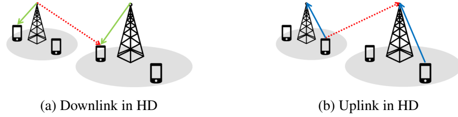
Fig. 1.2 Interference created in HD-based networks, where the red-dotted lines represent an interfering link. For the downlink in (a), the interference is generated by other DLs (transmitting BSs). For the uplink in (b), the interference is generated by other ULs (transmitting UEs).
