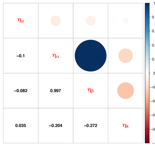
Figure 3.6 – Correlations between random effects.
