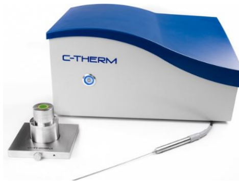
Figure 2.10 – TCi Thermal Conductivity Analyzer [184].
