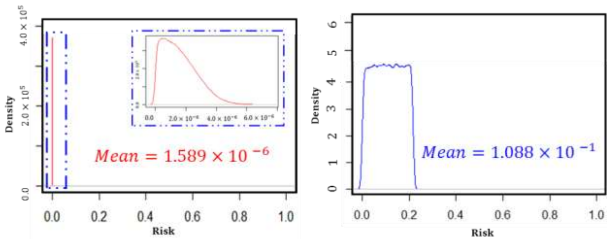
Figure 5 Updated risk estimates after considering the level of trustworthiness for external flooding (a) original risk estimate from the PRA, (b) Risk estimates after integrating the level of trustworthiness
