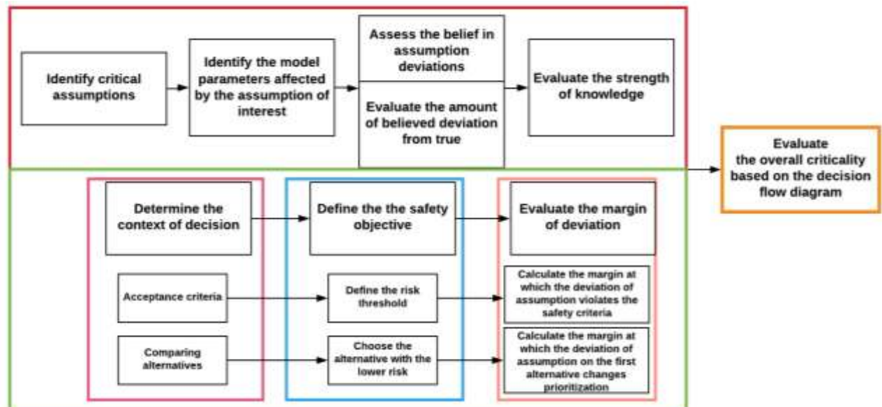
Figure 4.3 Procedure for applying the developed framework for assumption deviation criticality (risk) assessment.
