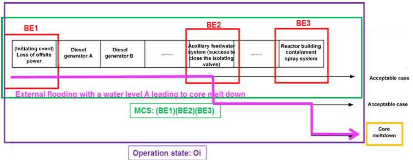
Figure 5 Illustration of a MCS in an individual reduced-order model
