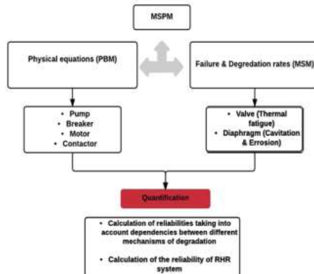
Figure 3 MSPM analysis: models of RHR components
