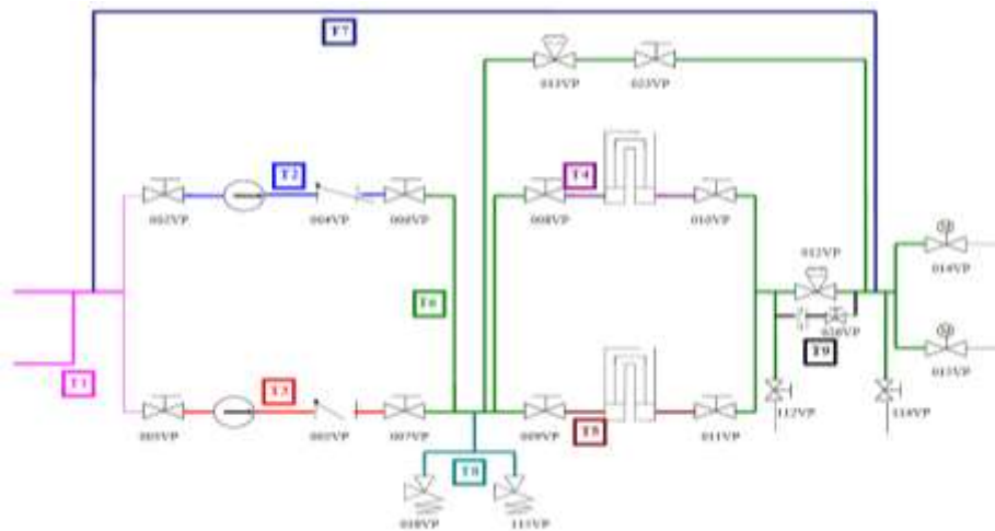
Figure 2.2 Schematic diagram of the RHR
