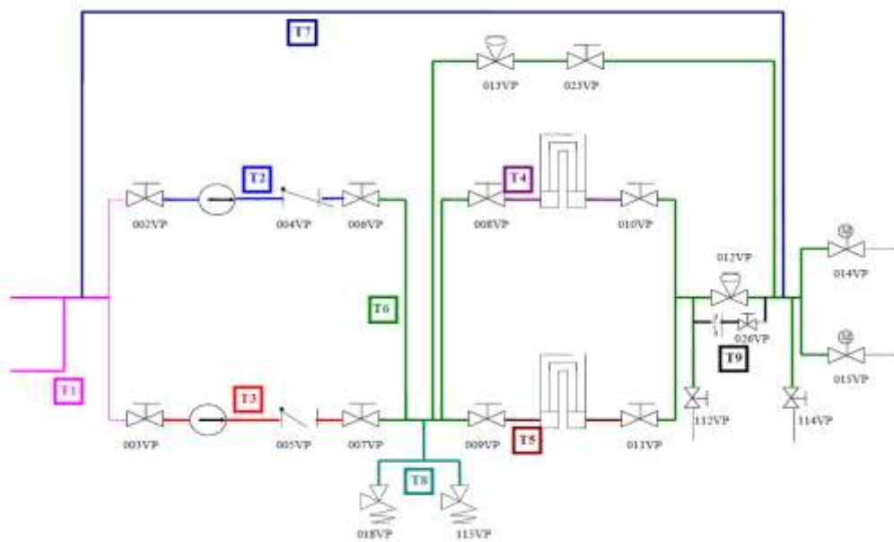
Figure 2 Schematic diagram of the RHR
