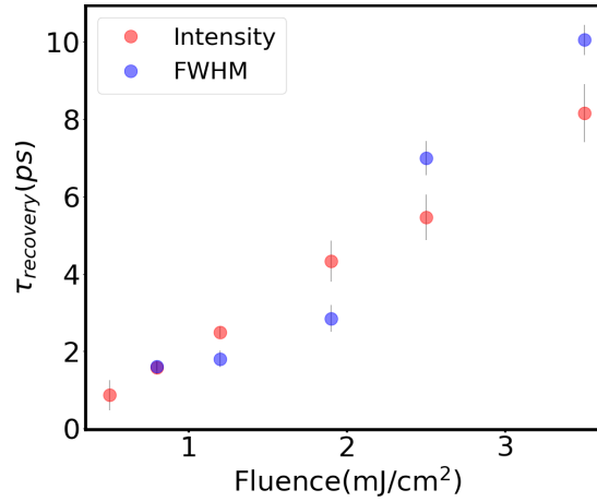
Figure 5.39: Recovery times of the CDW peak width and intensity as a function of the incident fluence. At F = 0.5 \text{ mJ/cm}^2 no changes of the peak width are observed.
