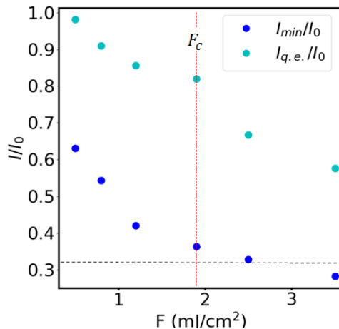
Figure 5.29: Intensity ratios at the minimum of the satellite intensity (dark blue) and at t > 40 ps (light blue). The dashed black line marks the background level and the red dashed line the critical fluence threshold.
