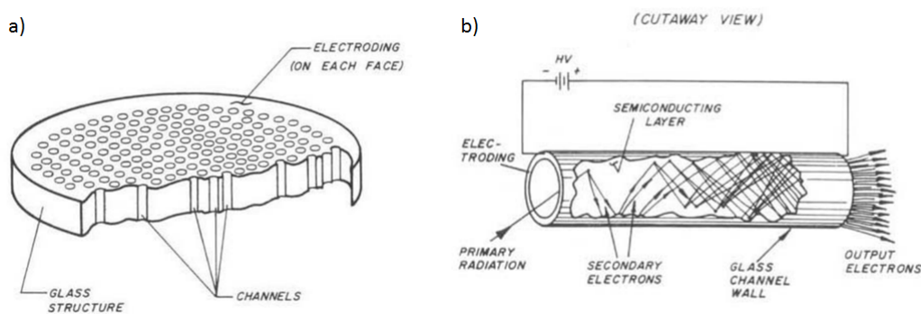
Figure 3.9: a) Schematic of a multiple channel plate showing the array of electron multipliers, b) schematic of a single electron multiplier tube. Images taken from [79].
