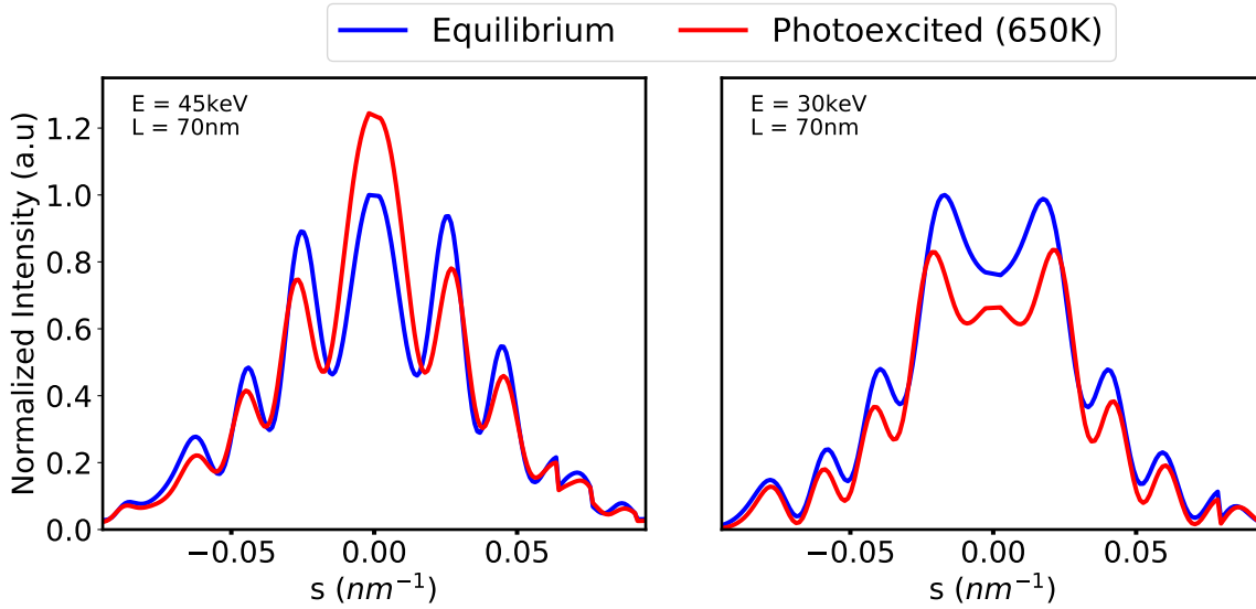
Figure 4.12: Modelled rocking curves via dynamical diffraction theory with the parameters from the experimental rocking curves considering a phenomenological background.
