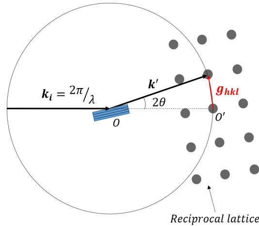
Figure 2.4: Schematic of the Ewald sphere with the radius given by the incident wavevector. The origin of real space is located at the point of incidence in the sample (blue rectangle) and O' denotes the center of reciprocal space.
