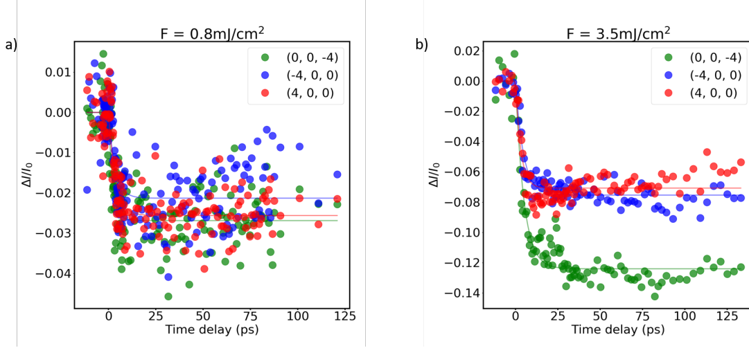
Figure 5.23: Comparison between the intensity changes of orthogonal Bragg peaks: ( \pm 400 ) and (00-4), with incident fluences of a) F = 0.8 \text{ mJ/cm}^2 and b) F = 3.5 \text{ mJ/cm}^2 , and initial temperature T_i = 155 \text{ K} .
