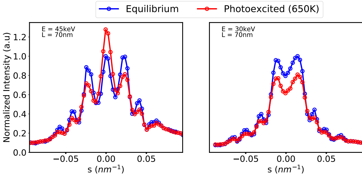
Figure 4.9: Left: Experimental rocking curves for the (2-20) peak taken with 45 keV electrons, at equilibrium T = 300 K (blue curve) and in the photoexcited state (red curve), taken at t = 150 ps delay with an incident fluence of F = 12 mJ/cm 2 . Right: Same but using 30 keV electrons as a probe. The rocking curves were normalized relative to the equilibrium case.
