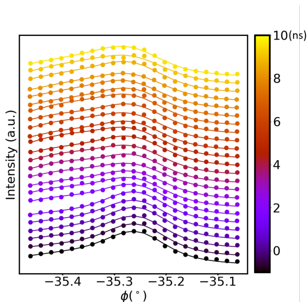
Figure 6.15: Rocking curves at different time delays at T=10\text{ K} and F=0.63\text{ mJ/cm}^2 .
