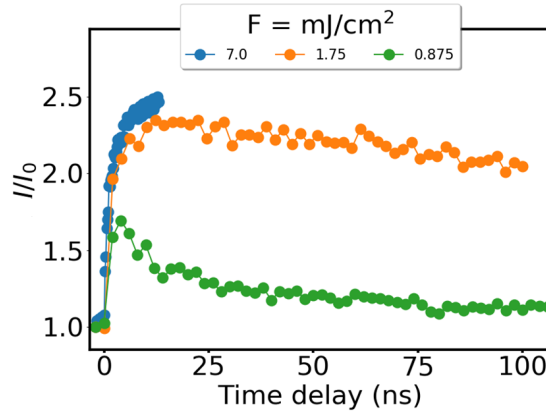
Figure 6.10: Relative intensity changes as a function of the time delay at constant \phi angle ( \phi = \phi_1 ) and at a sample temperature of T = 20 K.
