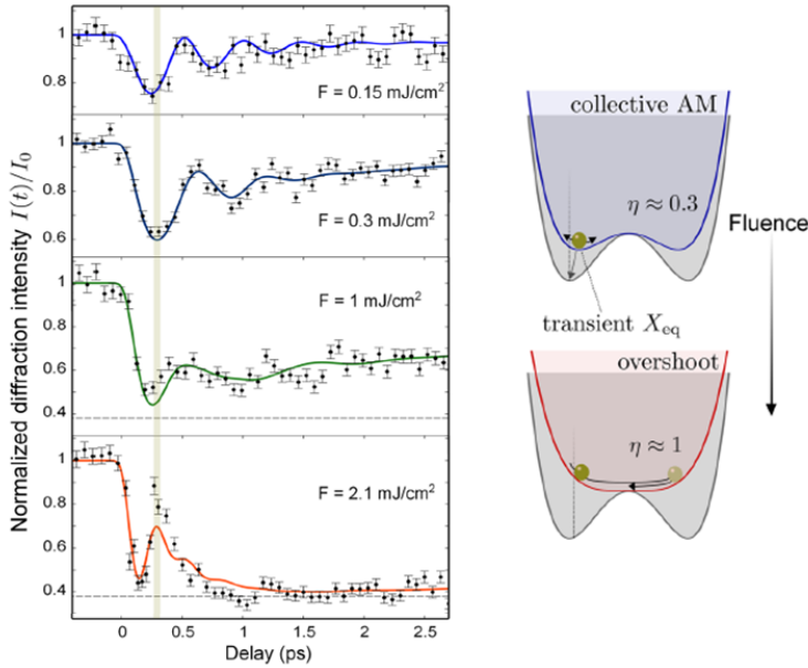
Figure 5.6: Temporal evolution of the satellite reflection intensity as a function of the incident fluence measured by Huber et al. in K_{0.3}MoO_3 . The solid lines represent fits within a displacive model which agrees to the dynamics resulting from equation 5.23. The schematic on the right side represents the potential energy of the Peierls barrier as a function of the excitation parameter \eta \propto F . Figure adapted from [22].
