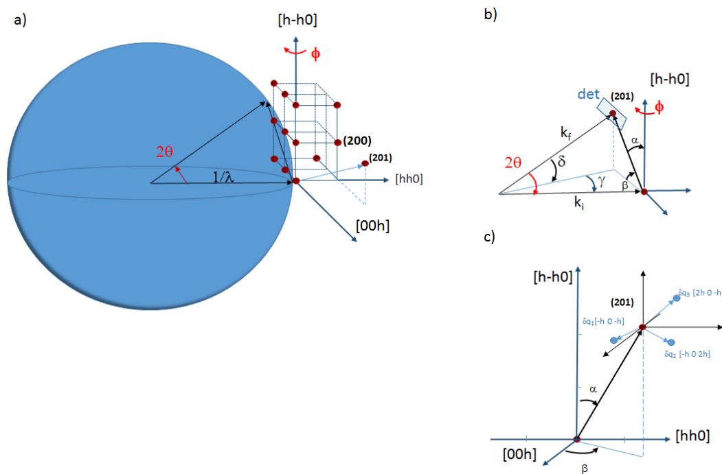
Figure E.1: a) Grazing incidence geometry with the \text{Nb}_3\text{Sn} sample orientation. The rotation around the \phi angle is used in order to intersect the (201) reflection on the Ewald sphere. b) Angular configuration with the section of the reciprocal lattice defined by the detector. c) The three possible variants observable in \text{Nb}_3\text{Sn} at low temperature.
