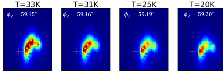
Figure 6.8: Detector images corresponding to the peak located at \phi_2 in the rocking curve. In this case the color map scale is the same for all images.
