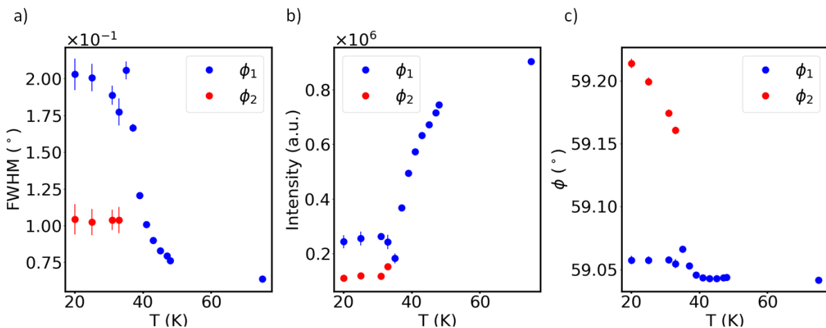
Figure 6.6: Fit parameters of the rocking scans at equilibrium temperatures: a) FWHM, b) maximum intensity (height parameter) and c) center.
