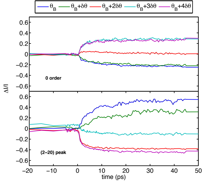
Figure 4.6: Photo-induced dynamics for various angles of incidence. The blue curve is obtained when the sample is exactly at the Bragg angle for the (2-20) peak; the other curves are obtained by tilting the sample by steps of \delta\theta = 0.26^\circ . The incident fluence is F = 12 \text{ mJ/m}^2 with an electron energy of 45 keV. Top: dynamics of the direct beam. Bottom: dynamics of the Bragg peak.
