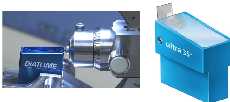
Figure 5.14: Left: Picture of an ultramicrotome with a 35^\circ diamond knife. Right: Sketch of the knife with the water container filled with the floating sections. Adapted figure from [144].
