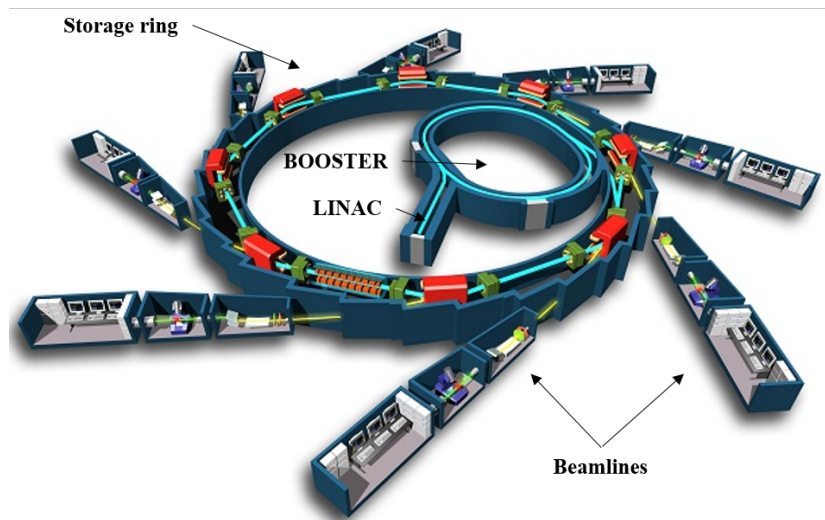
Figure 3.15: Schematic overview of the synchrotron main components.
