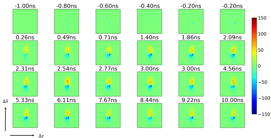
Figure 6.16: Detector images of the integrated rocking curve at different times delays. The sample temperature was T=10\text{ K} and the incident fluence F=0.63\text{ mJ/cm}^2 . Every image is a result after subtracting the image at negative time delays with t=-1\text{ ns} .
