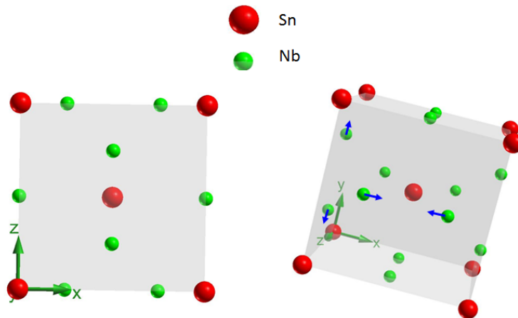
Figure 6.1: Unit cell of Nb 3 Sn in the cubic phase.
