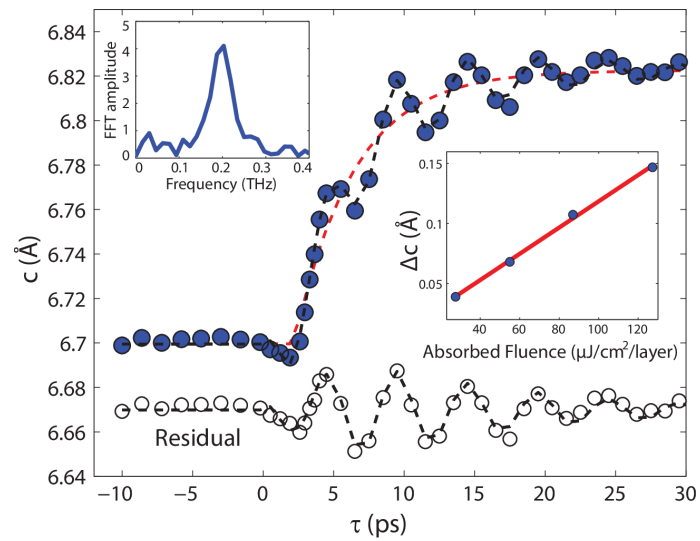
Figure 2.15: Coherent excitation of the thin film breathing mode in graphite. The c-axis lattice constant exhibits oscillatory dynamics in addition to simple expansion following photoexcitation. The measured frequency of 0.2 THz corresponds to a sample thickness of 10 nm. The overall c-axis expansion is linear in excitation fluence as shown in the inset. Image from [68].
