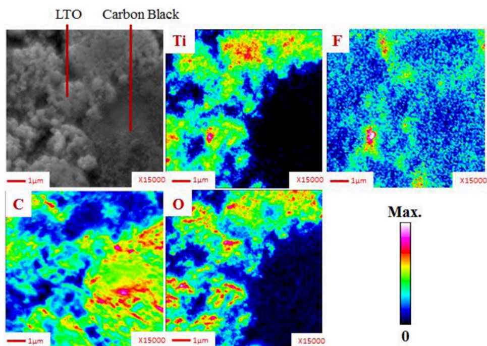
Figure 3. SEM image and SAM mappings of titanium Ti, fluorine F, carbon C and oxygen O of the LTO pristine electrode.
