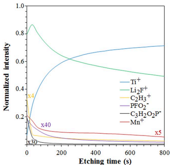
Figure 9. Normalized ToF-SIMS depth profiles over 800 s etching time of Ti^+ , Li_2F^+ , Mn^+ , C_2H_3^+ , POF_2^- and C_3H_2O_2P^- secondary ions detected in both polarities at the LTO electrode surface cycled facing NMC after hundred cycles at 4.6 V. For better clarity, Mn^+ , C_2H_3^+ , POF_2^- and C_3H_2O_2P^- signal intensities are multiplied \times 5 , \times 4 , \times 40 and \times 30 respectively.
