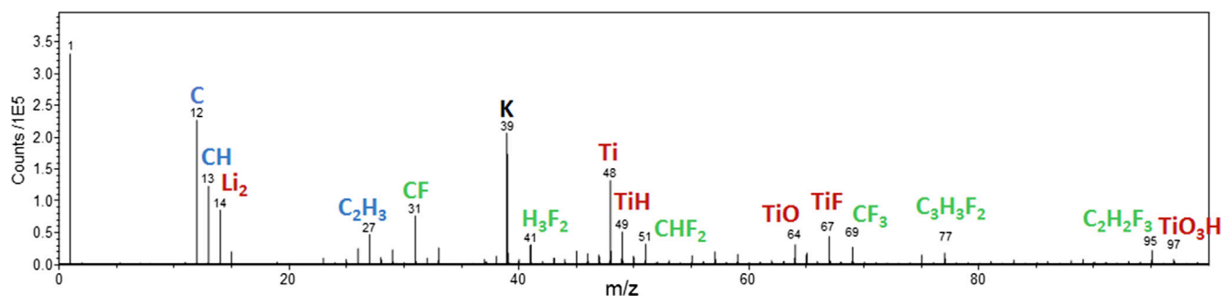
Fig. 1. ToF-SIMS mass spectrum of the pristine LTO electrode over 0–100 m/z range in the positive polarity (blue, red and green peaks are attributed to carbon black, LTO active material and PVdF respectively). (For interpretation of the references to colour in this figure legend, the reader is referred to the web version of this article.)
