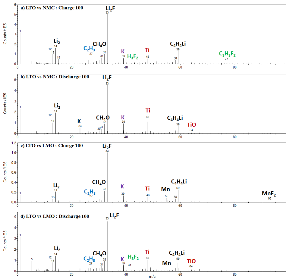
Figure S2. ToF-SIMS positive ion spectra of LTO electrodes cycled facing NMC after the hundredth charge a), after the hundredth discharge b), and cycled facing LMO after the hundredth charge c) and after the hundredth discharge d), over 0-100 m/z range.
