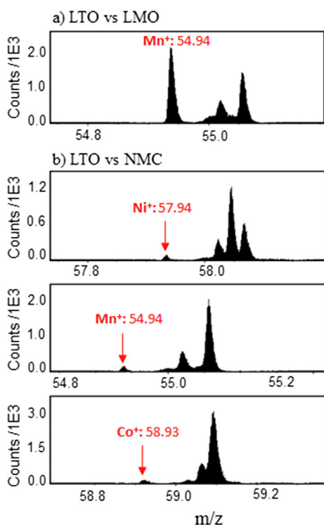
Fig. 3. ToF-SIMS positive ion spectra of LTO electrodes cycled facing LMO (a) and NMC (b) after the first cycle over \text{Mn}^+ , \text{Ni}^+ , and \text{Co}^+ specific m/z ranges.
