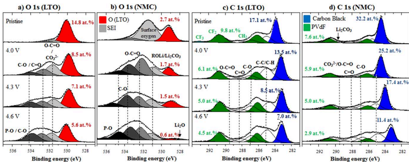
Figure 5. O 1s and C 1s XPS spectra of LTO (column a and c) and NMC (column b and d) pristine electrodes (first row), and LTO and NMC electrodes after 100 cycles operating the cathode at 4.0 V (second row), 4.3 V (third row) and 4.6 V (fourth row).
