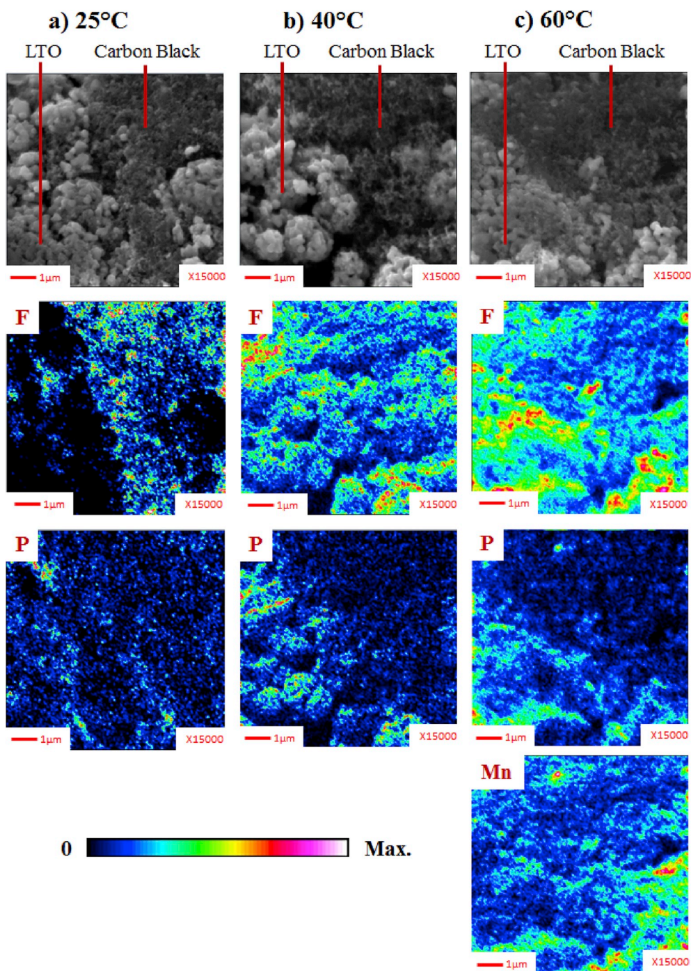
Fig. 6. SEM images and SAM chemical mappings of fluorine F, phosphorus P and manganese Mn on LTO electrodes surface at the end of the hundredth discharge for LTO/LMO cells cycled at 25 °C (a), 40 °C (b) and 60 °C (c). (in color). (For interpretation of the references to color in this figure legend, the reader is referred to the Web version of this article.)
