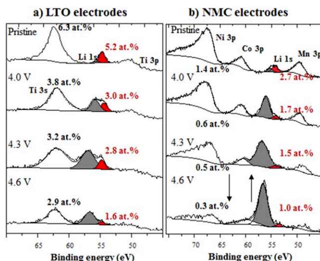
Figure 4. Ti 3s and Li 1s core peaks of the pristine LTO negative electrode (first row) and LTO electrodes after 100 cycles operating the NMC electrode at 4.0 V (second row), at 4.3 V (third row) and at 4.6 V (fourth row) (column a) and Ni 3p, Co 3p, Li 1s and Mn 3p core peaks of the pristine NMC positive electrode (first row) and NMC electrodes after 100 cycles at 4.0 V (second row), at 4.3 V (third row) and at 4.6 V (fourth row) (column b).
