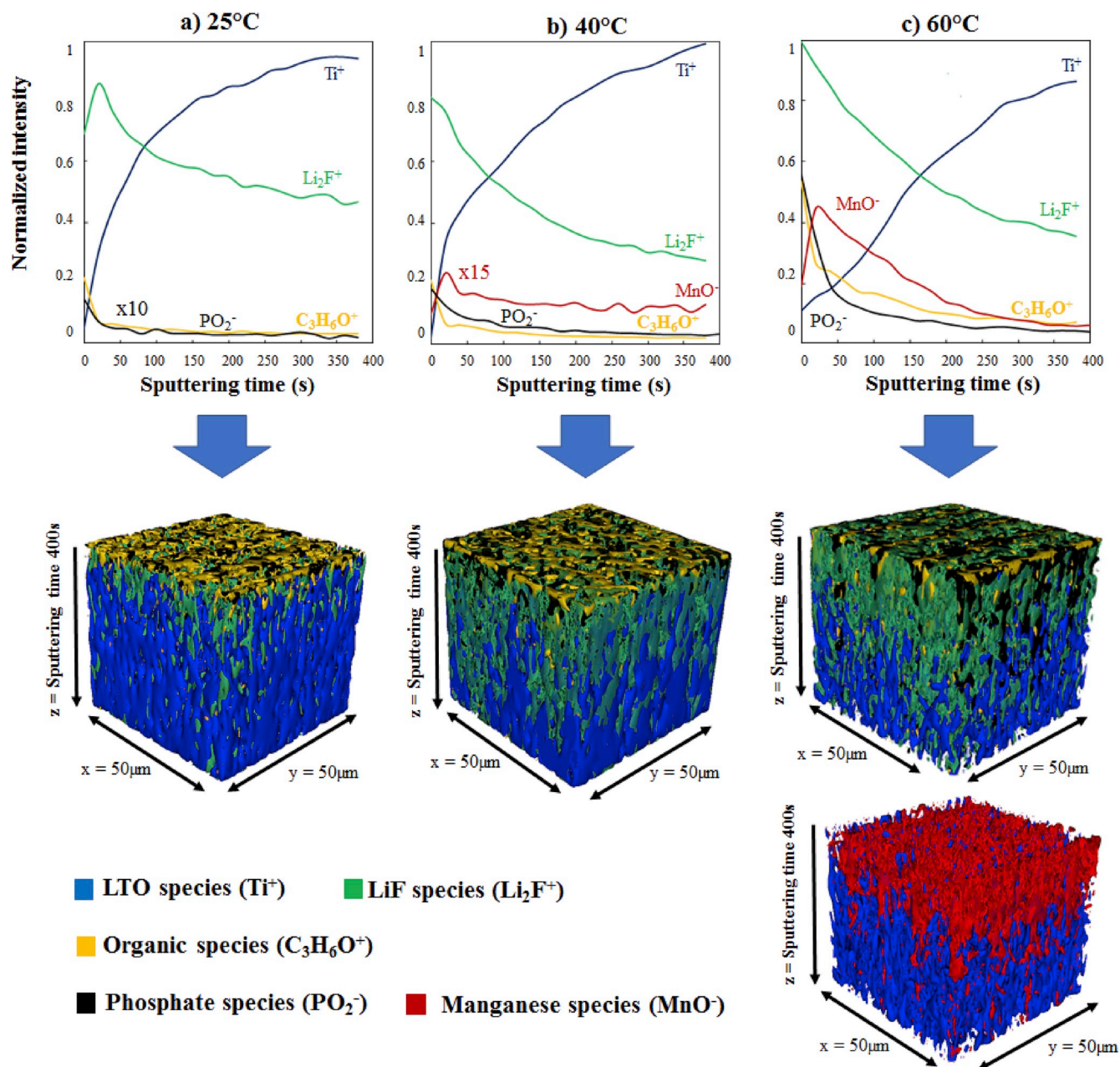
Fig. 8. Normalized ToF-SIMS depth profiles over 400 s of \text{Ti}^+ , \text{Li}_2\text{F}^+ , \text{C}_3\text{H}_6\text{O}^+ , \text{PO}_2^- and \text{MnO}^- secondary ions detected at the LTO electrode surface cycled facing LMO after the hundredth cycle at 25 °C (a), 40 °C (b) and 60 °C (c). 3D image reconstructions related to each depth profile, representing the in-depth spatial distribution of LTO (in blue), organic (in yellow), LiF (in green) and phosphates (in black) species. For better clarity, the 3D map representing manganese species (in red) with LTO (in blue) at 60 °C is presented separately. (in color). (For interpretation of the references to color in this figure legend, the reader is referred to the Web version of this article.)
