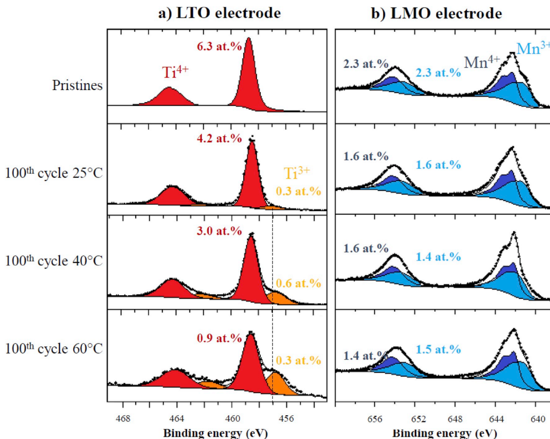
Fig. 2. (a) Ti 2p XPS spectra of the pristine LTO negative electrode (first line) and LTO electrodes after 100 cycles at 25 °C (second line), 40 °C (third line) and 60 °C (fourth line) and (b) Mn 2p core peaks of the pristine LMO positive electrode (first line) and LMO electrodes after 100 cycles at 25 °C (second line), 40 °C (third line) and 60 °C (fourth line). (in color). (For interpretation of the references to color in this figure legend, the reader is referred to the Web version of this article.)
