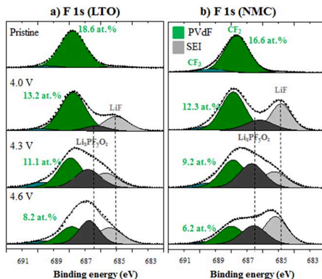
Figure 6. F 1s XPS spectra of LTO (column a) and NMC (column b) pristine electrodes (first row), and of LTO and NMC electrodes after 100 cycles operating the cathode at 4.0 V (second row), at 4.3 V (third row) and at 4.6 V (fourth row).
