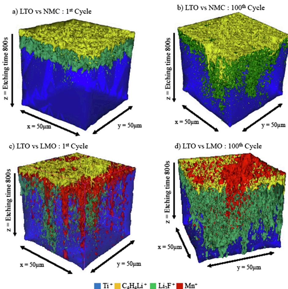
Fig. 5. 3D images reconstruction from ToF-SIMS depth profile experiments showing the spatial distributions of \text{Ti}^+ , \text{C}_4\text{H}_4\text{Li}^+ , \text{Li}_2\text{F}^+ and \text{Mn}^+ secondary ions over 50 \mu\text{m} (x axis) by 50 \mu\text{m} (y axis) raster size and 800 s etching time (z axis), at the LTO electrodes surfaces at the end of the first and the hundredth cycles versus NMC electrode (a) and (b) and versus LMO electrode (c) and (d).
