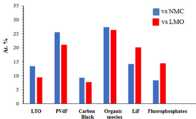
Figure 10. Histogram comparing the amount of species detected at the surface of LTO electrodes at the end of the 100 th lithiation cycle facing NMC (blue) and cycled facing LMO (red).
