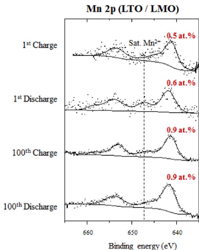
Figure 8. Mn 2p XPS spectra of the cycled LTO negative electrodes versus LMO after the first charge, after the first discharge, after the hundredth charge and after the hundredth discharge.
