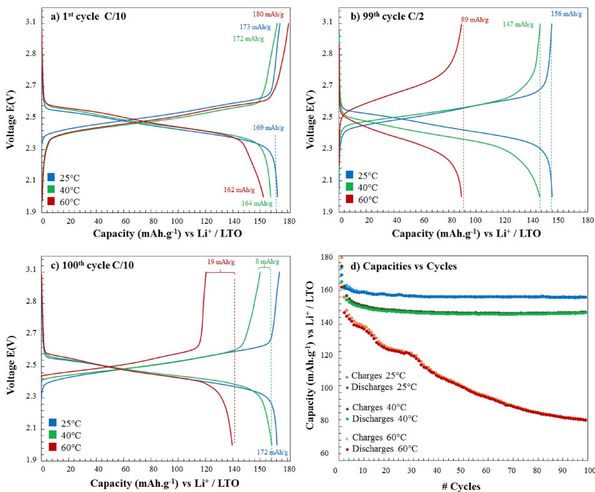
Fig. 1. Galvanostatic charge/discharge voltage profiles of LTO/LMO cells at 25 °C (in blue), 40 °C (in green) and 60 °C (in red) (a) for the 1 st cycle at C/10, (b) for the 99 th cycle at C/2 and (c) for the 100 th cycle at C/10; Charge and discharge capacities of LMO/LTO systems cycled at 25 °C (in blue), 40 °C (in green) and 60 °C (in red) for the first 100 cycles d). (in color). (For interpretation of the references to color in this figure legend, the reader is referred to the Web version of this article.)
