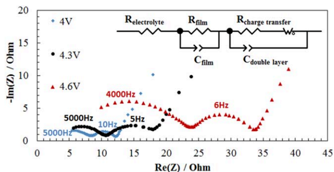
Figure 3. Experimental EIS results of NMC/LTO full cells at 0% SOC and at 25 °C after 100 cycles operating the positive electrode at 4.0 V (blue), 4.3 V (black) and 4.6 V (red) vs Li^0/Li^+ .
