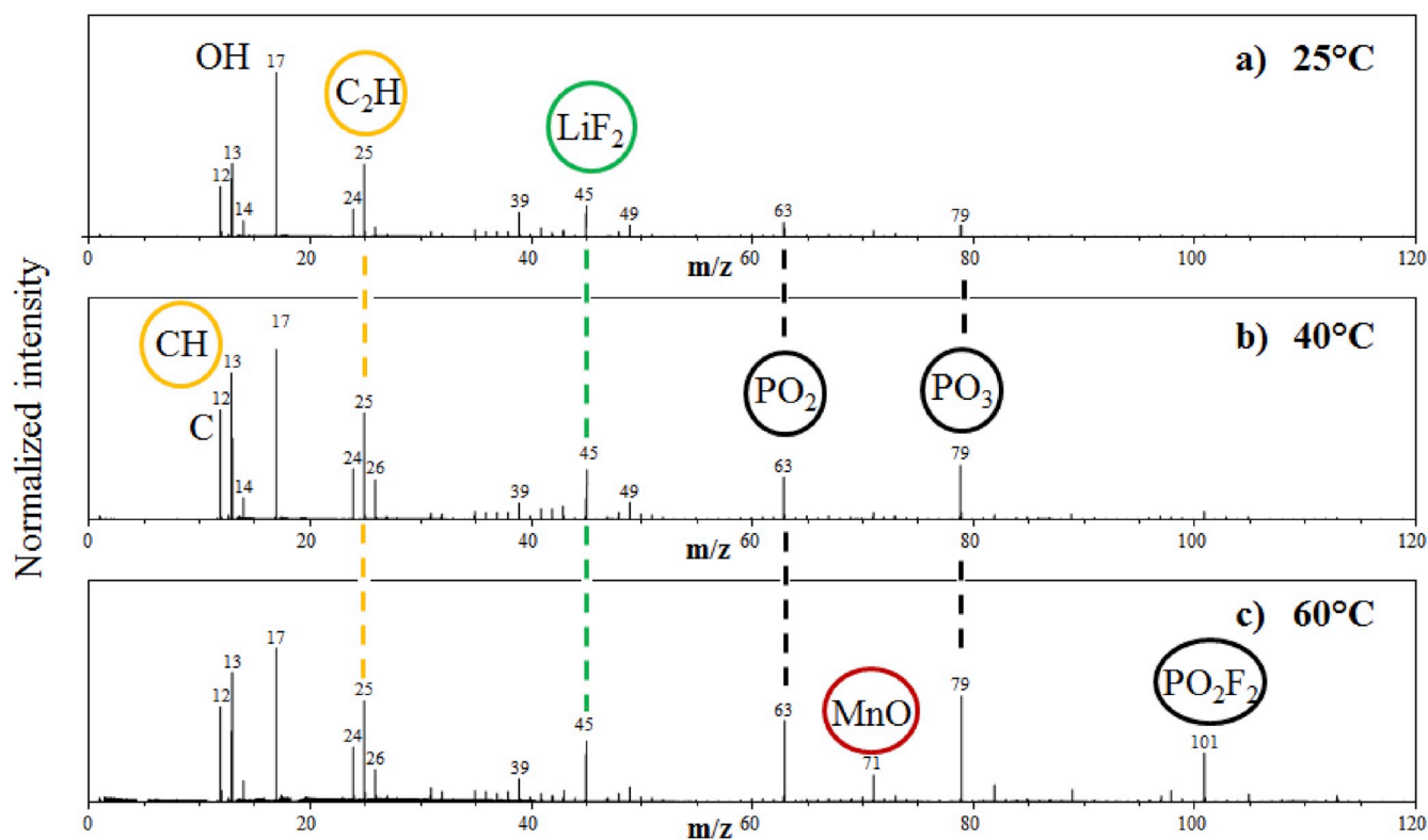
Fig. 7. ToF-SIMS negative ion spectra over 0–120 m/z range for LTO electrodes cycled at 25 °C (a), 40 °C (b), and 60 °C (c) at the end of the hundredth cycle. (in color). (For interpretation of the references to color in this figure legend, the reader is referred to the Web version of this article.)
