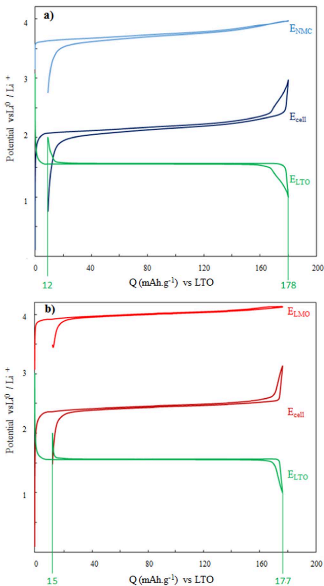
Figure 1. Galvanostatic profiles of a) LTO/NMC and b) LTO/LMO cells for the first cycle at 60^\circ\text{C} , displaying the potentials of LTO electrodes vs \text{Li}^0/\text{Li}^+ ( E_{\text{LTO}} ), the NMC electrode vs \text{Li}^0/\text{Li}^+ ( E_{\text{NMC}} ), the LMO electrode vs \text{Li}^0/\text{Li}^+ ( E_{\text{LMO}} ) and the cell voltages ( E_{\text{CELL}} ).
