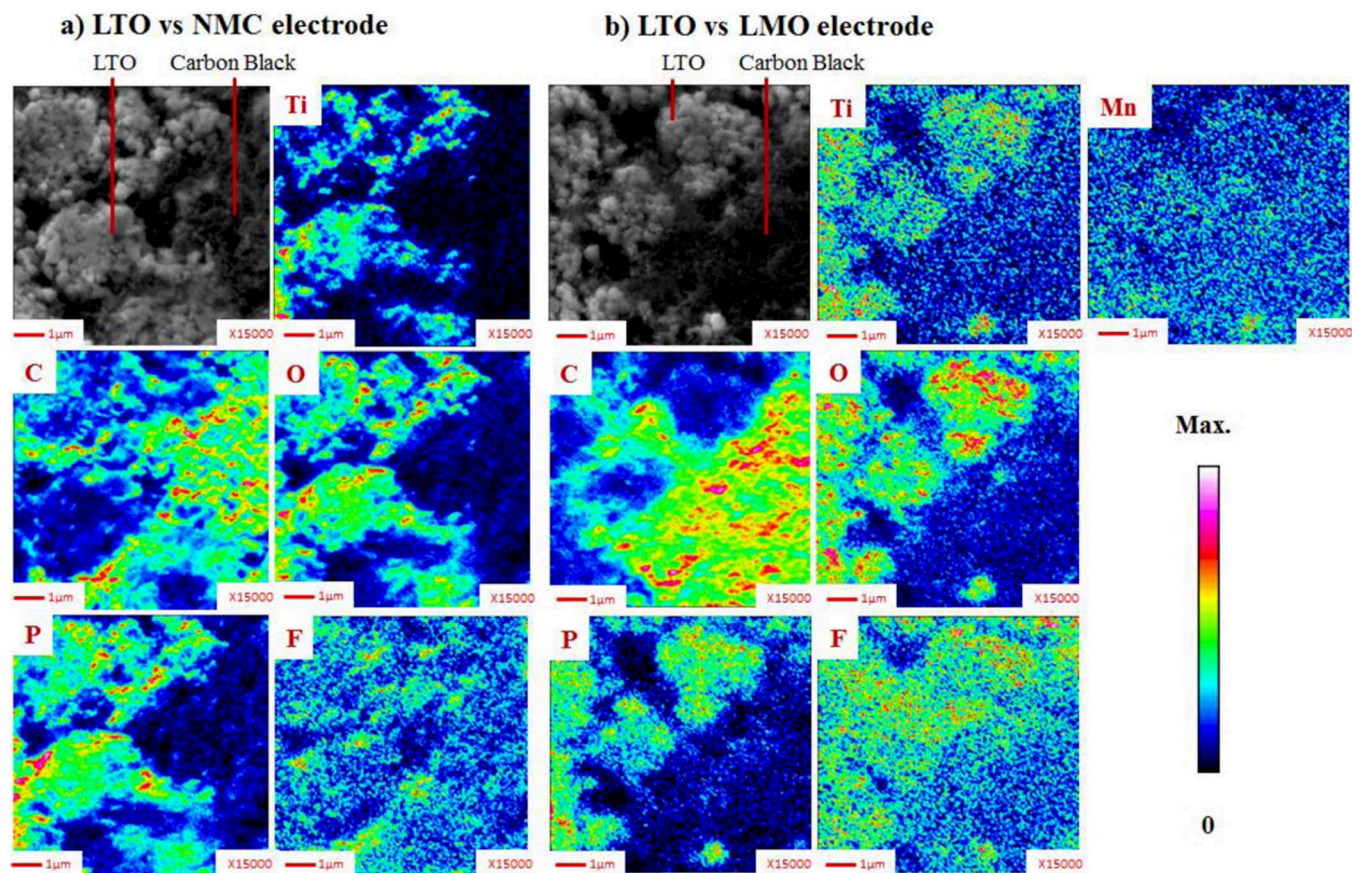
Figure 9. SEM images and SAM chemical mappings of carbon C, phosphorus P, titanium Ti, oxygen O, fluorine F, and manganese Mn on LTO electrodes surface at the end of the hundredth charge for LTO/NMC a) and LTO/LMO b) cells.
