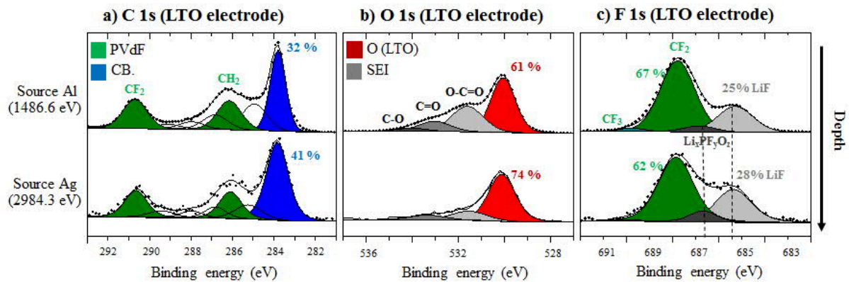
Figure S4. C 1s a), O 1s b) and F 1s c) XPS spectra of cycled LTO negative electrodes at the end of the first discharge in front of NMC electrode obtained with Al K \alpha radiation ( h\nu = 1486.6 eV) (first line) and Ag L \alpha radiation ( h\nu = 2984.3 eV) (second line).
