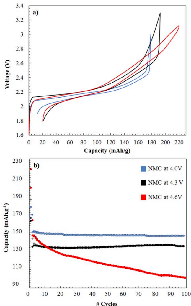
Figure 1. (a) Galvanostatic profiles of NMC/LTO cells at the first cycle at 60 °C, operating the NMC electrode at 4.0 V (blue curve), 4.3 V (black curve) and 4.6 V (red curve) vs \text{Li}^0/\text{Li}^+ . (b) Charge/discharge capacities vs \text{Li}^+/\text{LTO} of the NMC/LTO cells operating the NMC electrode at 4.0 V (blue) and 4.3 V (black) vs \text{Li}^0/\text{Li}^+ ; and charge/discharge capacities vs \text{Li}^0/\text{NMC} of the NMC/LTO cells operating the NMC electrode at 4.6 V (red) vs \text{Li}^0/\text{Li}^+ for the first 100 galvanostatic cycles.
