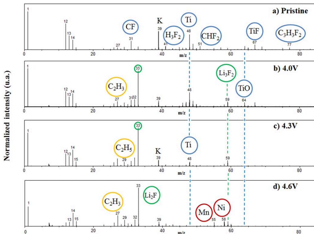
Figure 8. ToF-SIMS positive ion spectra over 0–90 m/z range for LTO electrodes before cycling (a) and after 100 cycles operating the NMC electrode at 4.0 V (b), 4.3 V (c), and 4.6 V (d).
