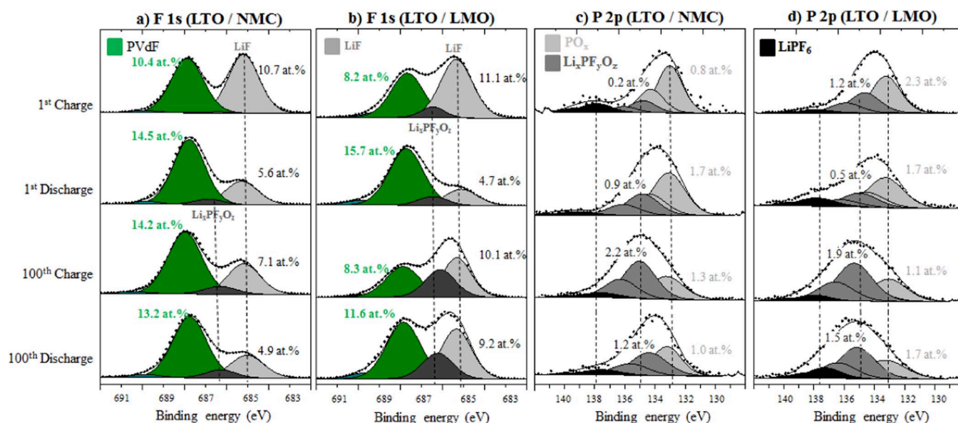
Figure 7. F 1s and P 2p XPS spectra of the cycled LTO negative electrodes after the first charge, after the first discharge, after the hundredth charge and after the hundredth discharge for a) and c) LTO/NMC as well as for b) and d) LTO/LMO cells.
