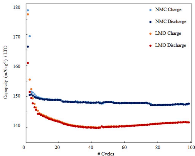
Figure 2. Charge and discharge capacities of the NMC/LTO (blue curves) and LMO/LTO systems (red curves) for the first 100 galvanostatic cycles.
