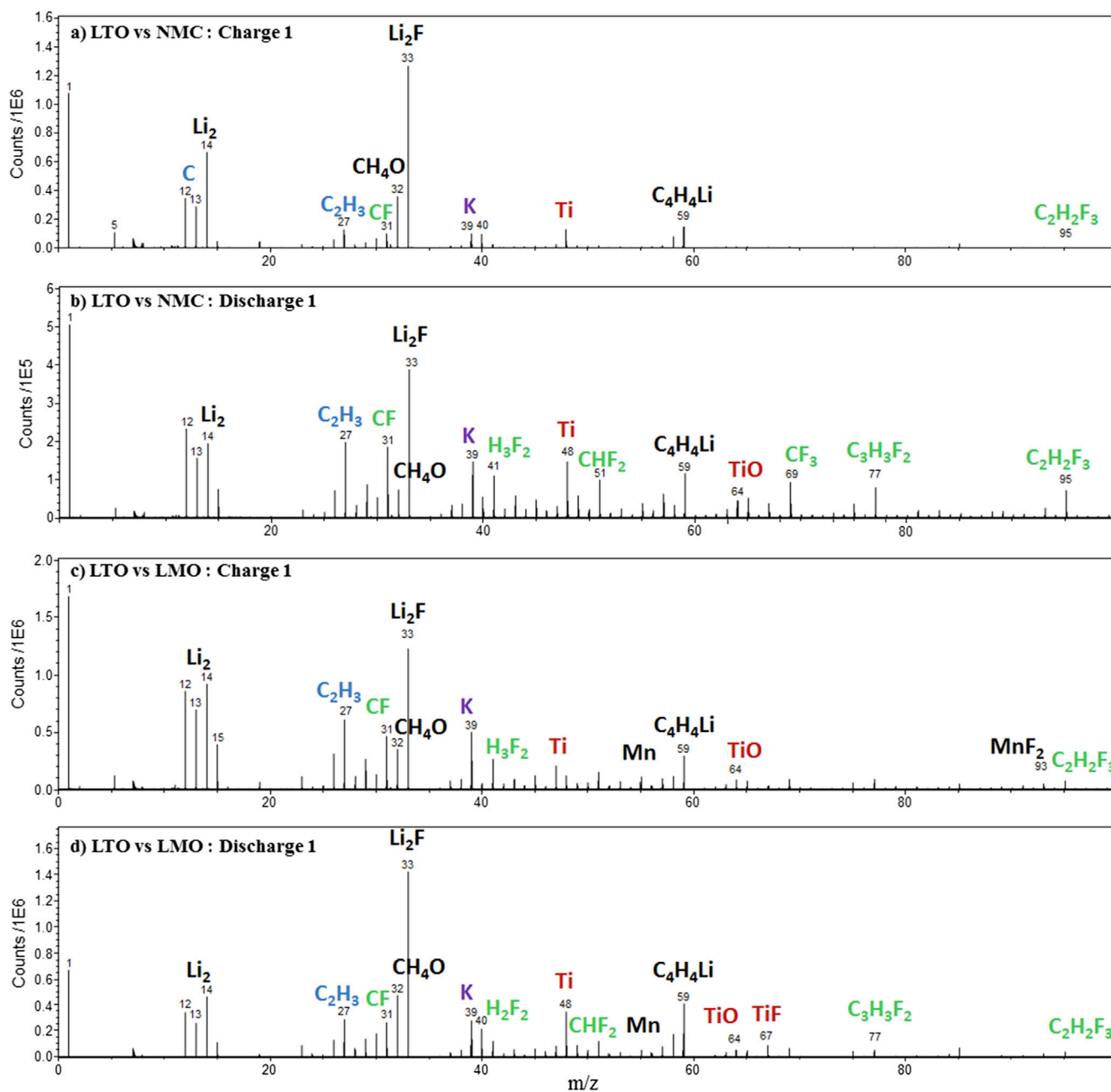
Fig. 2. ToF-SIMS positive ion spectra over 0–100 m/z range for LTO electrodes cycled facing NMC after the first charge (a), the first discharge (b), and for LTO electrodes cycled facing LMO after the first charge (c), and the first discharge (d).
