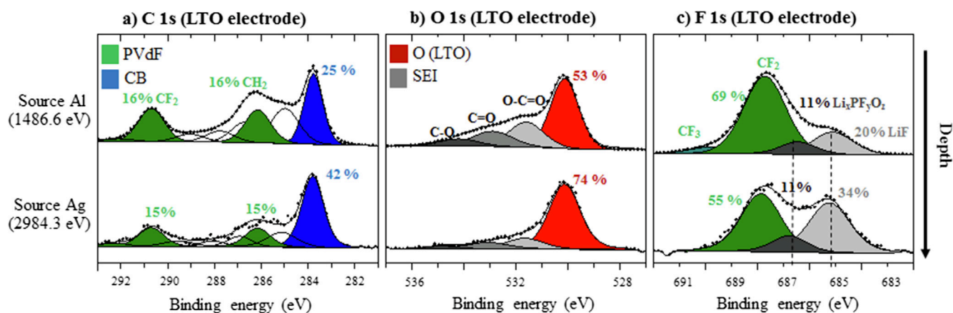
Fig. 6. C 1s (a), O 1s (b) and F 1s (c) XPS spectra of cycled LTO negative electrodes at the end of the first cycle in front of LMO electrode obtained with Al K \alpha radiation ( h\nu = 1486.6 eV) (first line) and Ag L \alpha radiation ( h\nu = 2984.3 eV) (second line). The relative percentages of main components are reported in the figure.
