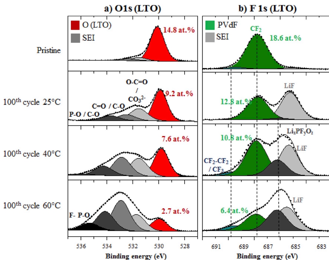
Fig. 3. (a) O 1s and (b) F 1s XPS spectra of the pristine LTO negative electrode (first line) and LTO electrodes after 100 cycles at 25 °C (second line), 40 °C (third line) and 60 °C (fourth line) versus LMO electrodes. (in color). (For interpretation of the references to color in this figure legend, the reader is referred to the Web version of this article.)
