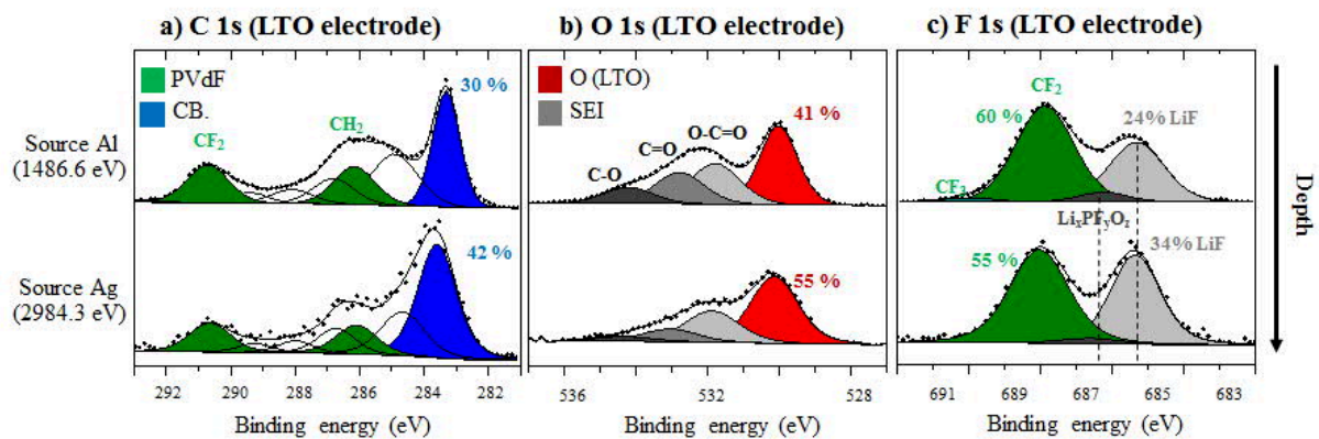
Figure S5. C 1s a), O 1s b) and F 1s c) XPS spectra of the cycled LTO negative electrodes at the end of the hundredth discharge in front of NMC electrode obtained with a monochromatized Al K \alpha radiation ( h\nu = 1486.6 eV) (first line) and Ag L \alpha radiation ( h\nu = 2984.3 eV) (second line). (in color)
