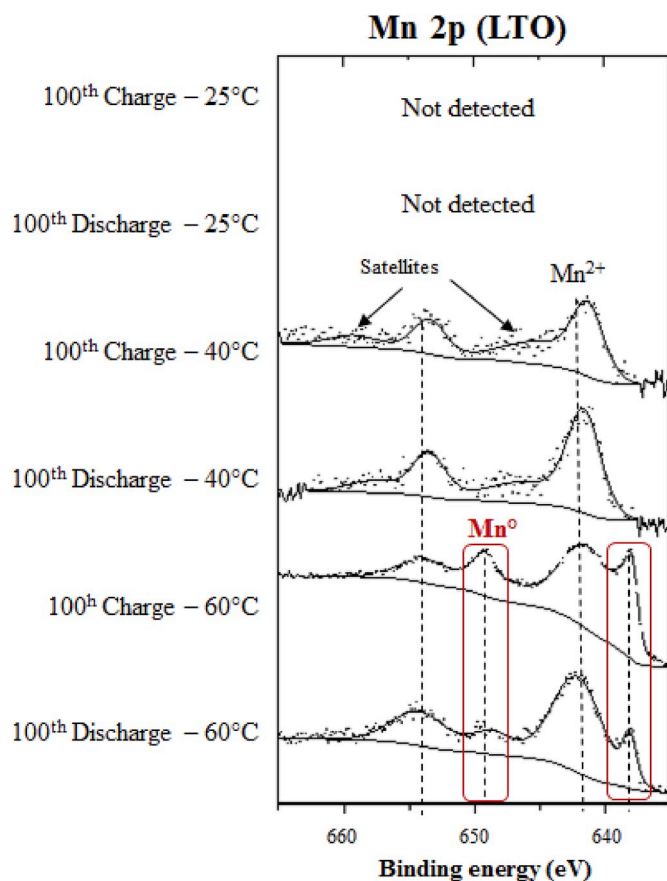
Fig. 5. Mn 2p XPS spectra of cycled LTO electrodes versus LMO after the 100 th charge and after the 100 th discharge at 25 °C, 40 °C and 60 °C. (in color). (For interpretation of the references to color in this figure legend, the reader is referred to the Web version of this article.)
