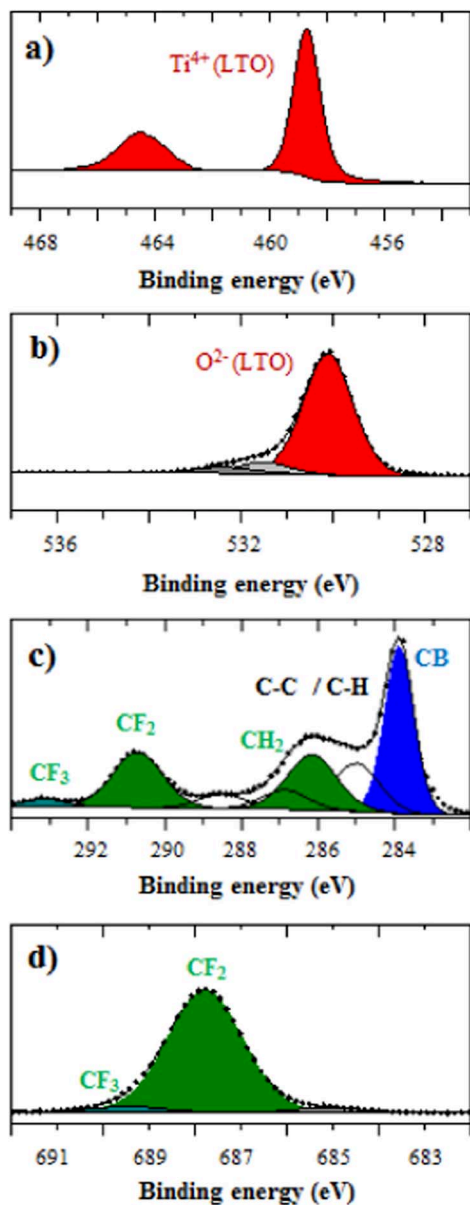
Figure 4. a) Ti 2p, b) O 1s, c) C 1s and d) F 1s XPS spectra of the LTO pristine electrode. CB = carbon black.
