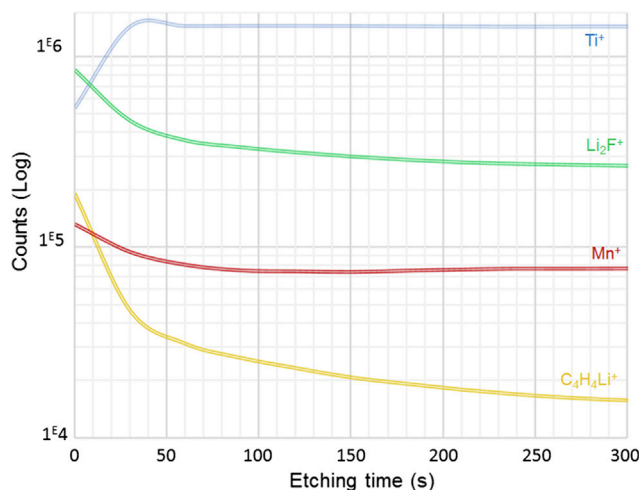
Fig. 4. ToF-SIMS depth profiles of \text{Ti}^+ (blue), \text{Li}_2\text{F}^+ (green), \text{Mn}^+ (red) and \text{C}_4\text{H}_4\text{Li}^+ (yellow) secondary ions over 300 s etching time for the LTO/LMO system after the first cycle. (For interpretation of the references to colour in this figure legend, the reader is referred to the web version of this article.)
