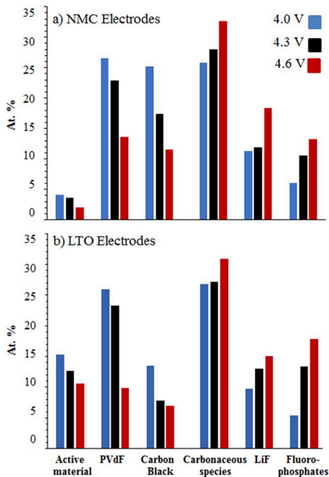
Figure 7. Histogram comparing the amount of species detected at the surface of LTO and NMC electrodes at the end of the 100th cycles operating the cathode at 4.0 V (blue), 4.3 V (black) and 4.6 V (red). Among carbonaceous species, oxalates, PEO, alkyl and lithium carbonates coming from solvent degradation are considered.
