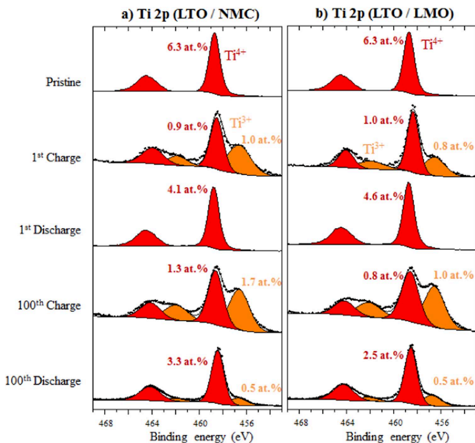
Figure 5. Ti 2p XPS spectra of the LTO negative pristine electrode (first line), the cycled LTO negative electrodes after the first charge, after the first discharge, after the hundredth charge and after the hundredth discharge for a) LTO/NMC and b) LTO/LMO cells.
