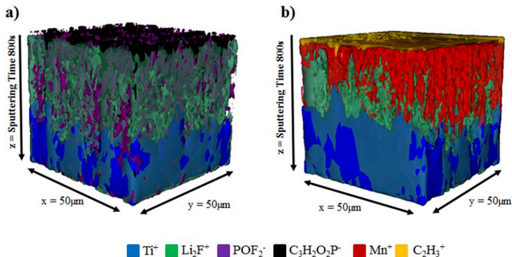
Figure 10. 3D images reconstructed from ToF-SIMS depth profile experiments showing the in-depth spatial distribution of \text{Ti}^+ (in blue), \text{Li}_2\text{F}^+ (in green), \text{POF}_2^- (in purple) and \text{C}_3\text{H}_2\text{O}_2\text{P}^- (in black) a) and of \text{Mn}^+ (in red), \text{C}_2\text{H}_3^+ (in yellow) and \text{Li}_2\text{F}^+ (in green) b) at the surface of LTO electrodes cycled facing NMC at 4.6 V (vs \text{Li}^0/\text{Li}^+ ) after the hundredth cycle.
