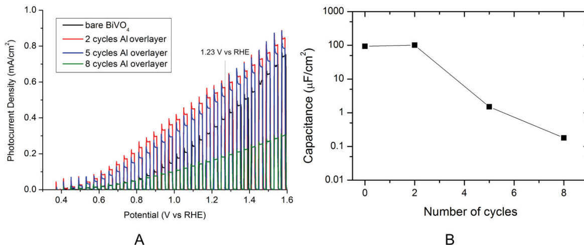
Figure S2. (A) Linear sweep voltammograms of bare BiVO 4 and Al-modified BiVO 4 (electrolyte: 0.1M Na-Pi pH 7, scan rate: 10 mV/s) and (B) Surface capacitance measurements at various cycles
