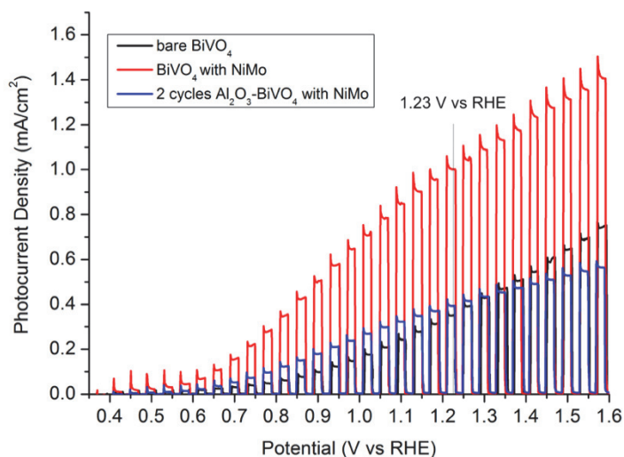
Figure S3. Linear sweep voltammogram for bare \text{BiVO}_4 , \text{BiVO}_4 with NiMo and 2 cycles Al- \text{BiVO}_4 with NiMo (electrolyte: 0.1 \text{ M Na-Pi} pH 7, scan rate: 10 \text{ mV/s} )
