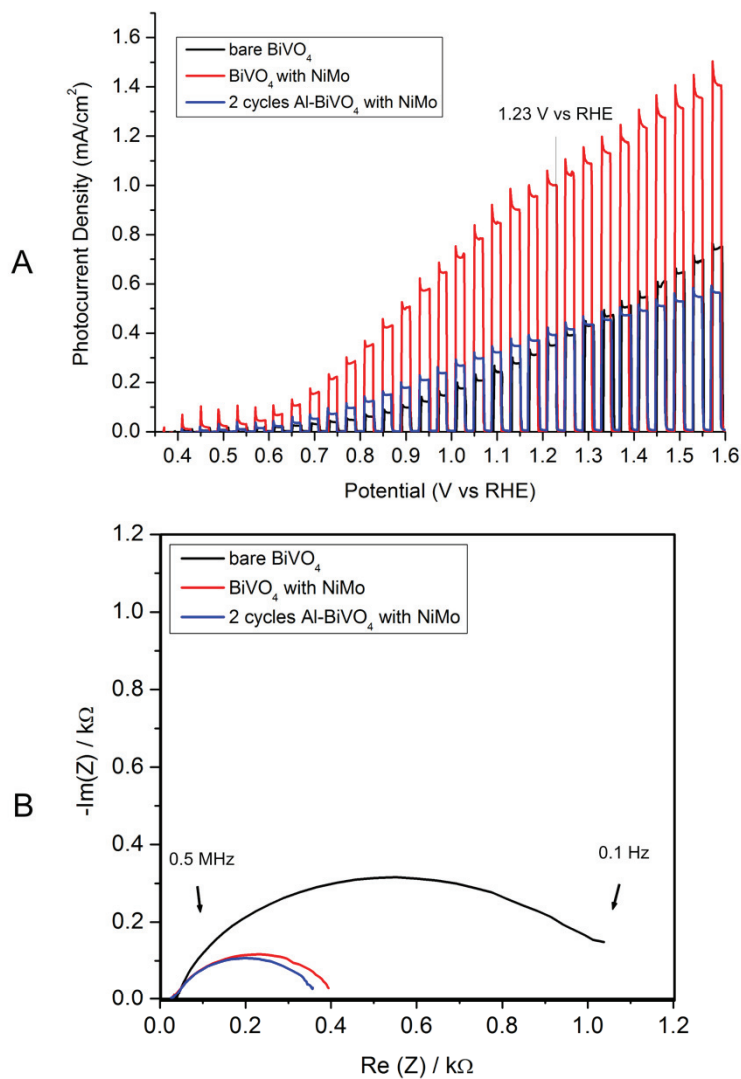
Figure 27. (A) LSV (electrolyte: 0.1 M Na-Pi pH 7, scan rate: 10 mV/s) and (B) Nyquist plots for bare BiVO 4 , BiVO 4 with NiMo and 2 cycles Al-BiVO 4 with NiMo
