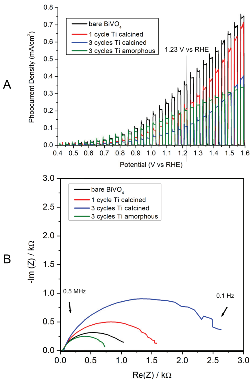
Figure 26. (A) LSV (electrolyte: 0.1 M Na-Pi pH 7, scan rate: 10 mV/s) and (B) Nyquist impedance plots for bare and Ti-modified BiVO 4
