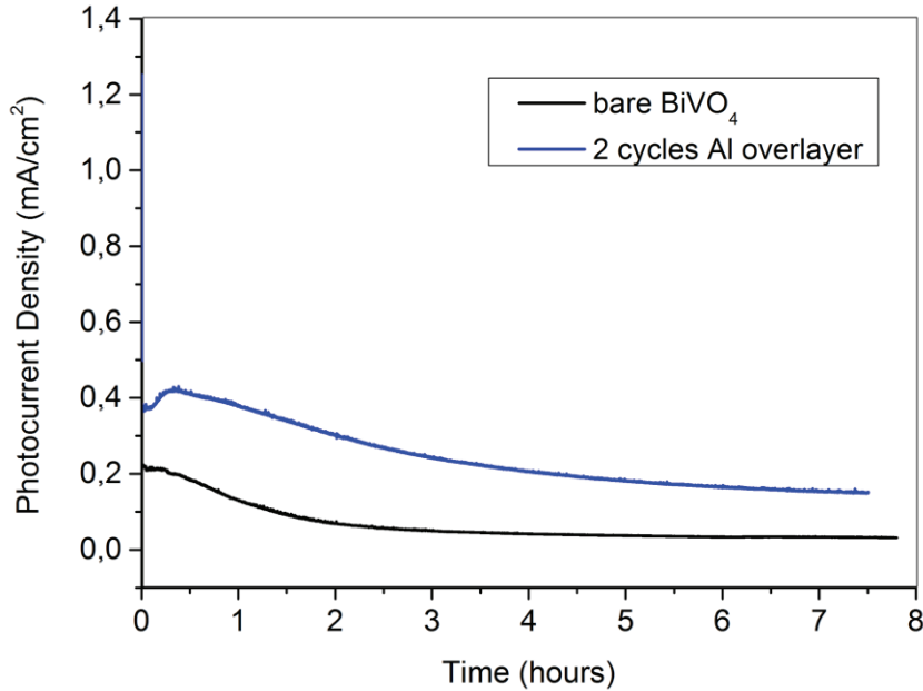
Figure 25. Stability test (chronoamperometry) plot for 2 cycles Al and bare BiVO 4 (electrolyte: 0.1 M Na-Pi pH 7, potential: 1.23 V vs RHE)
