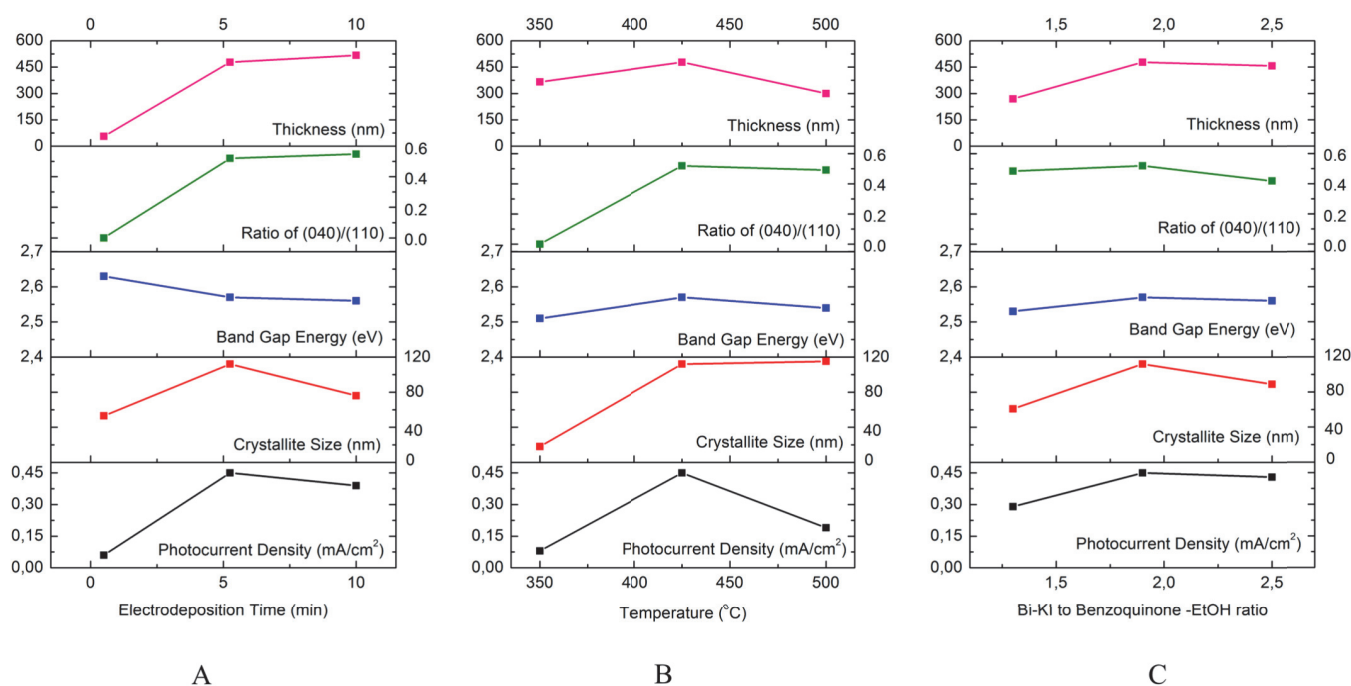
Figure S1. Summary of physico-chemical properties at various (A) electrodeposition time, (B) calcination temperature, and (C) Bi-KI to benzoquinone-EtOH ratio, plotted with respect to the photocurrent density at 1.23 V vs RHE
