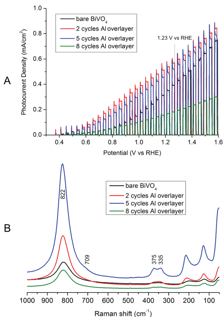
Figure 23. (A) LSV plot (electrolyte: 0.1M Na-Pi pH 7, scan rate: 10 mV/s) and (B) Raman spectra for bare \text{BiVO}_4 and Al-modified \text{BiVO}_4
