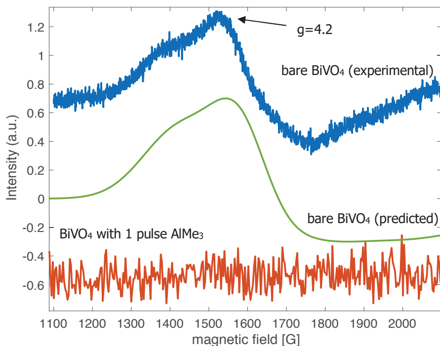
Figure 22. EPR spectra of bare \text{BiVO}_4 and \text{BiVO}_4 with 1 pulse of \text{AlMe}_3
