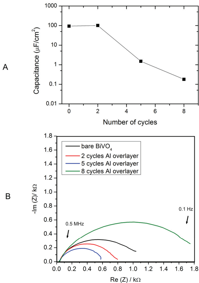
Figure 24. (A) Surface capacitance and (B) Nyquist impedance plots for bare and Al-modified \text{BiVO}_4
