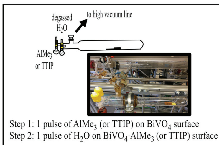
Figure 20. Surface modification of BiVO 4 electrode
