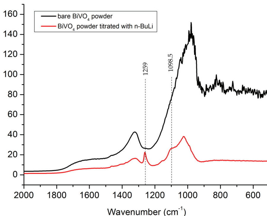
Figure 18. FTIR spectra of bare \text{BiVO}_4 and \text{BiVO}_4 titrated with n-BuLi
