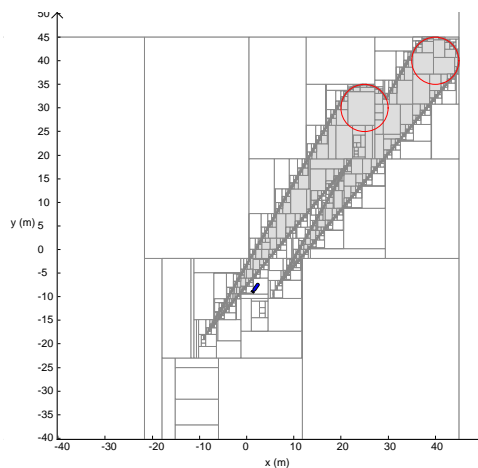
(d) Union of the backward reach taken separately at this same direction. The blue AUV does not belong to the backward reach set contrary to the one in the figure (c) at the same pose.
