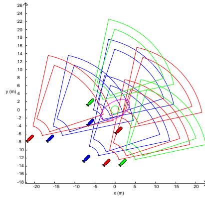
(b) 2D representation for the associated colored poses in the figure (a).
