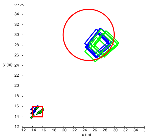
(d) Motion command ( 48^\circ, 18s ) corresponding to the red dot in the penumbra in the figure (a). Some of the robot poses (blue) end in the goal set and some (green) do not after this motion command (only partially).
