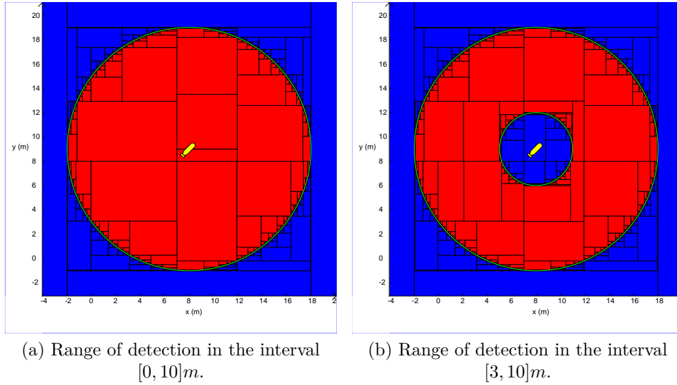
Figure 5.1: Visibility area for an isotropic sensor with limited ranges. The position of the robot is represented by the yellow AUV. The heading is not significant. The green line shows the contour.
