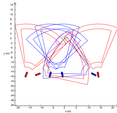
(f) Same definition for the 2D representation as in (d) where it corresponds to poses in the figure (e).
