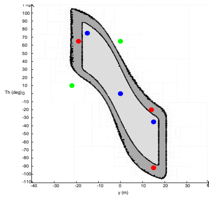
(c) Registration map in the (y - \theta) plane with x = -10m . Some poses are defined by dots.
