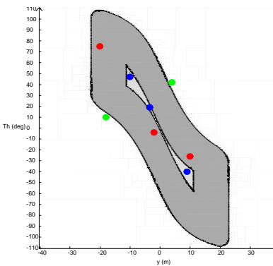
(d) Registration map in the (y - \theta) plane with x = -10m . Some poses are defined by dots.
