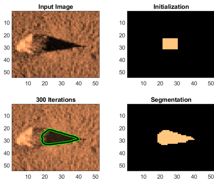
Figure 2.23: Snake algorithm to extract the shadow.
