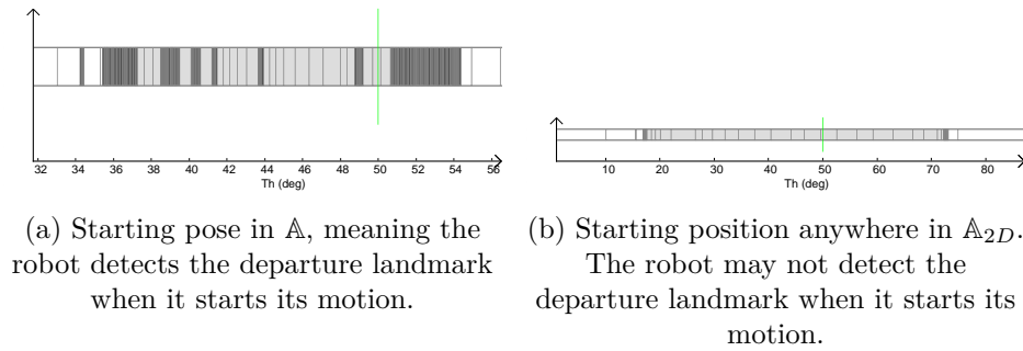
Figure 6.53: \Theta_{\mathbb{A}\mathbb{B}} using both methods for the departure area. The selected direction ( \theta_d = 50^\circ ) is the one that was used for the previous figures (green line).
