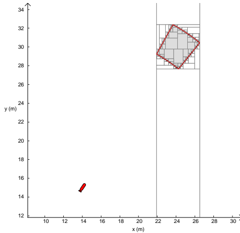
Figure 6.19: Set of positions after a motion command (\theta_d, t) = (56^\circ, 18s) starting from the initial pose (15, 15, 56^\circ) represented by the red AUV.
