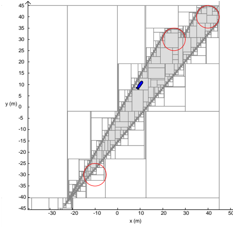
(c) Backward reach set of \mathbb{A} \cup \mathbb{B} at this same direction since 55^\circ \in \Theta_{\mathbb{A} \leftrightarrow \mathbb{B}} .
