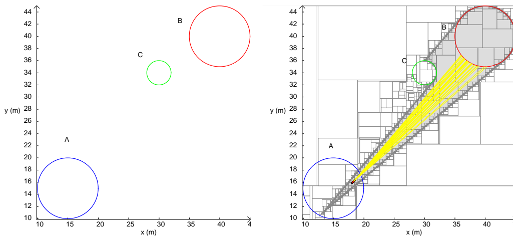
(a) Environment with a goal area \mathbb{B} from a relocation area \mathbb{A} with an obstacle or another relocation area \mathbb{C} . (b) 2D backward reach set at \theta_d = 45^\circ (green line in the figure (e)) where some trajectories in yellow are represented from a possible initial location at the red AUV.
