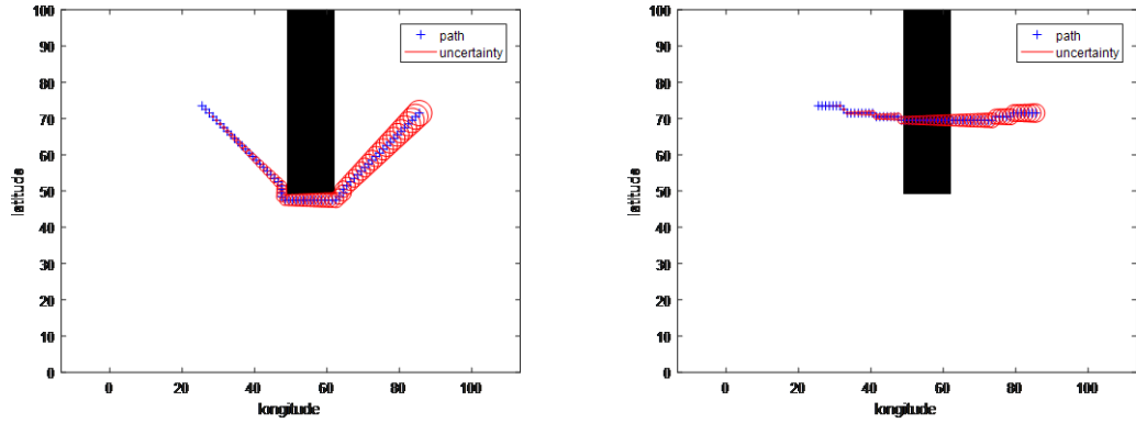
(a) Path getting around the high cost region where the final uncertainty asked was \epsilon_f < 5m . The final uncertainty is actually 3.48m and the cost path 151. (b) Path going through the high cost region in black to respect the final uncertainty condition fixed at \epsilon_f < 3m . The path cost is 552 and the final uncertainty is 2.52m .
