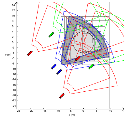
(c) Thick intersection of the thick visibility areas at the 3 blue poses.
