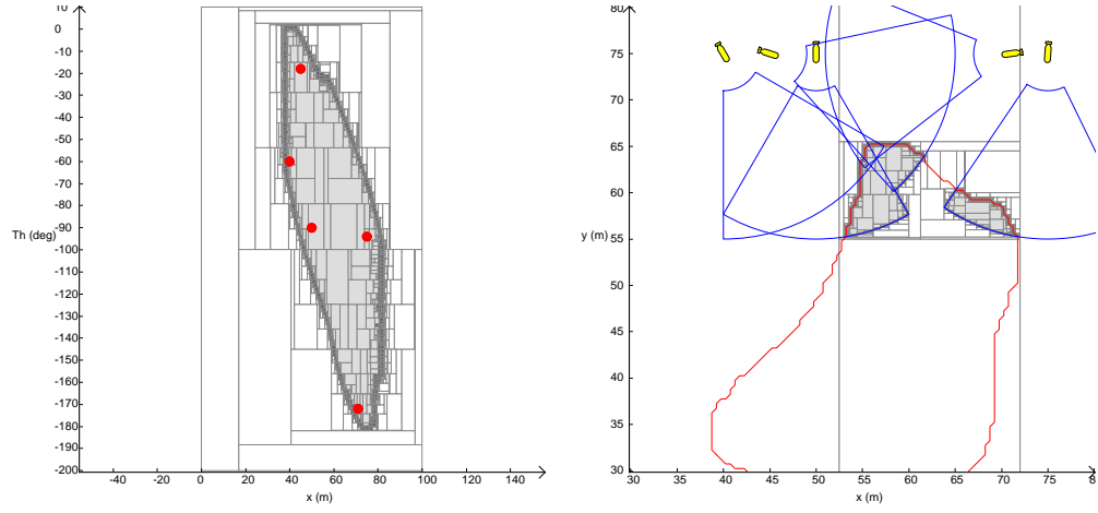
(a) Registration map with y = 75m fixed. The representation is in the plane (x - \theta) . (b) Representation in the (x - y) plane of the AUV poses depicted by red dots in the figure (a).
