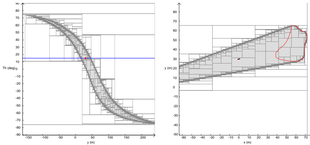
(a) (y, \theta_d) representation for the slice at x = 0m .
