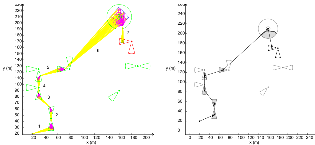
(c) Strategy execution with uncertain trajectories in yellow and with relocation process in magenta in the relocation areas. Number are given for the different sub-strategy. (d) Set of departure positions in each relocation area according to the strategy found. Grayscale convention for thin sets.
