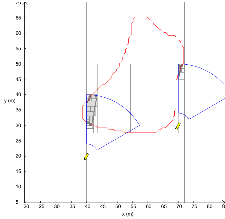
Figure 5.15: Set of visible points from the landmark by the sensor respecting the point of view at the two robots poses in Figure 5.14(d).
