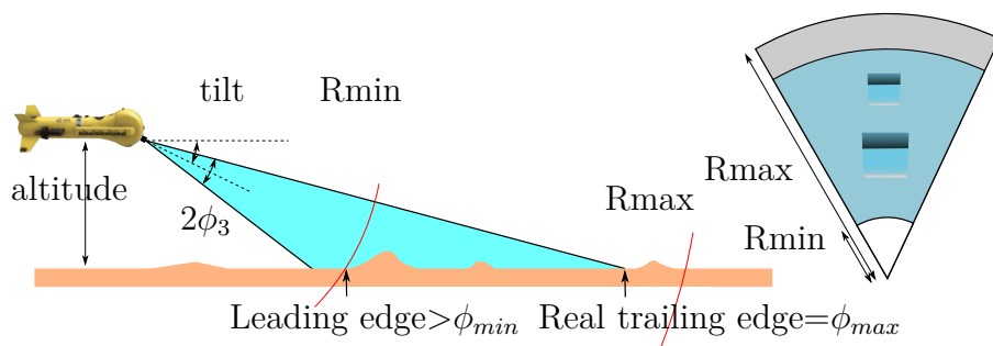
Figure 2.11: The ranges R_{min} and R_{max} do not correspond to the extremum \phi_{min} and \phi_{max} . On the top figure, the trailing edge does not correspond to \phi_{max} and R_{min} does not correspond to the real leading edge. This latter can be detected in the image (gray part). On the bottom figure, the leading edge has an angle bigger than \phi_{min} that is supposed being at R_{min} . The real trailing edge is at \phi_{max} but it does not correspond to R_{max} . The trailing edge can be detected in the image (gray part).
