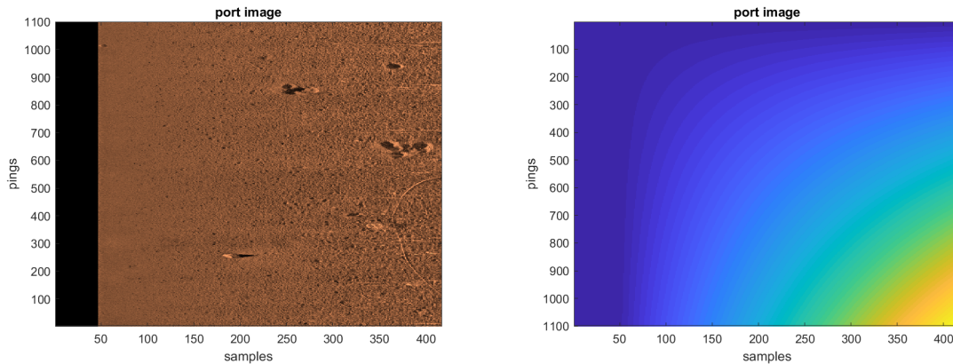
(a) Original port image after TVG correction and water-column removal.
