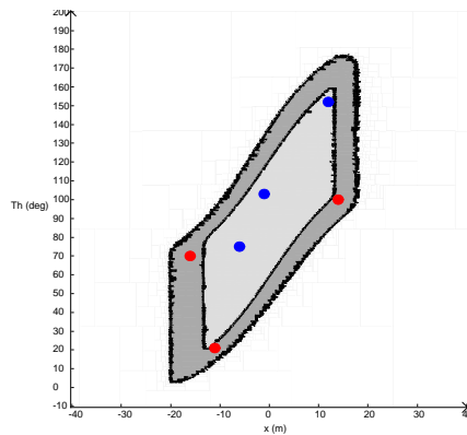
(e) Registration map in the (x - \theta) plane with y = -15m .
