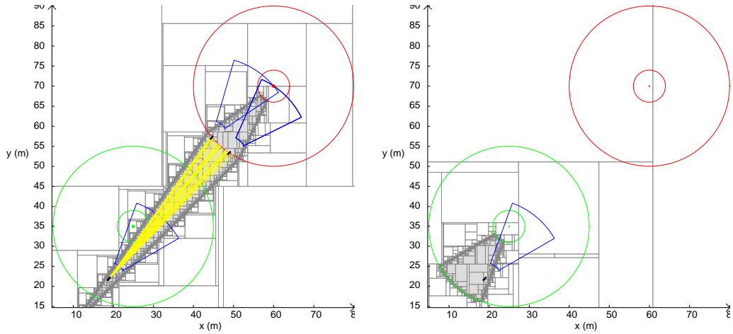
(a) 2D backward reachability of the registration map associated to the goal landmark (red) at the defined direction \theta_d = 50^\circ .
