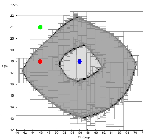
(a) Thick solution of the set TC(\mathbf{q}_0) . Grayscale convention for thick sets.
