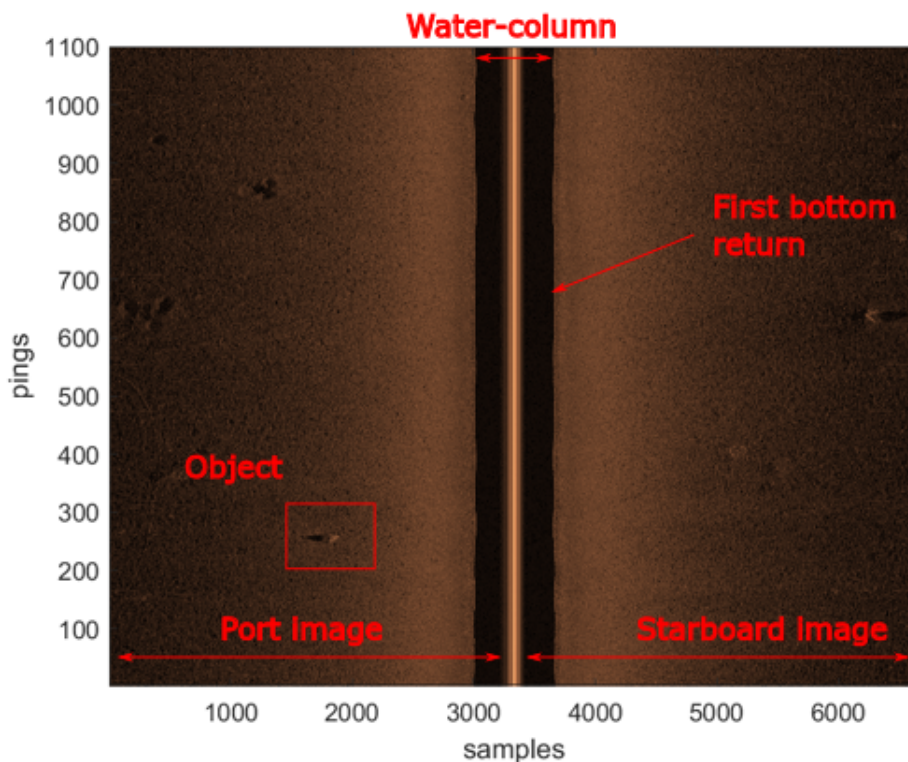
Figure 2.7: Water-fall image for a sidescan sonar.
