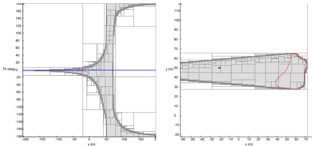
(c) (x, \theta_d) representation for the slice at y = 50m .
