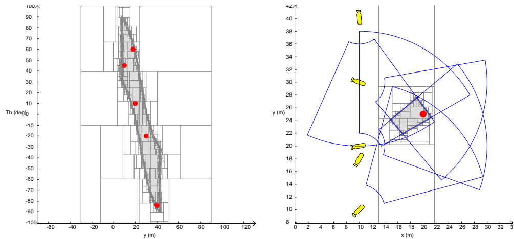
(c) Registration map with x = 20m fixed. The representation is in the plane (y - \theta) . (d) Representation in the (x - y) plane of the AUV poses depicted by red dots in the solution set associated.
