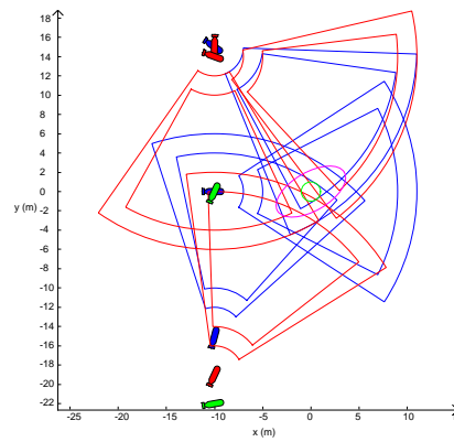
(d) 2D representation of the selected poses with the color associated in the figure (c).
