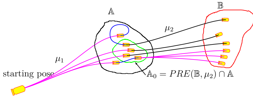
(b) Path execution. Magenta paths depict the potential paths due to the drift of the robot at different poses. Some paths already end in A_0 and two others need a relocation represented by the blue paths.
