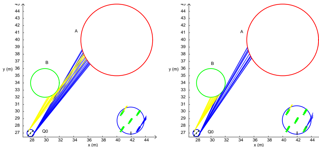
(c) \theta_d = 56^\circ inside the penumbra (red line in the figure (e)), where some position guarantees to reach A (position in blue AUV and blue trajectories) and others (green AUV and yellow trajectories) with trajectories that cross B . Similarly a zoom is provided. (d) \theta_d = 60^\circ outside the solution set (green line in the figure (e)), where no initial position (green AUV) can reach for sure A without ambiguity with B or even reachability of A . Similarly a zoom is provided.
