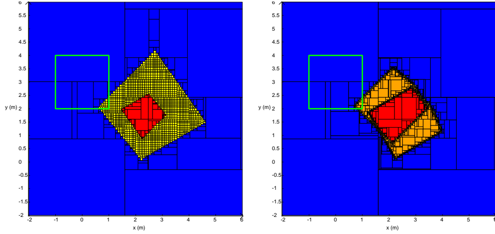
(a) Classical set inversion. Blue boxes are outside, red ones are inside and yellow ones no conclusion can be made.
