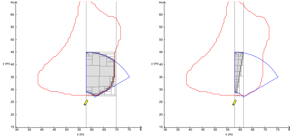
(a) Set of visible points from the landmark by the sensor at the robot pose (58, 25, 60^\circ) . (b) Set of visible points from the landmark by the sensor at the robot pose (58, 25, 60^\circ) and respecting the point of view [\theta_{detection}] .
