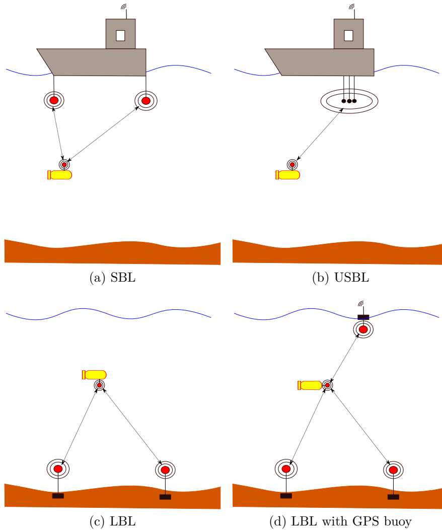
Figure 1.12: Acoustic-based navigation configuration
