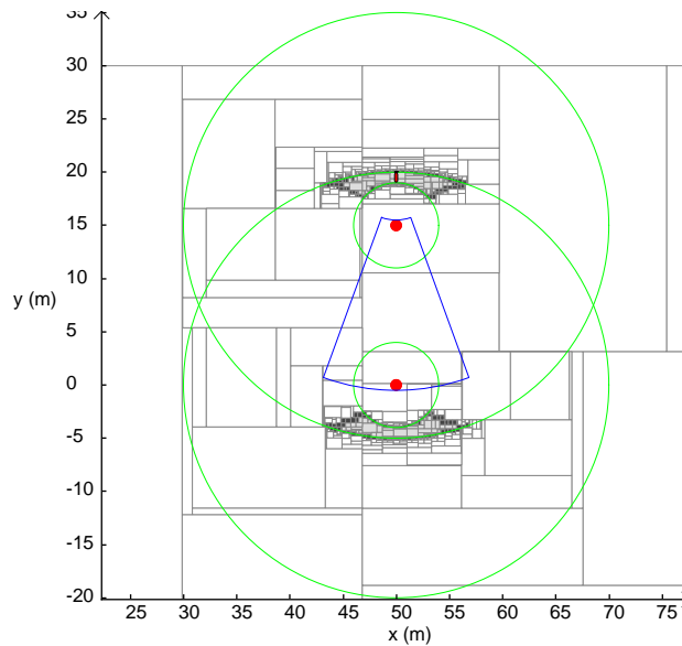
(a) \mathbb{P}_{\mathbb{A}\mathbb{B}}^{2D} with y_b = 15m . The two registration maps are not connected.
