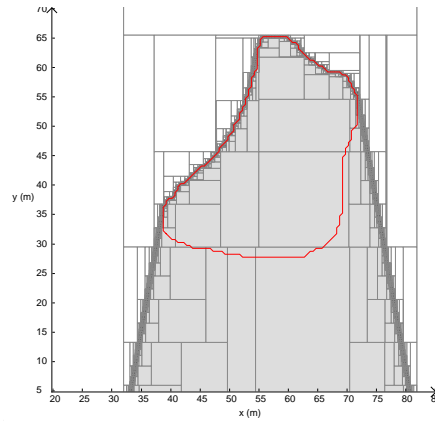
(b) Minkowski sum to compute the (x, y) robot position consistent with the point of view on the shape landmark corresponding to the set \mathbb{P}_{view}^{\mathbb{B}}([\theta_{detection}]) .
