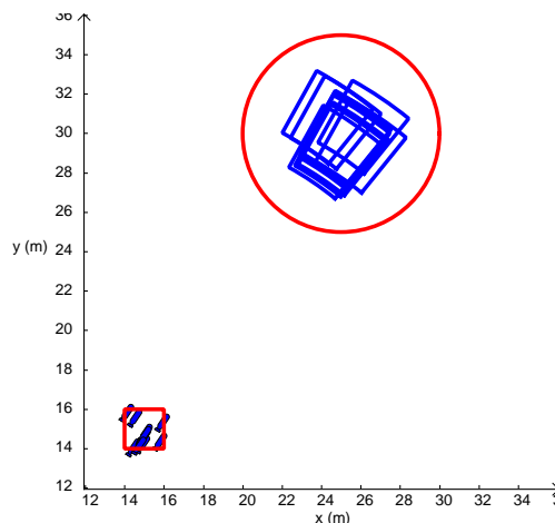
(b) Motion command ( 56^\circ, 18s ) corresponding to the blue dot inside the solution set in the figure (a). All the robot poses end in the goal set after this motion command.
