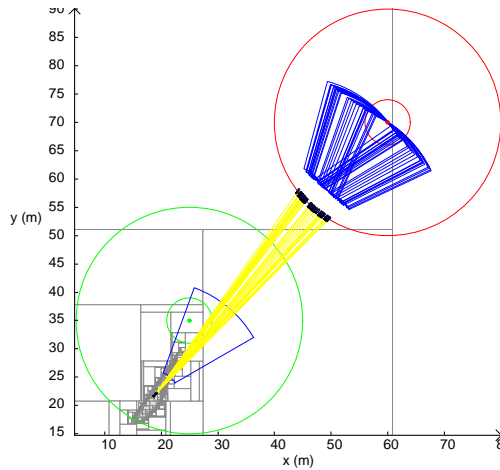
(c) Intersection between the 2D backward reachability and the registration map of the departure landmark at the direction \theta = 50^\circ . Departure area to guarantee the reachability at \theta_d = 50^\circ .
