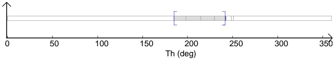
(b) Solution of \Theta_{\mathbb{B} \rightarrow \mathbb{A}} .
