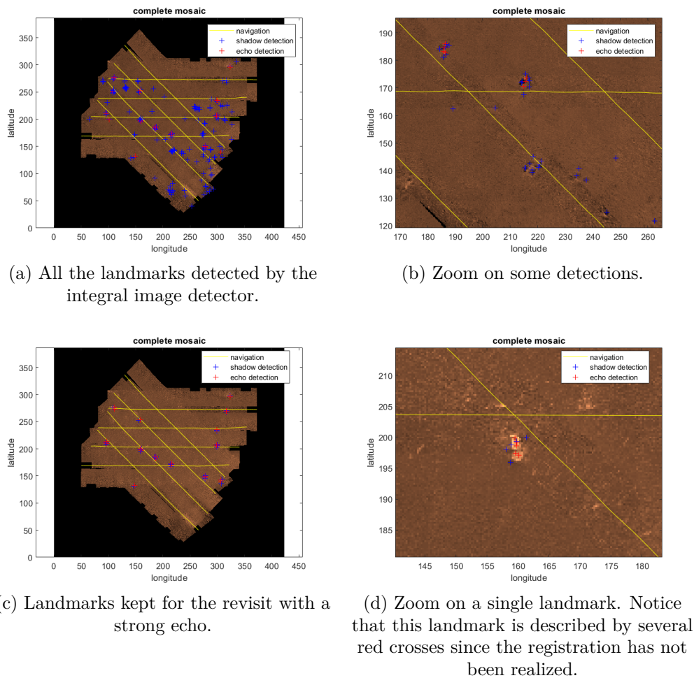
Figure 2.30: Filtering step on real data. The complete mosaic of some sonar passes on the survey area. The sonar images have not been registered.
