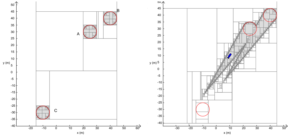
(a) Goal set defined by three non connected sets \mathbb{A} , \mathbb{B} and \mathbb{C} .
