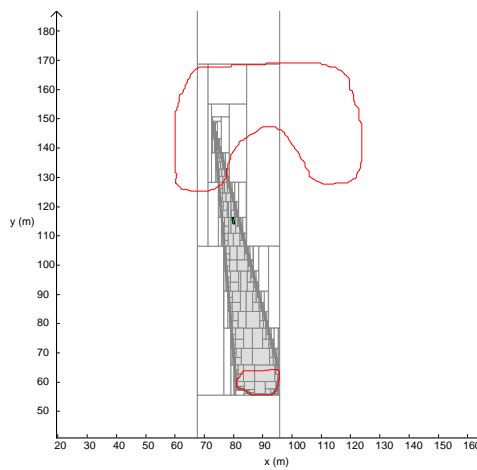
(c) 2D backward reach at \theta_d = 280^\circ corresponding to the green line in the figure (a).
