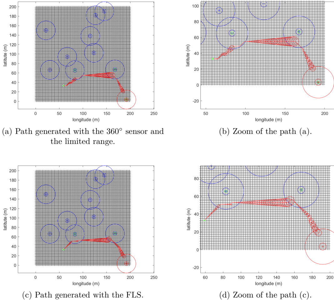
Figure 3.12: Comparison between the paths found with the two sensors. The black crosses show the grid (the states). The blue points are the landmarks with the associated range detection drawn by blue circles. It is drawn in red similarly for the target. The green asterisk is the initial configuration. The path is in red with the uncertainty circles at 2\sigma in red too.
