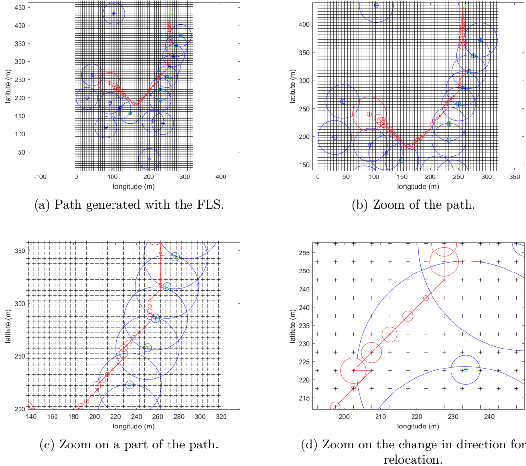
Figure 3.14: Path found for the revisit with the FLS. The black crosses show the grid (the states). The blue points are the landmarks with the associated range detection drawn by blue circles. It is drawn in red similarly for the target. The green asterisk is the initial configuration. The path is in red with the uncertainty circles at 2\sigma in red too.
