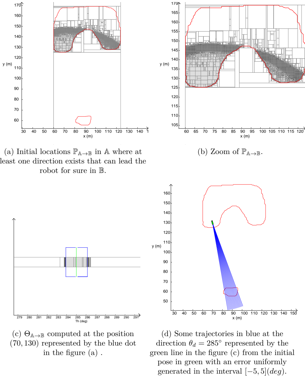
Figure 6.15: Computation of \mathbb{P}_{\mathbb{A} \rightarrow \mathbb{B}} . Many little boxes due to the resolution of the initial image and the size of the boxes that are getting smaller with the distance to \mathbb{B} .
