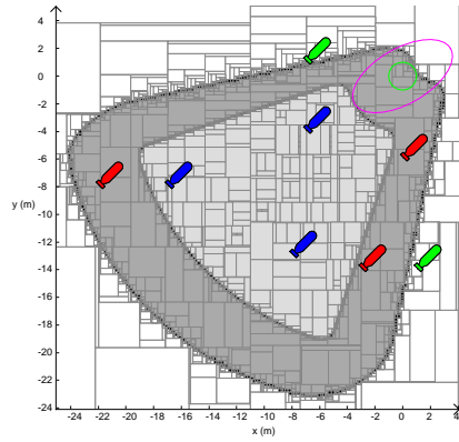
(a) Registration map at heading 45^\circ . The contours of the thick landmark are represented in green for \mathbb{B}^- and in magenta for \mathbb{B}^+ . Some AUV poses are chosen for a 2D representation.
