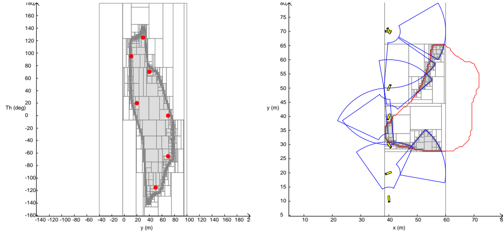
(c) Registration map with x = 40m fixed. The representation is in the plane (y - \theta) . (d) Representation in the (x - y) plane of the AUV poses depicted by red dots in the figure (c).
