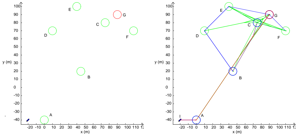
(a) Environment with disk relocation areas in green and goal area in red. The initial pose is represented by the blue AUV. (b) Graph built with the path found in red. Blue links are direct links between two relocation areas, and green links are high level links between a set of disconnected relocation areas (at least 3).
