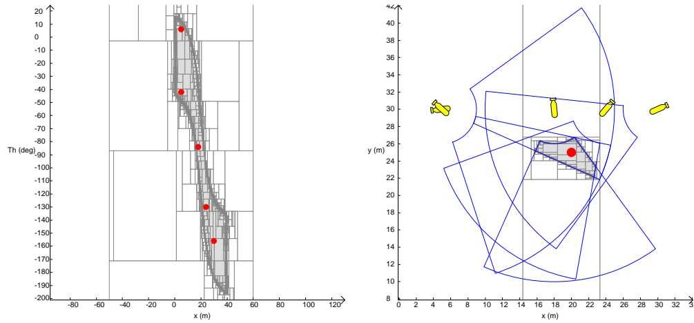
(a) Registration map with y = 30m fixed. The representation is in the plane (x - \theta) . (b) Representation in the (x - y) plane of the AUV poses depicted by red dots in the solution set associated.
