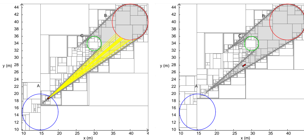
(c) 2D backward reach set at \theta_d = 39^\circ (green line in the figure (e)) where some trajectories in yellow are represented from a possible initial location at the red AUV. (d) 2D backward reach set at \theta_d = 36^\circ (red line in the figure (e)), no possible link at this direction.
