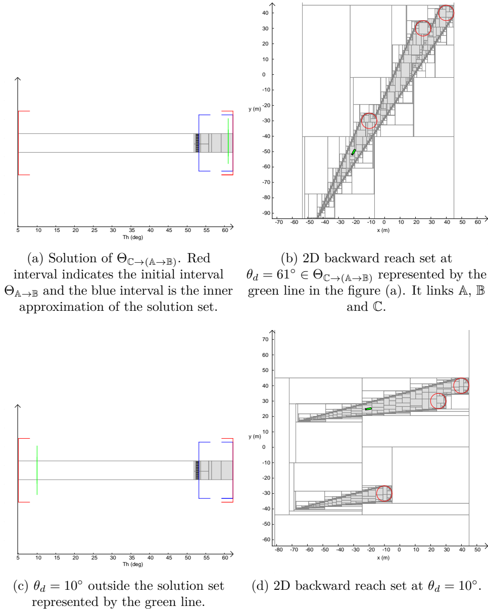
Figure 6.13: Different sets of direction linking A, B and C. The blue intervals indicate the inner approximation of \Theta_{C \rightarrow (A \cup B)} and the red brackets are the intervals (set of directions) that link A to B. Grayscale convention for thin sets.
