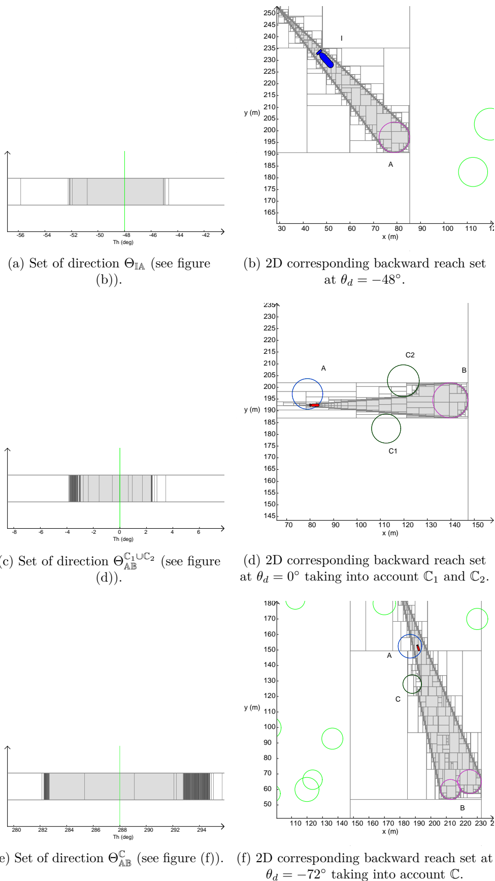
Figure 6.43: Intermediate reachability between the blue departure area and the intermediate goal area in magenta taking into account potential other relocation areas in black.
