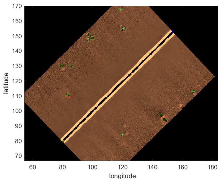
Figure 2.25: Detections on the mosaic. Red crosses indicate echo detection and green crosses shadow detections.
