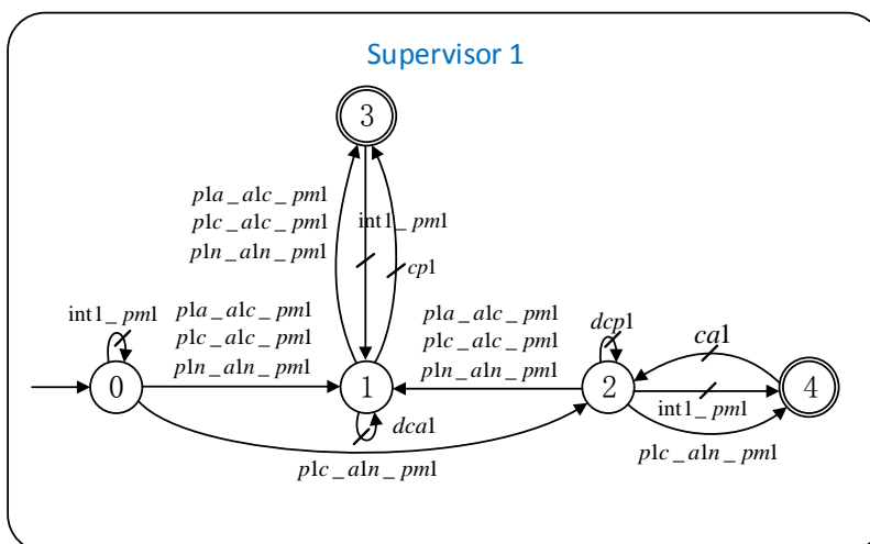
Figure 5.14 Model of supervisor 1
