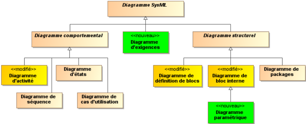
Figure C.6 Taxonomie du diagramme SysML
