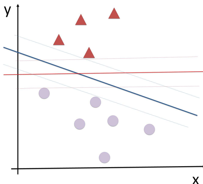
FIGURE 1.6 – Algorithme SVM.
