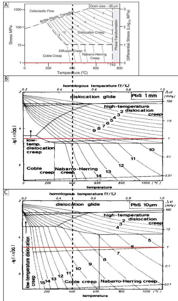
Figure 33. Deformation mechanism maps comparison between pyrite and galena. The deformation maps are normalized at the same temperature. Red line indicates the same stress value. A. Deformation map of pyrite (from Barrie et al., 2011 ). B-C. Deformation map of galena (from Atkinson, 1976 ).
