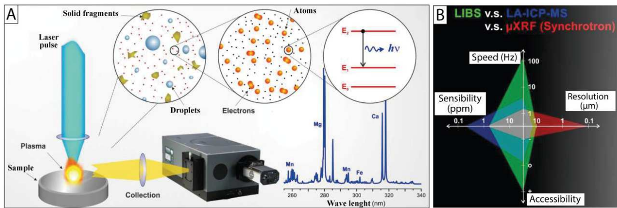
Figure 39: A: Schematic representation of the LIBS technique. B: Schematic comparison of LIBS with other traditional trace element analyzer such as LA-ICP-MS or \mu -XRF (synchrotron)
