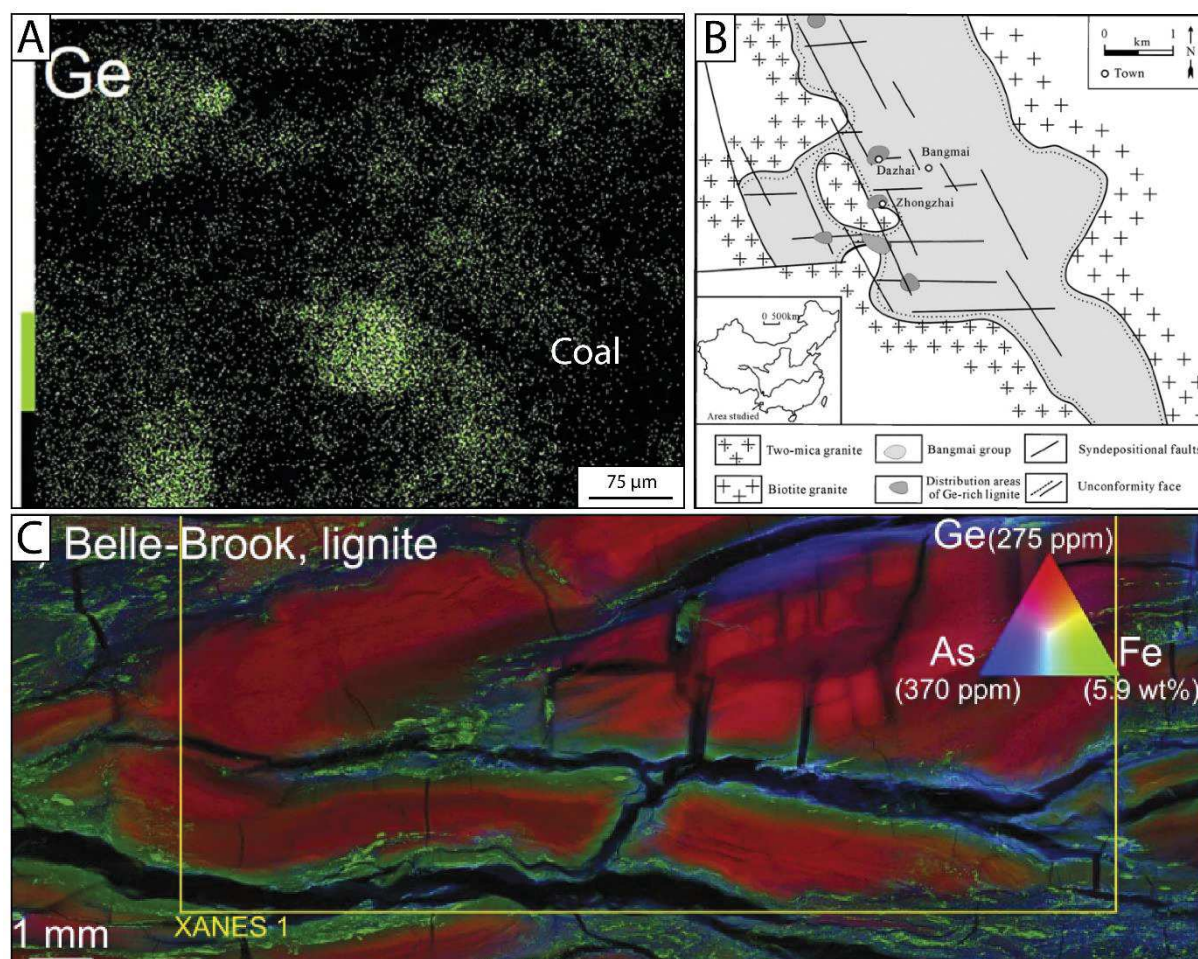
Figure 26. A. Elemental map of Ge in coal from the Blue Gem deposit-Kentucky coal field (from Hower et al. , 2018). B. Geological map of the Lincange coal field with noted the Ge-rich lignite areas close to the faults (from Hu et al. , 2009). C. SXRF maps of the Belle Brooke (New Zealand) coal samples (a) lignite, red = Ge, green = Fe, blue = As and (b) wood, showing the distribution of Ge (from Etschmann et al. , 2017).
