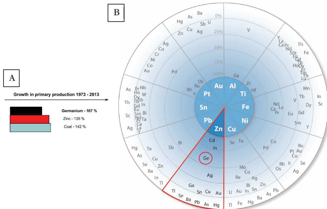
Figure 14. A. Growth in primary production of Germanium from 1973 to 2013 (from Frenzel et al. 2017 and reference herein). B. Wheels of the relation between host metals in the inner circle and by-product metals in the outer circle. By-product elements appear at distances proportional to the percentage of their total production in the outer circle (from Nassar et al., 2015)
