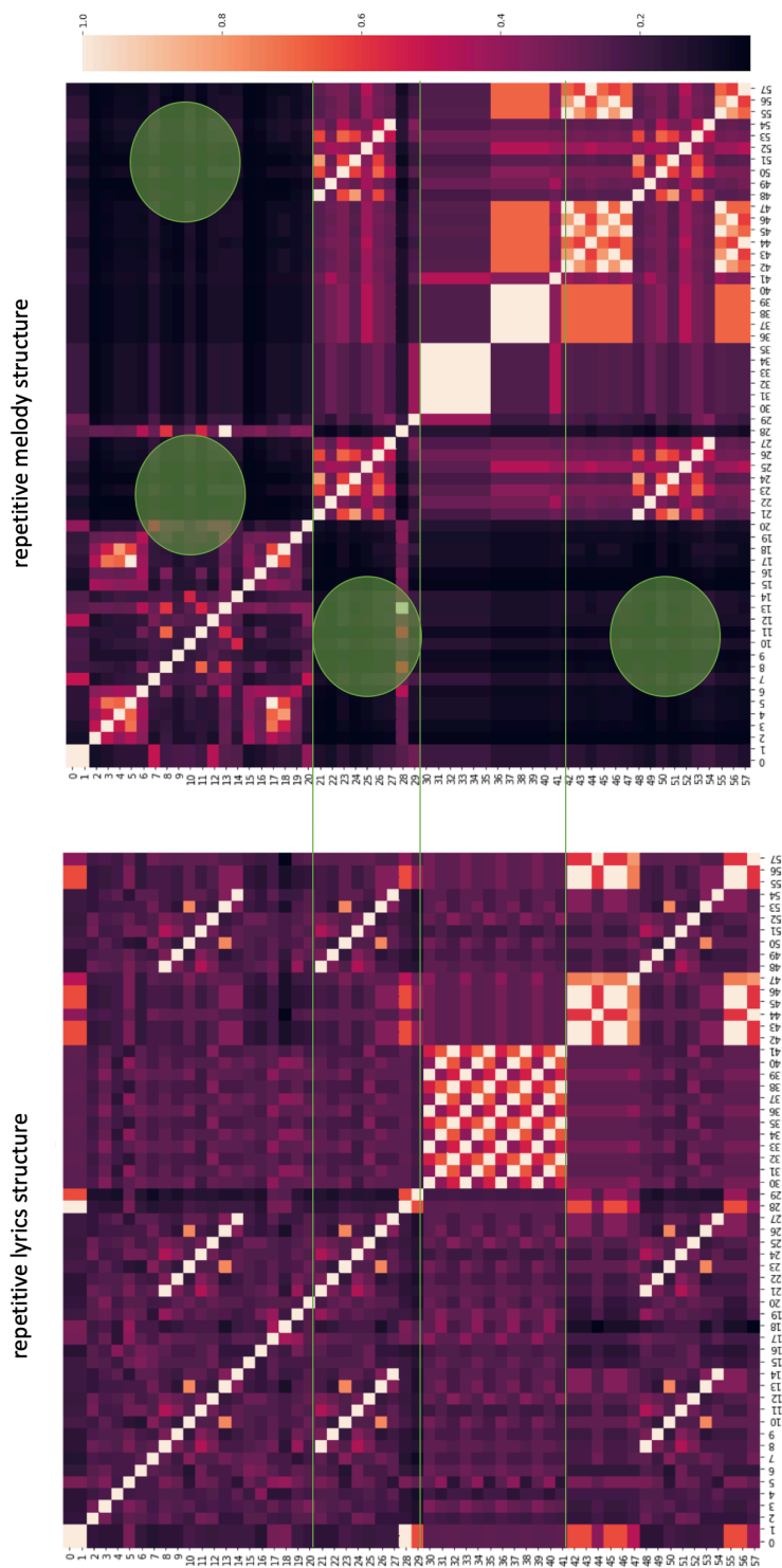
Figure 3.6: Octave-shifted chorus appears as repetition in melody structure (green circles).
