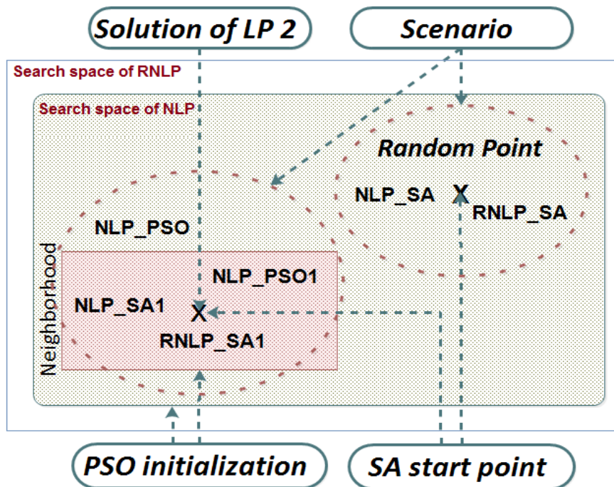
Figure 3.2 Algorithms initialization scenarios.
