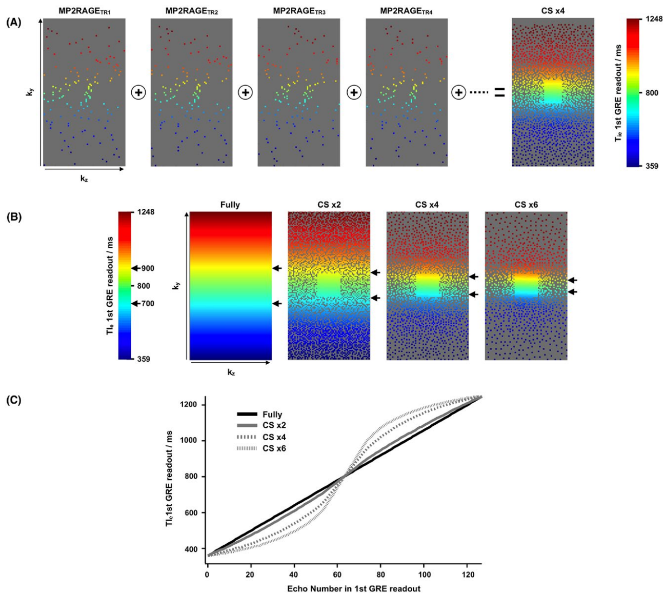
FIGURE 1 (A) Encoding trajectories within the k -spaces for a CS-MP2RAGE sequence with an acceleration factor of 4. The trajectories in the k_y - k_z plane during the first four MP2RAGE_{TR} and their combination are shown. The example of the first GRE readout (set at TI_1 value of 800 ms) is shown. TI_{e(n)} within the 1st GRE readout are color-encoded (see color scale). (B) Effect of the CS acceleration factors ( \times 2 , \times 4 , and \times 6 ) on the TI_e position in the k -space. The example of the first GRE readout (set at TI_1 value of 800 ms) is shown. The arrows point at TI_e = 700 and 900 ms to show the increasing concentration of the TI_e at the center of the k -spaces. (C) Curves of TI_e as a function of the echo number in the GRE readout, for Fully and accelerated acquisitions
