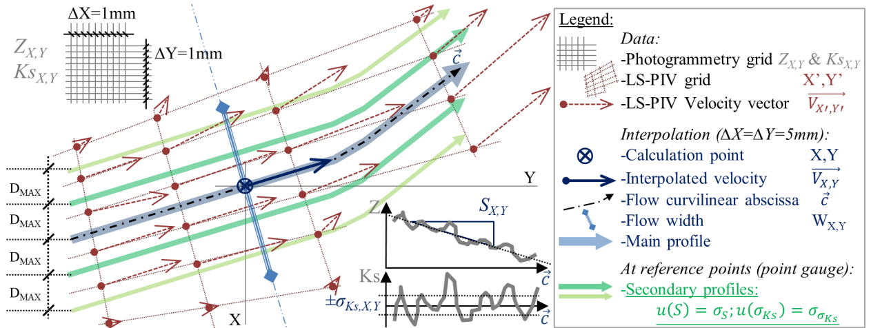
Figure 6.9 – Sketch of the friction law parameters extraction algorithm: extraction of the flow slope S_{X,Y} and roughness standard deviation \sigma_{K_{X,Y}} along curvilinear profiles following the flow direction defined by LS-PIV velocity data. Main profile defined parallel to the main stream line passing by X,Y and additional uncertainty measurements at reference points (underlined steps).
