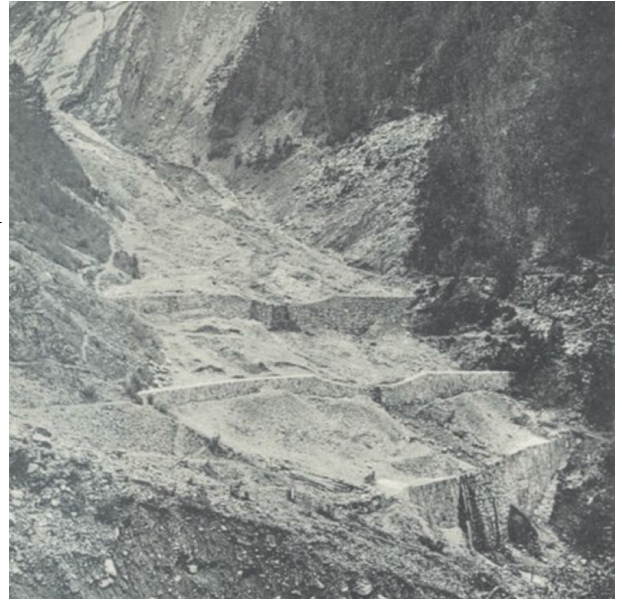
Figure 1.3 – Headwater-moraine-retention-dams in the Ravin des Arandellys (74 – FRA.) (Eaux et Forêts, 1911a)
