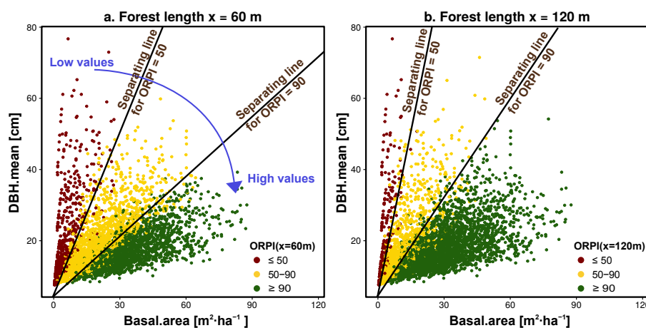
FIGURE 3.3 – Illustration of the clockwise motion of ORPI values for a rock volume of 1 \text{ m}^3 at forest lengths x=60 m (a.) and x=120 m (b.). Points are coloured according to ORPI(x) . The separating lines between plots were ORPI(x) < 90 (or 50) and plots were ORPI(x) \geq 90 (or 50) are shown. (Figure adapted from Dupire et al. (2016a))
