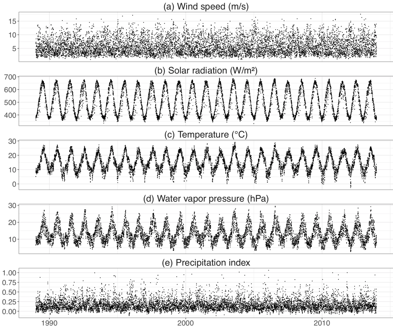
Figure 9.4: The time-series of daily average observation of 5 variables from 1989 to 2013.
