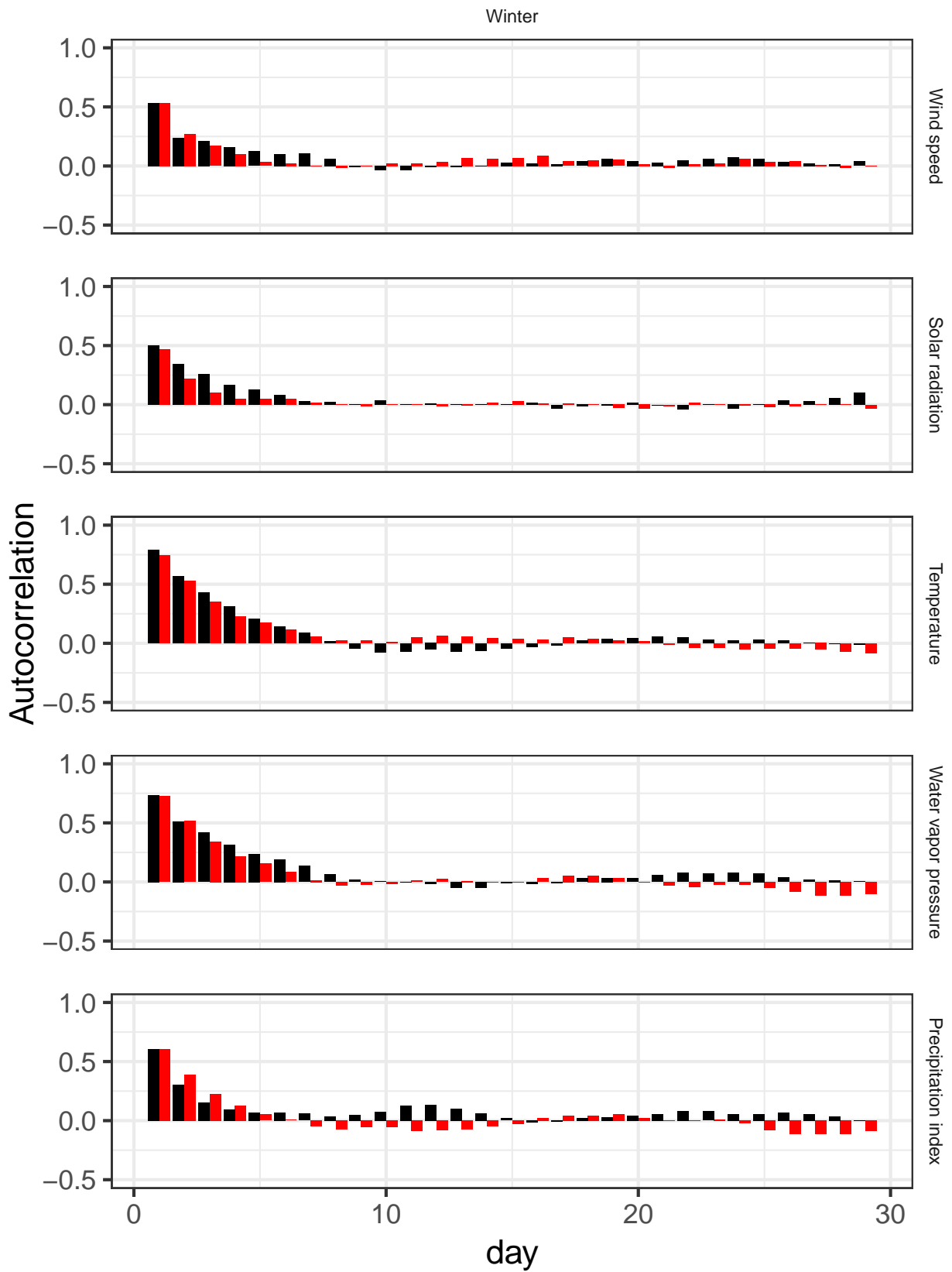
Figure 9.22: Auto-correlation functions (ACF) of observed (in black) and simulated (in red) data for the winter season within the 1989-2013 period.
