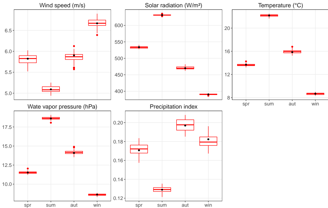
Figure 9.12: Statistics, illustrated with boxplots for each season, of the average value for each variable over the 25-years period. Black points refer to the observed average value. The statistics of the simulated values, in red, rely on the 50 replications of 25-years simulations.
