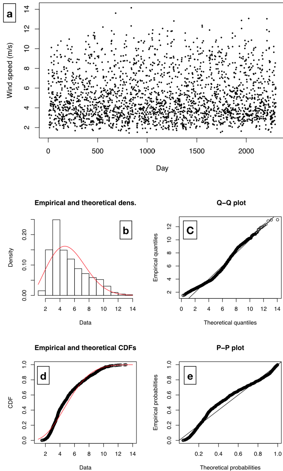
Figure 9.5: (a) Time series of average daily wind speed (m/s) in summer periods from 1989 to 2013. (b) Histogram of data and the fitted Weibull distribution (red line) with parameters (shape, scale) = (2.336, 5.922). (c) Q-Q (quantile-quantile) plot between empirical quantile of data (y-axis) and theoretical quantiles (x-axis). (d) Comparison of cumulative distribution function between the data (in black) and theoretical Weibull distribution (in red). (e) P-P (probability-probability) plot between empirical quantile of data (y-axis) and theoretical quantiles (x-axis).
