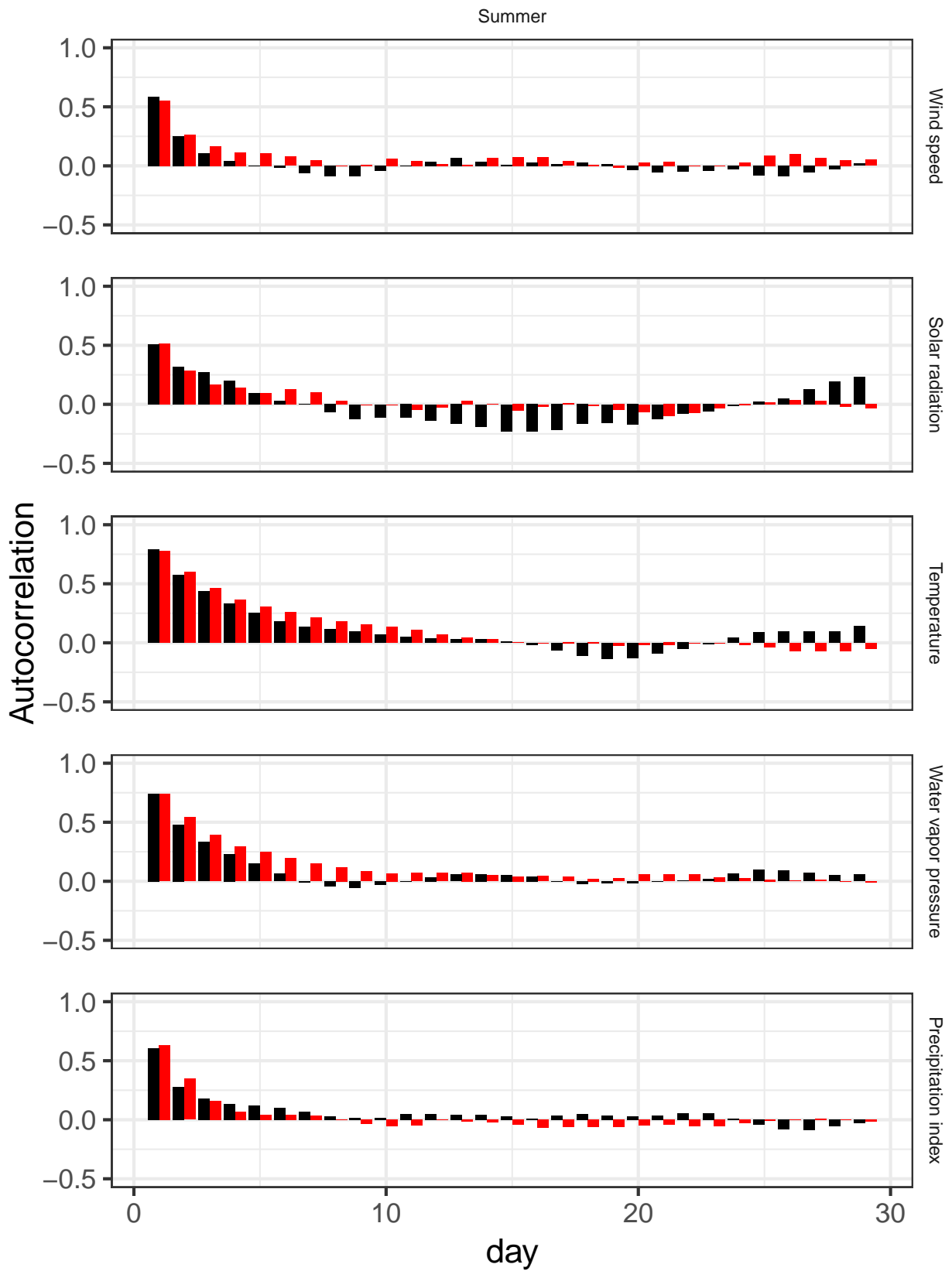
Figure 9.20: Auto-correlation functions (ACF) of observed (in black) and simulated (in red) data for the summer season within the 1989-2013 period.
