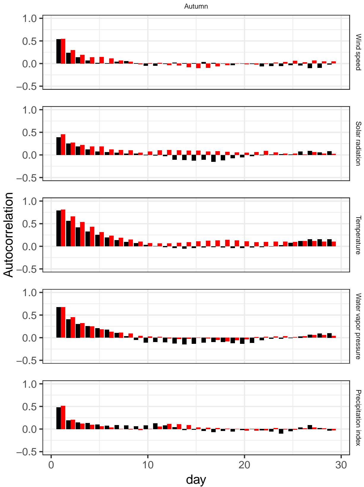
Figure 9.21: Auto-correlation functions (ACF) of observed (in black) and simulated (in red) data for the autumn season within the 1989-2013 period.
