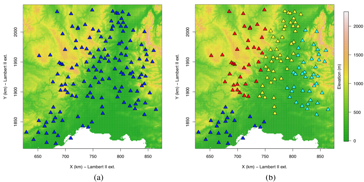
Figure 9.2: (a) 146 daily rainfall gauge stations in Cévennes Vivarais within the 1989-2013 period. (b) 146 gauges stations are partitioned into 4 clusters by using the k-means clustering. The clusters are located in the Mediterranean area (in dark blue), the Hill area (in cyan), the Piedmont area (in yellow) and the Mountain ares (in red).
