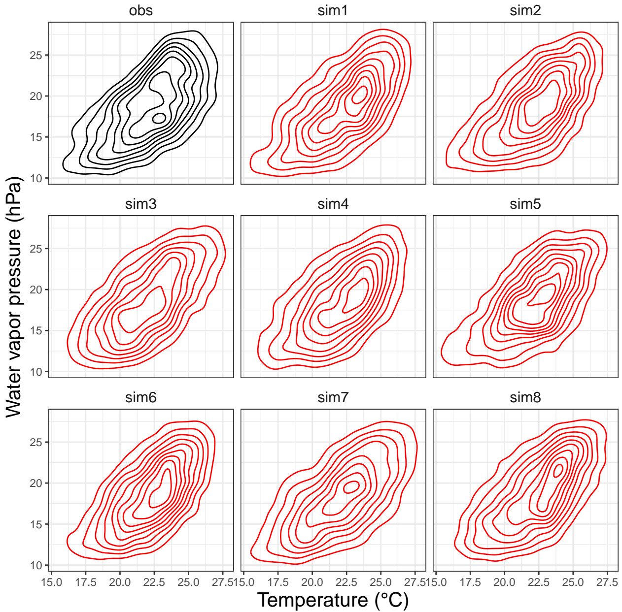
Figure 9.18: Comparison of bivariate distributions of temperature and water vapor pressure between the observation data and simulation data. There are one observation plot and 8 simulation plots. The span of each data is 25-years for summer periods. This displays the variability of 25-years chunks, and suggest there is no obvious difference between any of them and the observed.
