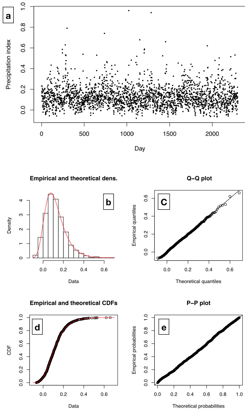
Figure 9.9: (a) Time series of daily precipitation index in summer periods from 1989 to 2013. (b) Histogram of data and the fitted Gumbel distribution with parameters (location, scale) = (0.0768, 0.0814). (c) Q-Q (quantile-quantile) plot between empirical quantile of data (y-axis) and theoretical quantiles (x-axis). (d) Comparison of cumulative distribution function between the data (in black) and theoretical Gumbel distribution (in red). (e) P-P (probability-probability) plot between empirical quantile of data (y-axis) and theoretical quantiles (x-axis).
