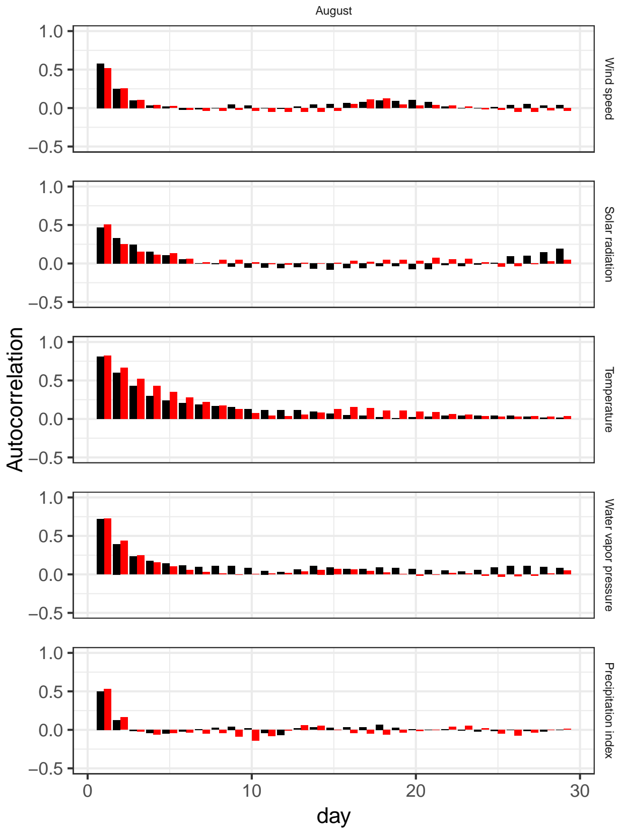
Figure 9.24: Representations of the auto-correlation function of observed data and simulated data for each variable in August periods. Black represents the observed data and red represents the simulated data.
