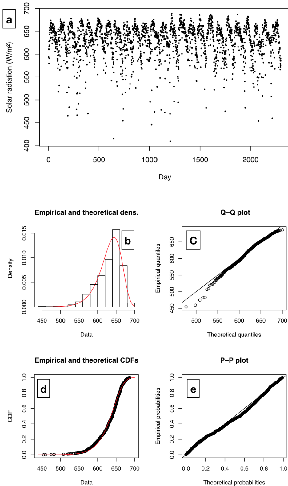
Figure 9.6: (a) Time series of average daily solar radiation ( \text{W/m}^2 ) in summer periods from 1989 to 2013. (b) Histogram of data and the fitted Weibull distribution with parameters (shape, scale) = (24.78, 645.4). (c) Q-Q (quantile-quantile) plot between empirical quantile of data (y-axis) and theoretical quantiles (x-axis). (d) Comparison of cumulative distribution function between the data (in black) and theoretical Weibull distribution (in red). (e) P-P (probability-probability) plot between empirical quantile of data (y-axis) and theoretical quantiles (x-axis).
