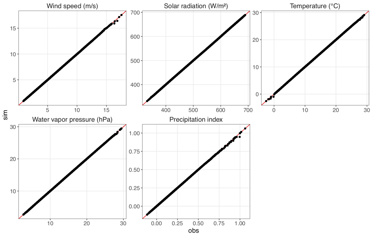
Figure 9.13: QQ-plots for each variable by comparing the marginal distributions between 25-years observed and one 25-years simulation.
