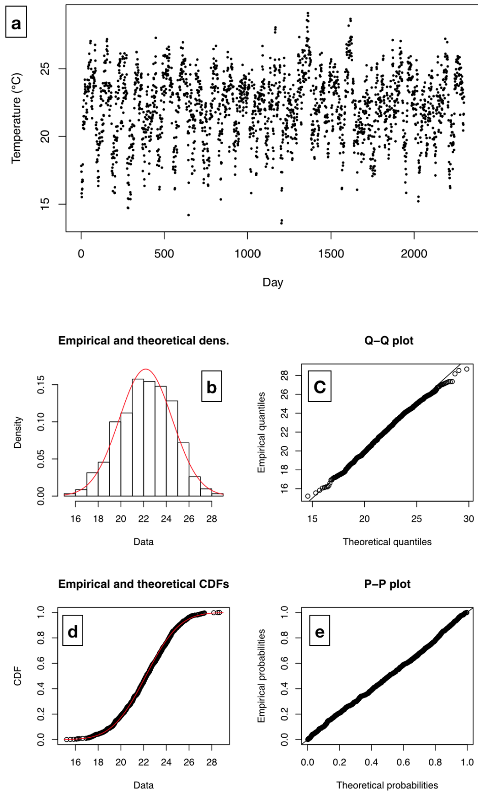
Figure 9.7: (a) Time series of average daily temperature (Celsius) in summer periods from 1989 to 2013. (b) Histogram of data and the fitted Normal distribution with parameters (mean, sd) = (22.18, 2.332). (c) Q-Q (quantile-quantile) plot between empirical quantile of data (y-axis) and theoretical quantiles (x-axis). (d) Comparison of cumulative distribution function between the data (in black) and theoretical Normal distribution (in red). (e) P-P (probability-probability) plot between empirical quantile of data (y-axis) and theoretical quantiles (x-axis).
