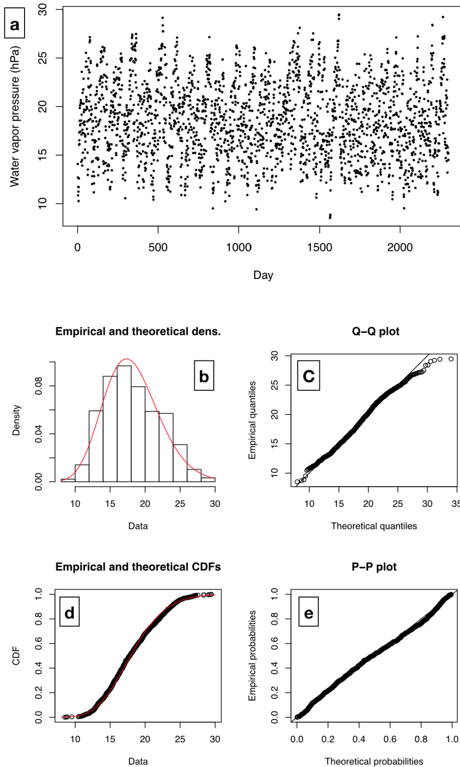
Figure 9.8: (a) Time series of average daily water vapor pressure (hPa) in summer periods from 1989 to 2013. (b) Histogram of data and the fitted Gamma distribution with parameters (shape, rate) = (21.02, 1.155). (c) Q-Q (quantile-quantile) plot between empirical quantile of data (y-axis) and theoretical quantiles (x-axis). (d) Comparison of cumulative distribution function between the data (in black) and theoretical Gamma distribution (in red). (e) P-P (probability-probability) plot between empirical quantile of data (y-axis) and theoretical quantiles (x-axis).
