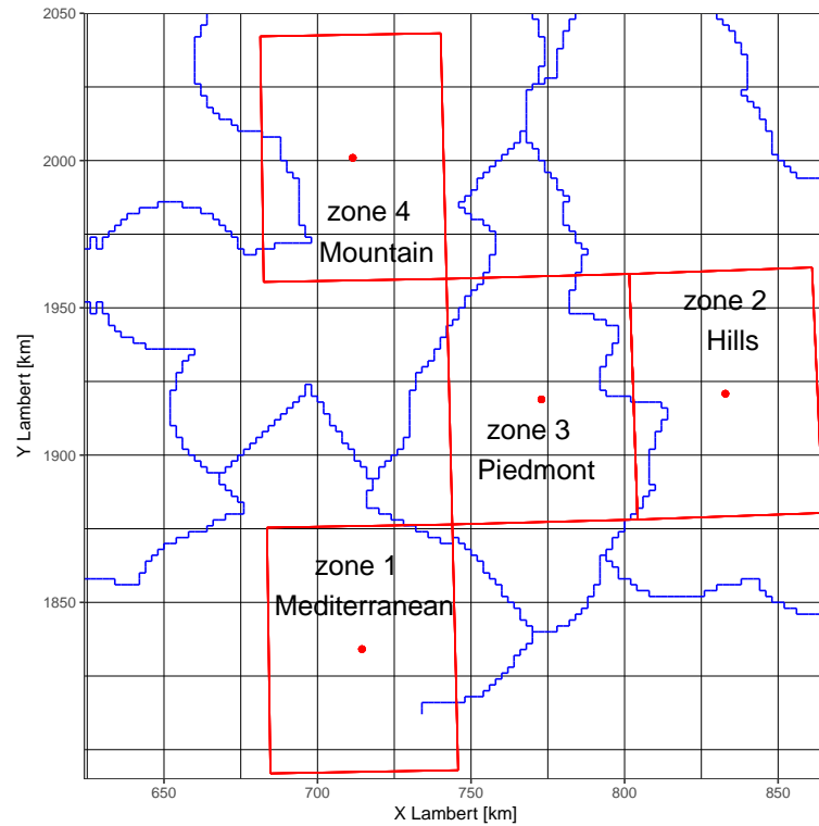
Figure 9.3: Location of ERA-Interim pixel (red rectangle) associated with each zone. Rectangle (in red) is the 0.75^\circ \times 0.75^\circ grid associated to each zones. Points (in red) are the centers of the grids.
