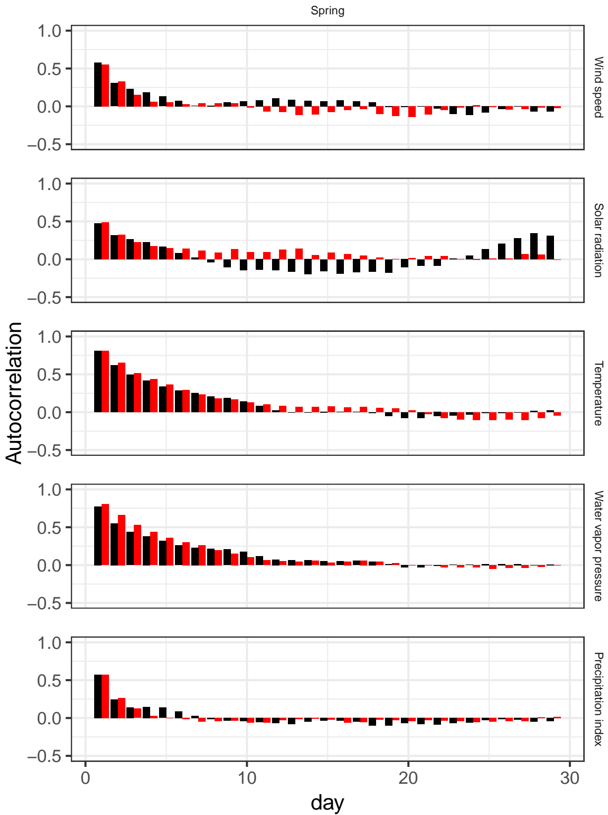
Figure 9.19: Auto-correlation functions (ACF) of observed (in black) and simulated (in red) data for the spring season within the 1989-2013 period.
