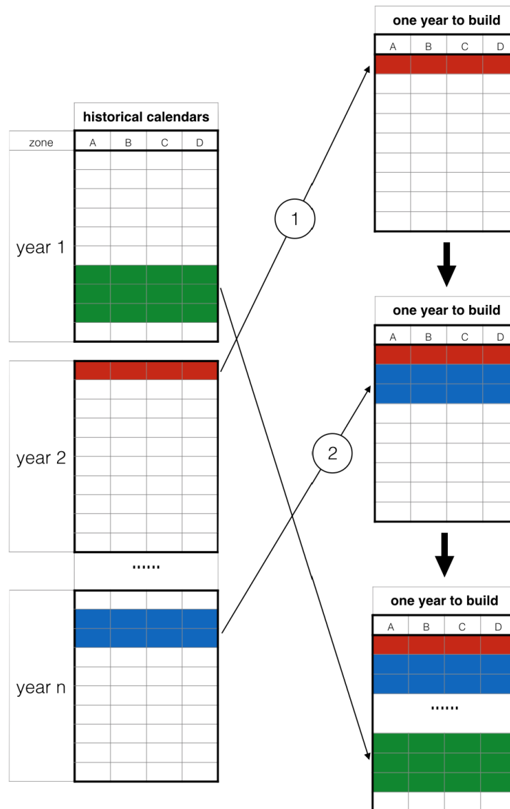
Figure 5.9: Diagram of resampling technique.
