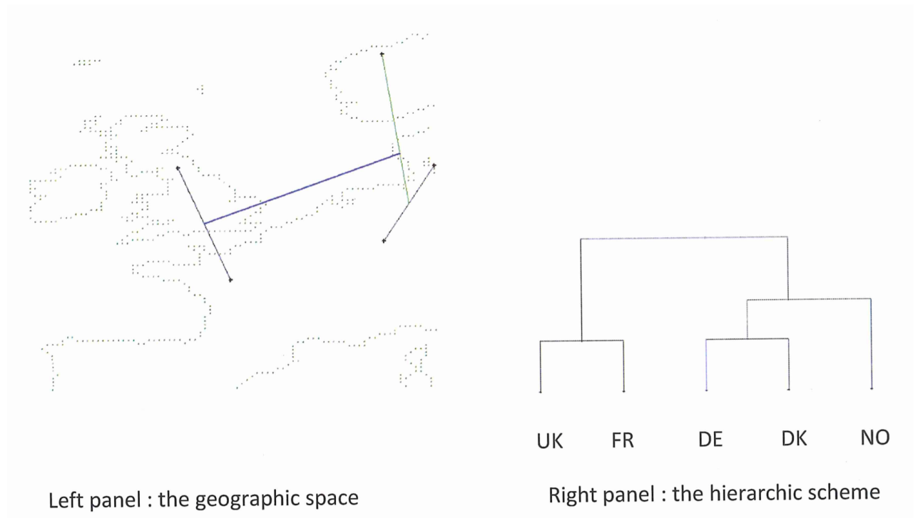
Figure 4.3: Coordinating atmospheric weather classes over five countries by means of Condorcet model. Source: [Leblois, 2014]
