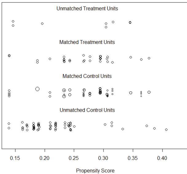
Distribution of Propensity Scores
