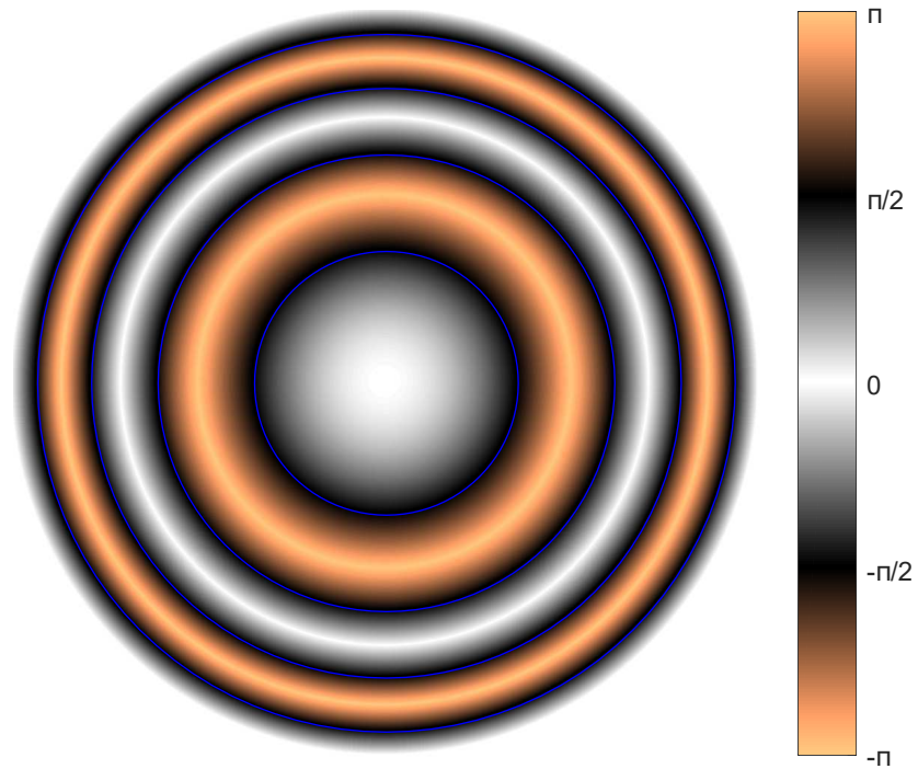
Figure 11.5: Phase distribution on the first four Fresnel zones. White and orange represent constructive and destructive interference, respectively.
