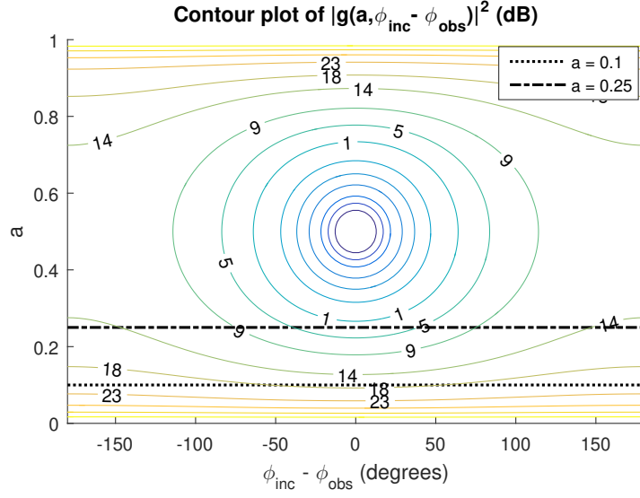
Figure 3.5: Contour plot of |g(a, \hat{\mathbf{r}}_{inc}, \hat{\mathbf{r}}_{scat})|^2 in dB.
