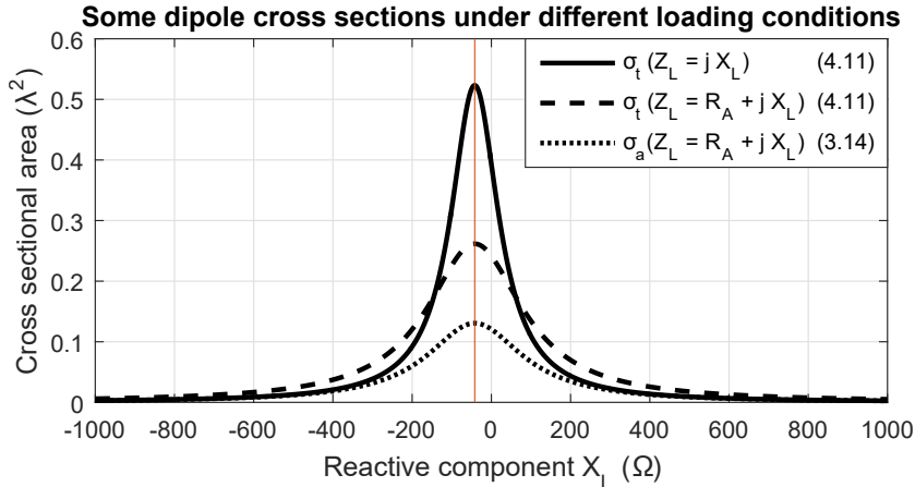
Figure 3.2: Total scattering and absorption cross sections of a dipole under different loading conditions versus the reactive component of Z_L .
