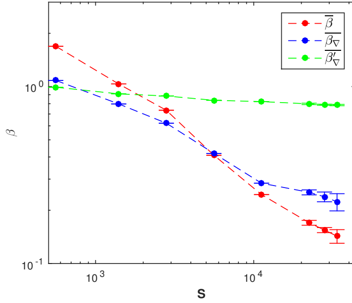
Figure 4.4: Importance of the pressure force on the dynamics as measured by \overline{\beta} , \overline{\beta}_{\nabla} and \overline{\beta}'_{\nabla} for different values of the Lundquist number.
