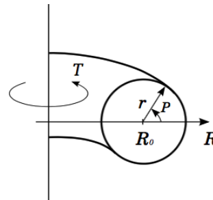
Figure 1.3: (Left) geometrical and electrical parameters of different tokamak devices, where R_0 is the major radius of the torus and r = a the minor radius of the poloidal cross-section, (right) schematic figure of the toroidal geometry.
