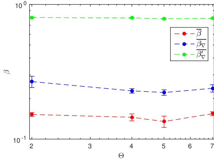
Figure 4.3: Importance of the pressure force on the dynamics as measured by \overline{\beta} , \overline{\beta}_{\nabla} and \overline{\beta}'_{\nabla} for different values of the pinch ratio with S = 2.8 \times 10^4 .
