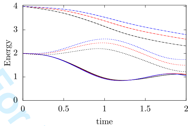
Figure 3. Orszag-Tang vortex problem at Re \approx 628 . Time evolution of the space-average kinetic (continuous lines), magnetic (dotted lines) and total (dashed-dotted lines) energies with Pr_m = 0.5 (black), 1 (red) and 2 (blue). The kinetic energy does not experience a large influence. Conversely, the magnetic energy increases with Pr_m due to the reduction of the magnetic diffusivity \eta .
