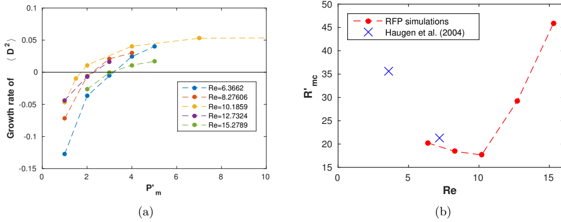
Figure 6.4: (a) Growth rate of \langle D^2 \rangle for different values of Re and P'_m , (b) critical magnetic Reynolds number R'_{mc} function of Reynolds number Re .
