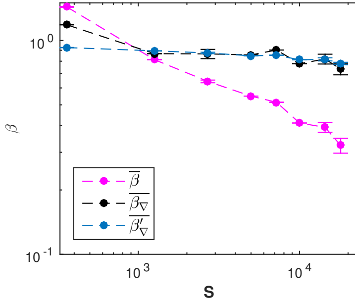
Figure 4.6: Importance of the pressure force on the dynamics of elliptical RFP with a = 1.2 b = 0.833 , as measured by \beta , \overline{\beta_\nabla} and \overline{\beta'_{\nabla}} for different values of the Lundquist number.
