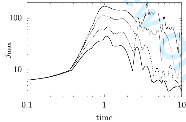
Figure 4. Orszag-Tang vortex problem. Hybrid LB simulation: Time evolution of the current maxima at Re = 500 (continuous line), 1000 (dashed), 2500 (dotted) and 5000 (dashed-dotted).
