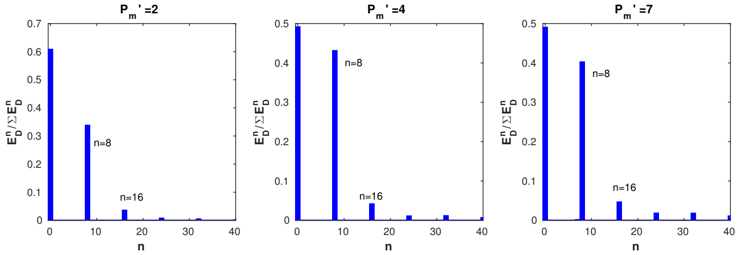
Figure 6.8: Axial spectra of D^2 for Re = 10.2 and different values of P'_m .
