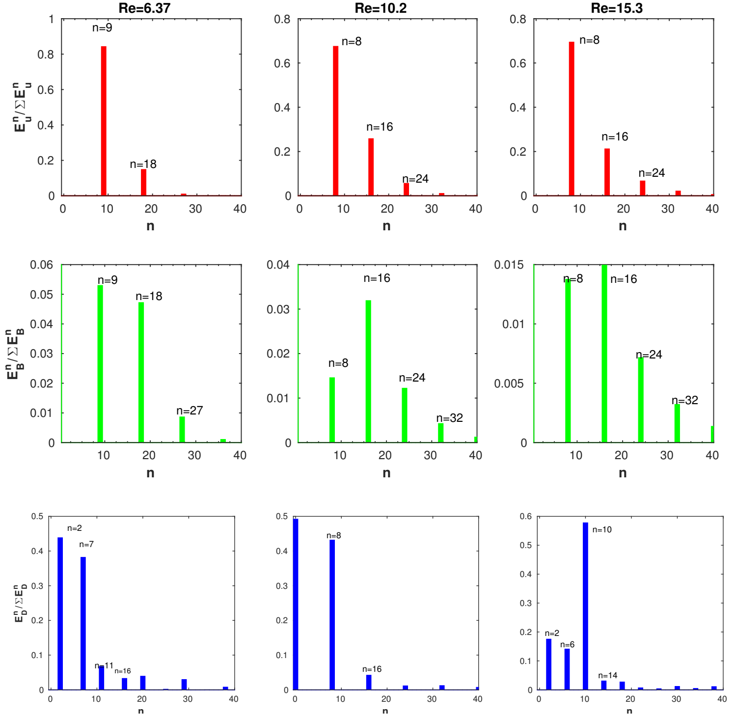
Figure 6.5: Axial spectra of u^2 (red), B^2 (green) and D^2 (blue) for different values of Re and for P'_m = 4 .
