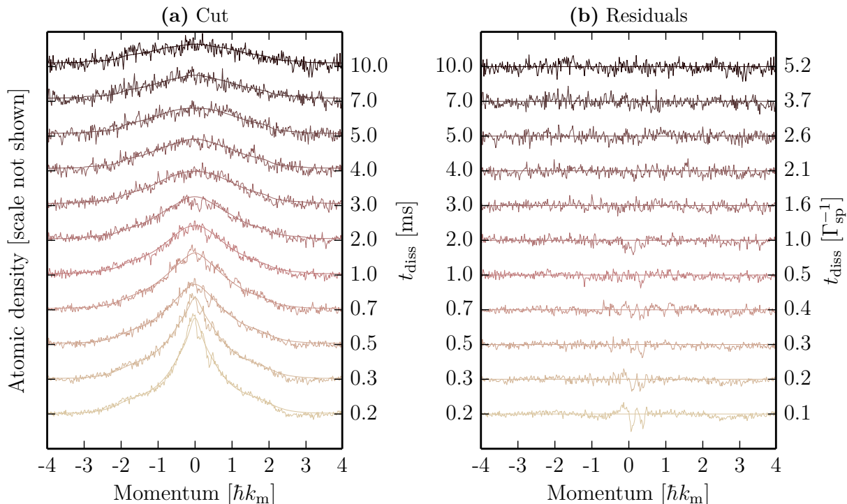
Figure 4.12: Momentum profile evolution with respect to dissipation pulse time in the algebraic regime of the decay with parameters V_{\perp} = 7.3 E_R and \Gamma_{\text{sp}} = 520 \text{ s}^{-1} . As indicated by the vertical scale in the middle, dissipation pulse time grows upwards. (a) Cuts along one axis of the optical lattice, smooth solid lines are fits. The atomic density scale is not shown for clarity: the corresponding peak optical density is \text{OD}_{\text{max}} \approx 0.1 for the bottom curve. (b) Residuals of the fit.
