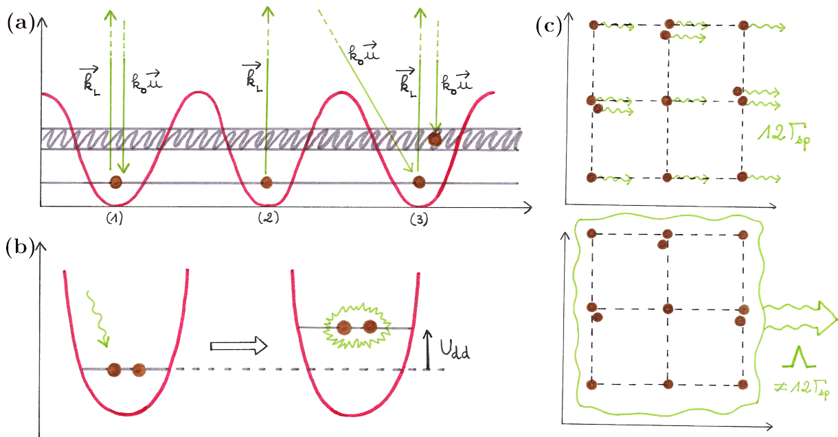
Figure 5.1: Pictorial description of various effects related to spontaneous emission in optical lattices. (a) The absorption of a laser photon (wavevector \mathbf{k}_L ) and its subsequent emission (wavevector k_0\mathbf{u} ) can either leave an atom in place (see site 1), transfer an atom to the next site (see site 2) or promote it to another band (see site 3). (b) The absorption of a photon on a site with two atoms leads to an energy shift U_{dd} associated to the exchange of this photon between the two atoms, also called induced dipole-dipole interaction. (c) Spontaneous emission for independent emitters (here 12 atoms contribute to a rate 12\Gamma_{sp} ) is sketched on the top. Collective emission with a rate \Lambda a priori different from 12\Gamma_{sp} is sketched on the bottom. Figure designed with Marion Bouganne.
