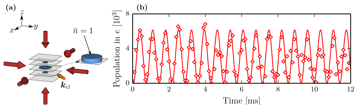
Figure 3.5: Single-particle Rabi oscillations. The coupling by the clock laser is turned on at time t = 0 . (a) Sketch of the experiment, the atomic sample is a MI phase with unit filling fraction ( N_{\text{at}} \approx 8 \times 10^3 ). (b) Coherent driving on the clock transition with Rabi frequency \Omega \approx 2\pi \times 1400 Hz and zero detuning, measuring the number of excited state atoms. We observe long-lived oscillations up to 10 ms before the contrast diminishes. The solid line is a sinusoidal fit to the data. Figure adapted from Bouganne et al. (2017).
