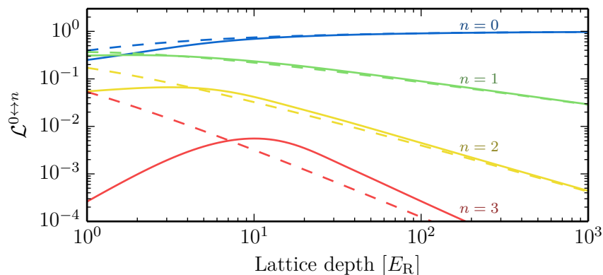
Figure 5.3: Lamb-Dicke factors \mathcal{L}^{0\leftrightarrow n} for a 1D sinusoidal potential (solid lines) calculated from (5.20), and \mathcal{L}_{\text{ho}}^{0\leftrightarrow n} for a harmonic oscillator potential (dashed line) calculated from (5.19).
