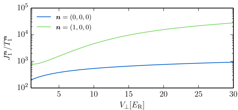
Figure 5.9: Comparison between coherent and light-induced tunnellings for various lattice depth V_{\perp} . The rate of spontaneous emission is \hbar\Gamma_{\text{sp}} = 0.1 E_R .
