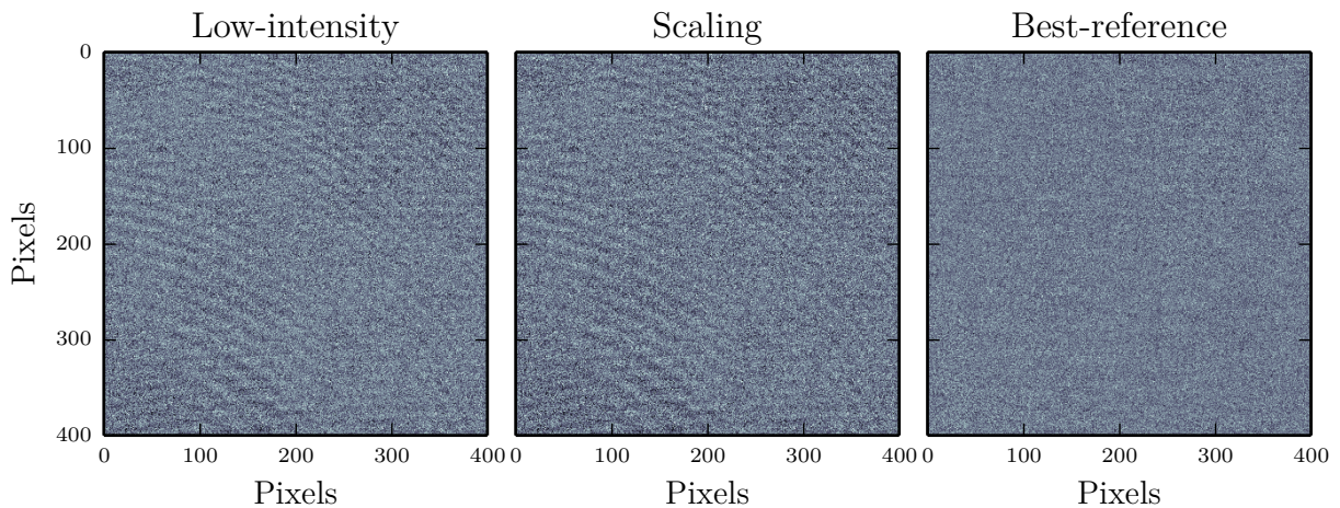
Figure A.1: Optical depths in the region of interest obtained from the different methods. It is clear that the fringes appearing in the low-intensity treatment cannot be removed using only a rescaling of the reference image. The best-reference picture provides a way to do so.
