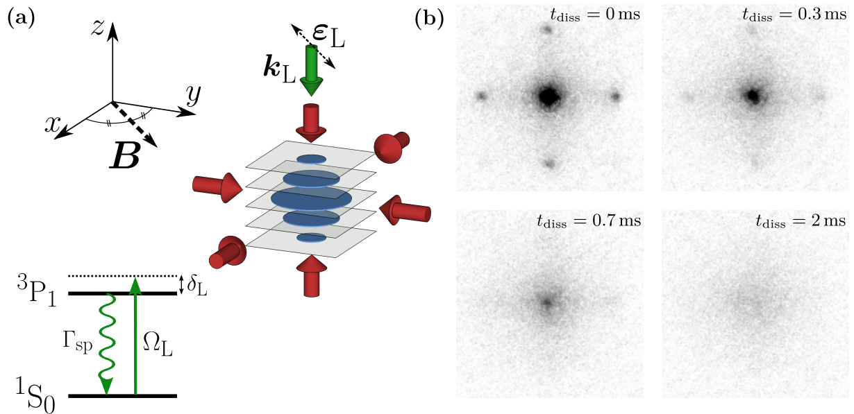
Figure 4.1: Dissipation in a superfluid. (a) Sketch of the experiment and of the level scheme of the intercombination transition. The red arrows denote optical lattice beams, the green arrow denotes the dissipation laser beam with wavevector \mathbf{k}_L propagating vertically with a polarisation \boldsymbol{\epsilon}_L parallel to the applied magnetic field \mathbf{B} along the x+y direction. The dissipation laser drives the intercombination transition with Rabi frequency \Omega_L , detuning \delta_L and spontaneous emission rate \Gamma_{sp} . (b) Absorption images taken after 20 ms expansion for various dissipation times t_{diss} , the line of sight is vertical. In this experiment the parameters are V_{\perp} = 8.8 E_R , \Gamma_{sp} = 250 \text{ s}^{-1} , \delta_L = +15\Gamma_g and \Omega_L = 2\pi \times 81 \text{ kHz} .
