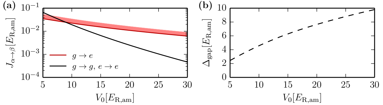
Figure 1.14: (a) Comparison between laser-induced tunnelling J_{g \rightarrow e} and natural tunnelling J_{g \rightarrow g} and J_{e \rightarrow e} for a typical Rabi frequency \Omega_{cl} = 2\pi \times 1 kHz. The red shaded area represents the possible values taken by J_{g \rightarrow e} when varying the flux \chi/(2\pi) from 0 to 1/2 . (b) Band gap \Delta_{\text{gap}} between the fundamental and the first excited band of the lattice.
