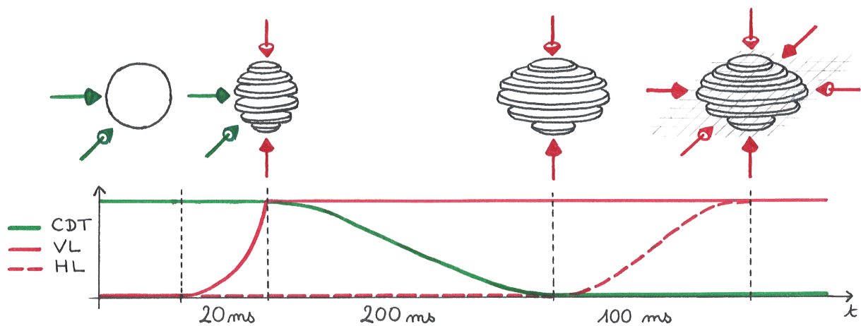
Figure 2.9: Time sequence for loading the optical lattices. A deep vertical lattice is first ramped-up in 20 ms. Then the crossed dipole trap is smoothly extinguished in 200 ms to let atoms redistribute in the planes. Finally, horizontal lattices are adiabatically turned on in 100 ms. Figure designed with Marion Bouganne.
