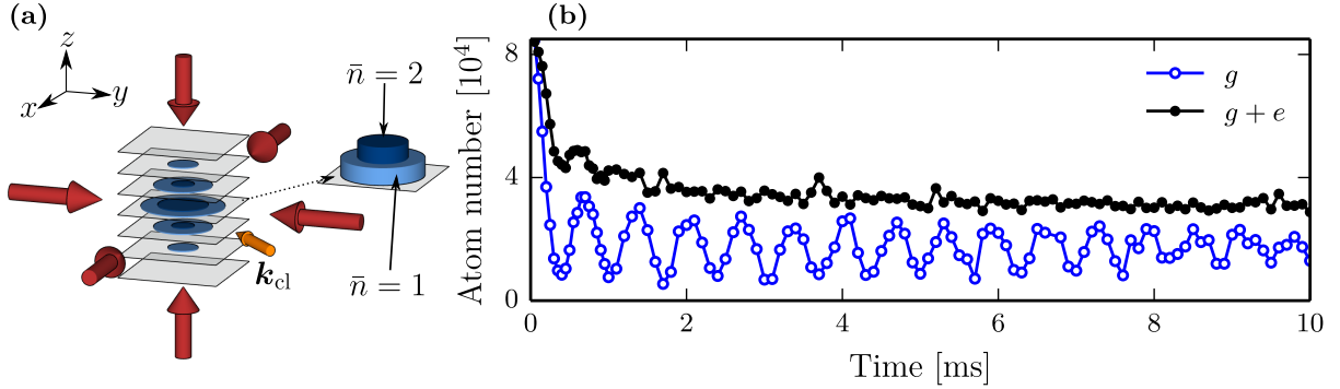
Figure 3.6: Rabi oscillations for high atom number. The driving by the clock laser is turned on at time t = 0 . (a) Sketch of the experiment, the atomic sample consists of MI phases with filling fractions of one and two ( N_{\text{at}} \approx 8 \times 10^4 ). (b) Coherent driving on the clock transition with Rabi frequency \Omega \approx 2\pi \times 1450 Hz and zero detuning. Closed (respectively open) symbols represent the remaining total atom number (resp. the population in the ground state g ). We observe an initial decay at early times followed by long-lived oscillations. Figure adapted from Bouganne et al. (2017) .
