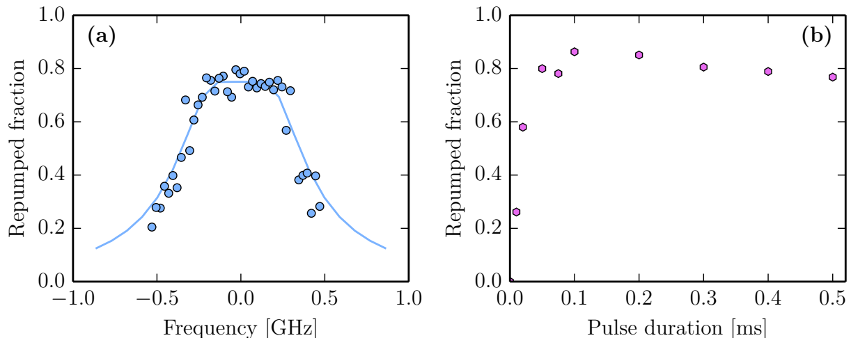
Figure 2.7: Characterisation of the repumping laser. (a) Spectrum of the repumping transition with 500 \mu\text{s} -long pulses, the solid line is a calculation using optical Bloch equations for the 5-level system shown in Figure 2.6. (b) Efficiency of the repumping versus pulse duration.
