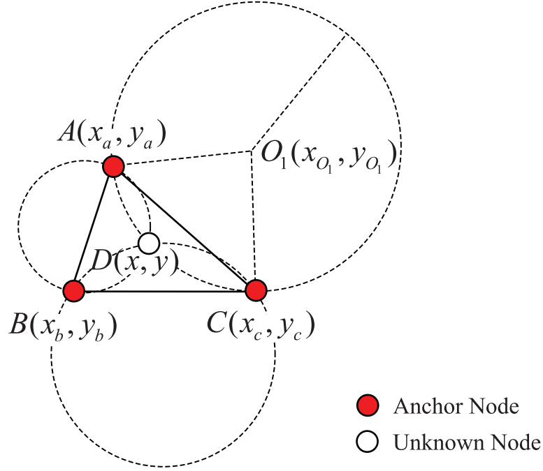
Figure 2.8: An example of the triangulation algorithm [56].
