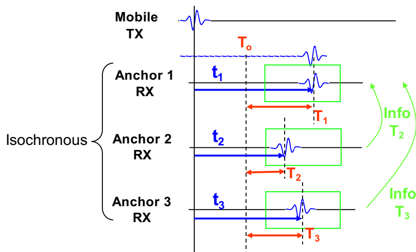
Figure 2.3: The diagram of the TDOA technique.
