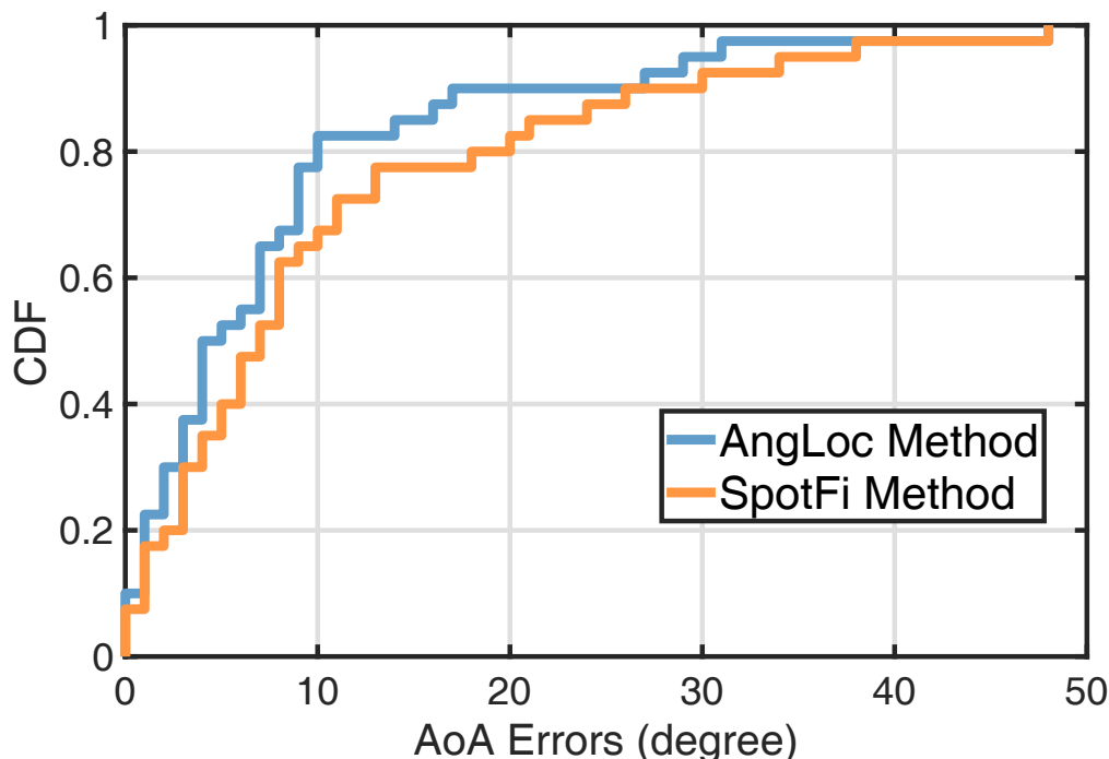
Figure 4.17: AoA estimation errors in LoS condition.
