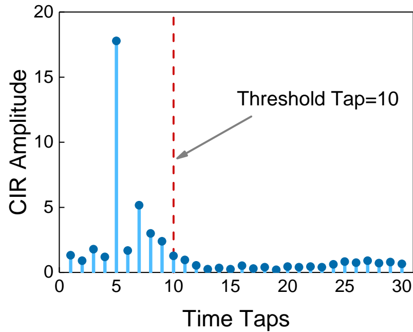
Figure 3.2: Channel impulse response.
