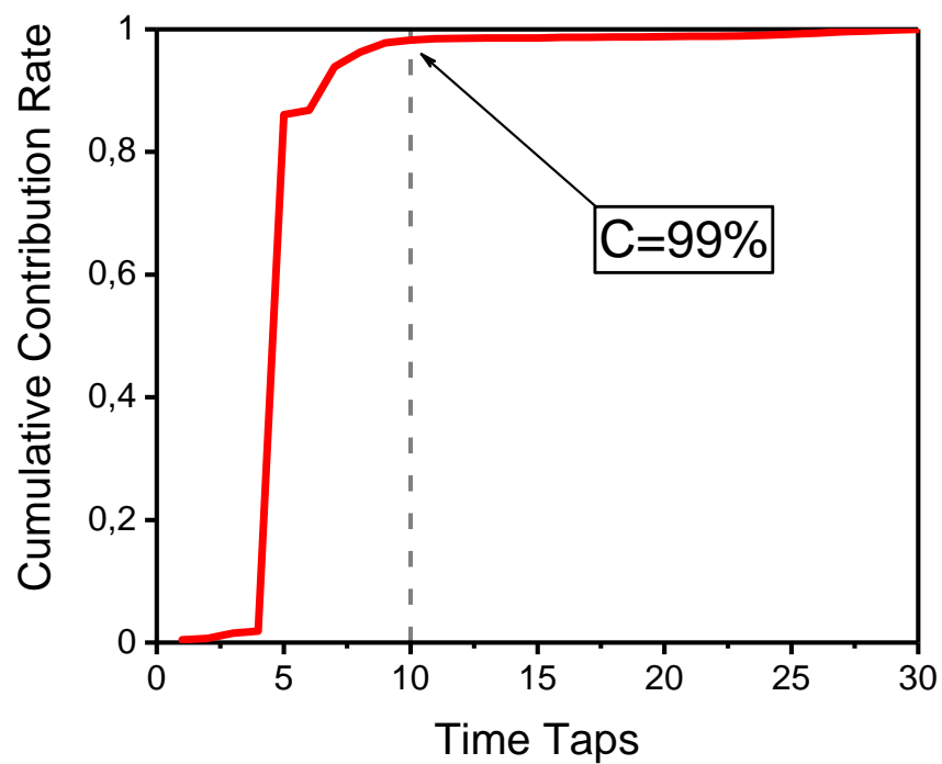
Figure 3.3: Power threshold.
