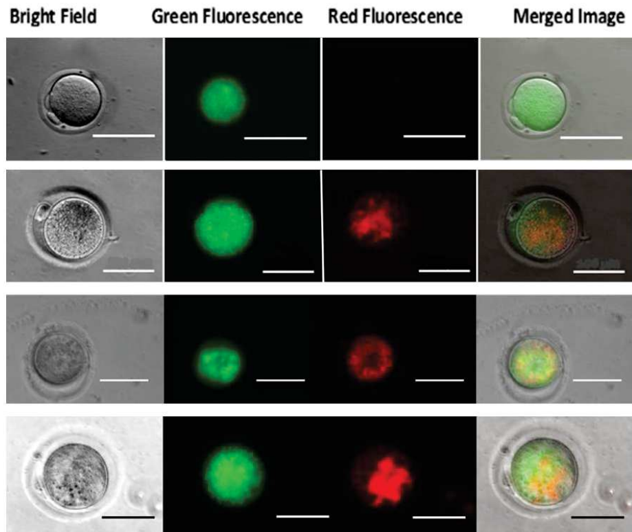
Figure 4. Artificial Mitochondrial Transfer by MitoCeption after IVF to murine zygotes. Mature oocytes were fertilized, stained with CytoTracker Green, and immediately after MitoCepted with HPMM isolated from PBMCs labelled with MitoTracker Red. Micrographs were taken after 1h culture of the MitoCepted zygotes. Columns: first, bright field; second, green fluorescence micrograph; third, red fluorescence micrograph; fourth, merged of bright field and fluorescence in green and red. a. Control zygote without exogenous mitochondria b. Zygote with 12.5 ng / \mu\text{L} of HPMM c. Zygote with 25 ng / \mu\text{L} of HPMM. d. Zygote with 50 ng / \mu\text{L} of HPMM. Scale bar 100 \mu\text{m}
