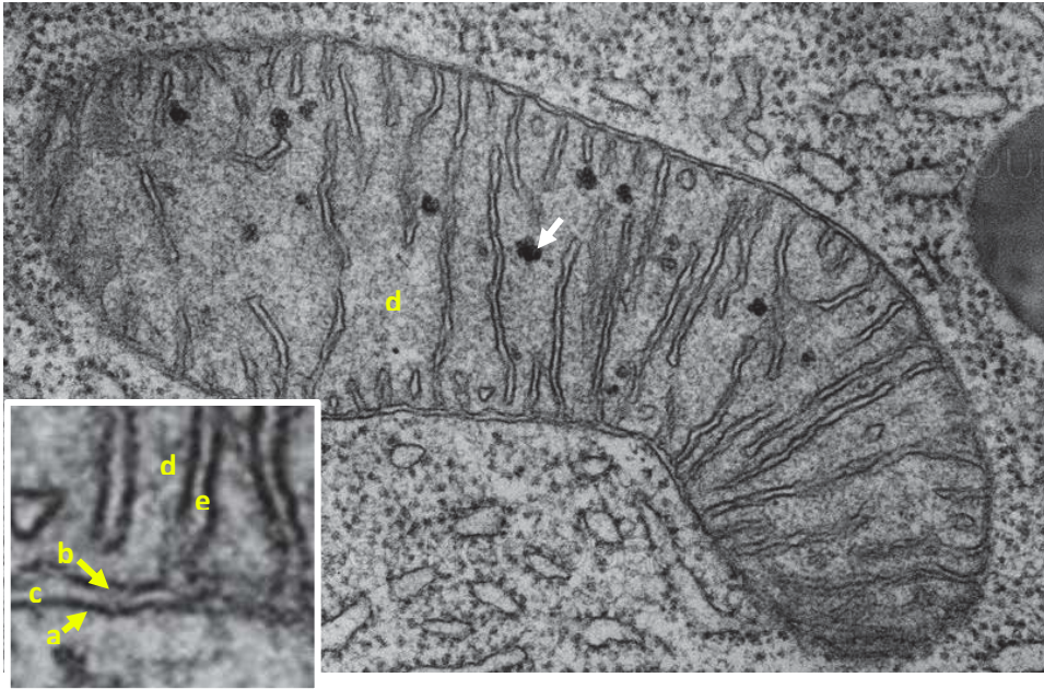
Fig. 4 Mitochondrion in Bat Pancreas Cell. a. Outer Mitochondrial Membrane, b. Inner Mitochondrial Membrane, c. Intermembrane space, d. Mitochondrial Matrix, e. Cristae, White Arrow: calcium granule. Inset: amplification of OMM and IMM. TEM micrography modified from (Science Source, n.d.)
