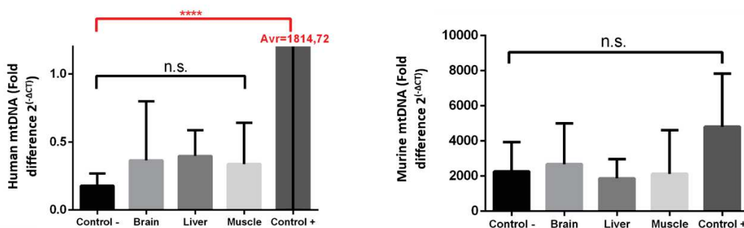
Figure xx: Detection of murine and human mitochondrial genes in mitocepted murine newborns calculated by Delta CT method at 25 ng/ \mu\text{L} of mitochondrial protein in three tissues: Brain, liver and muscle and using mitocepted morulae genomic DNA as positive control. a. expression
