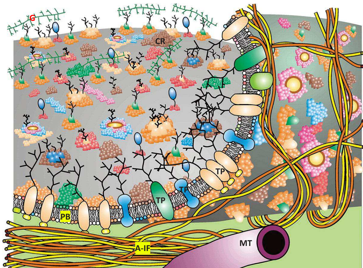
Figure 2. General Components of Plasma Membrane: G. Glycocalyx, CR. Cholesterol Raft, TP. Transmembrane proteins, PB. Phospholipidic Bilayer, MT. Microtubule (cytoplasmic component), A-IF Actin and Intermediate Filaments (cytoplasmic component). Transmembrane proteins in pink represent receptors or carriers with enzymatic intracellular domains (as ATPase-dependant Na-K pump) (Modified from (Jacobson et al., 2019)).
