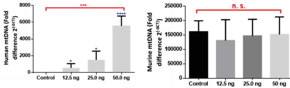
Figure 3: Detection of human and murine mitochondrial genes in mitocepted murine oocytes calculated by 2^{(-\Delta CT)} method at 3 dosages: 12.5, 25 and 50 ng/ \mu l of mitochondrial protein. Housekeeper gene: Murine B 2 M (MB 2 M). a: Human Mito (HMito) b: Murine Mito (MMito)
