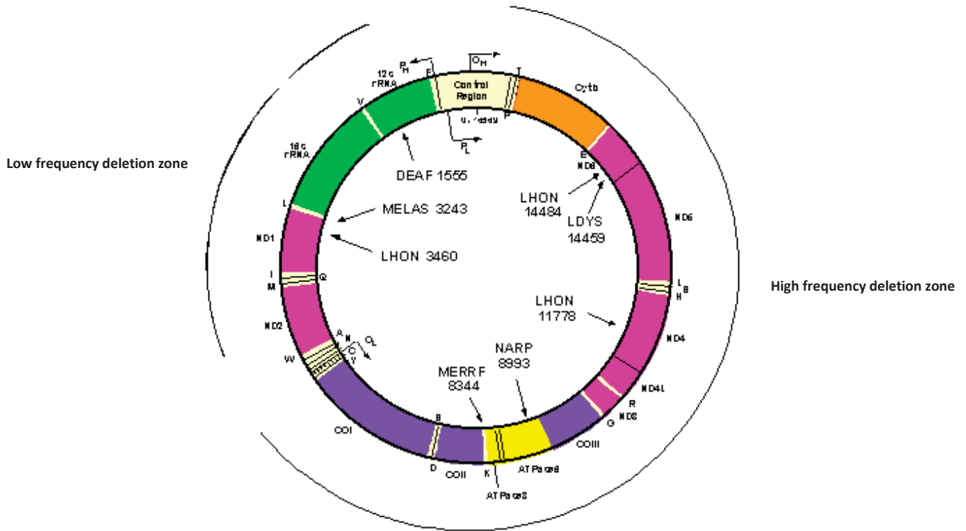
Figure 5: Map of Human Mitochondrial DNA and main mutations and deletions causing inherited mitochondrial diseases. Descriptions in the text (“WebHome < MITOMAP < Foswiki,” n.d.)
