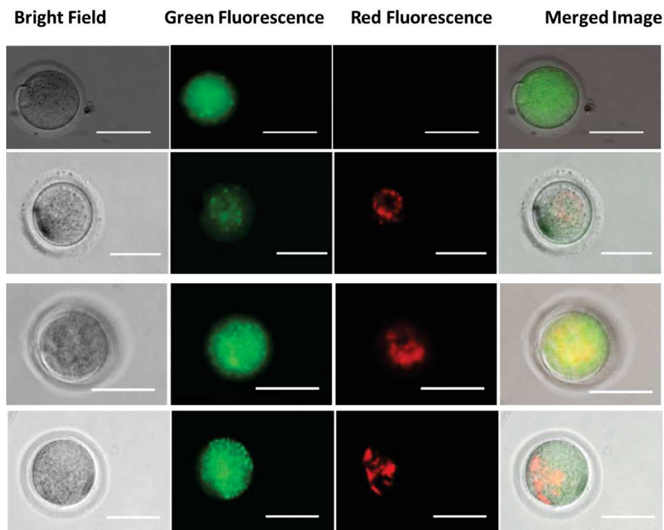
Figure 2. Artificial Mitochondrial Transfer by MitoCeption to murine Oocytes. Mature oocytes were stained with CytoTracker Green; HPMM isolated from PBMCs was marked with MitoTracker Red. MitoCeption of oocytes with HPMM was performed after isolation of the oocytes and washing. Micrographs were taken after 1h culture of the MitoCepted oocytes. Columns: first, bright field; second, green fluorescence micrograph; third, red fluorescence micrograph; fourth, merged of bright field and fluorescence in green and red. a. Control oocyte without exogenous mitochondria b. Oocyte with 12.5 ng / \mu\text{L} of HPMM c. Oocyte with 25 ng / \mu\text{L} of HPMM. d. Oocyte with 50 ng / \mu\text{L} of HPMM. Scale bar 100 \mu\text{m}
