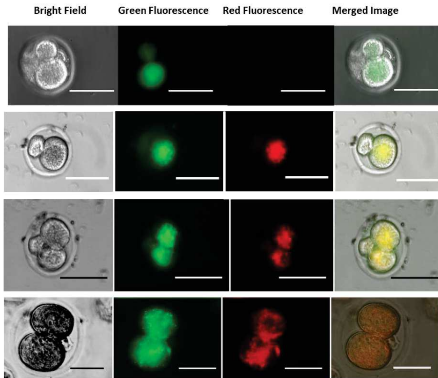
Figure 3. 2-cell development of Mitocepted embryos with HPMM. Green zygotes after MitoCeption with HPMM (in red) were maintained in culture during 6h (2-cell embryos) and micrographs were performed to follow up its development and survival. Columns: first, bright field; second, green fluorescence micrograph; third, red fluorescence micrograph; fourth, merged of bright field and fluorescence in green and red. a. Control 2-cell embryos without exogenous mitochondria b. 2-cell embryos with 12.5 ng / \mu L of HPMM c. 2-cell embryos with 25 ng / \mu L of HPMM. d. 2-cell embryos with 50 ng / \mu L of HPMM. Scale bar 100 \mu m
