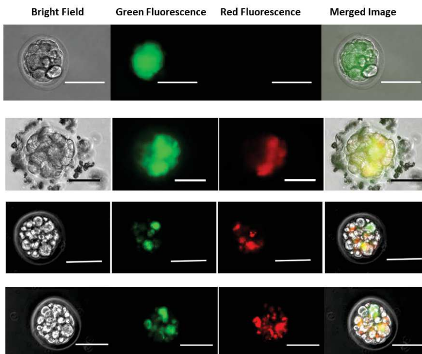
Figure 4. Morula development of Mitocepted embryos with HPMM. Green zygotes after MitoCeption with HPMM (in red) were maintained in culture during 10h (Morula stage) and
