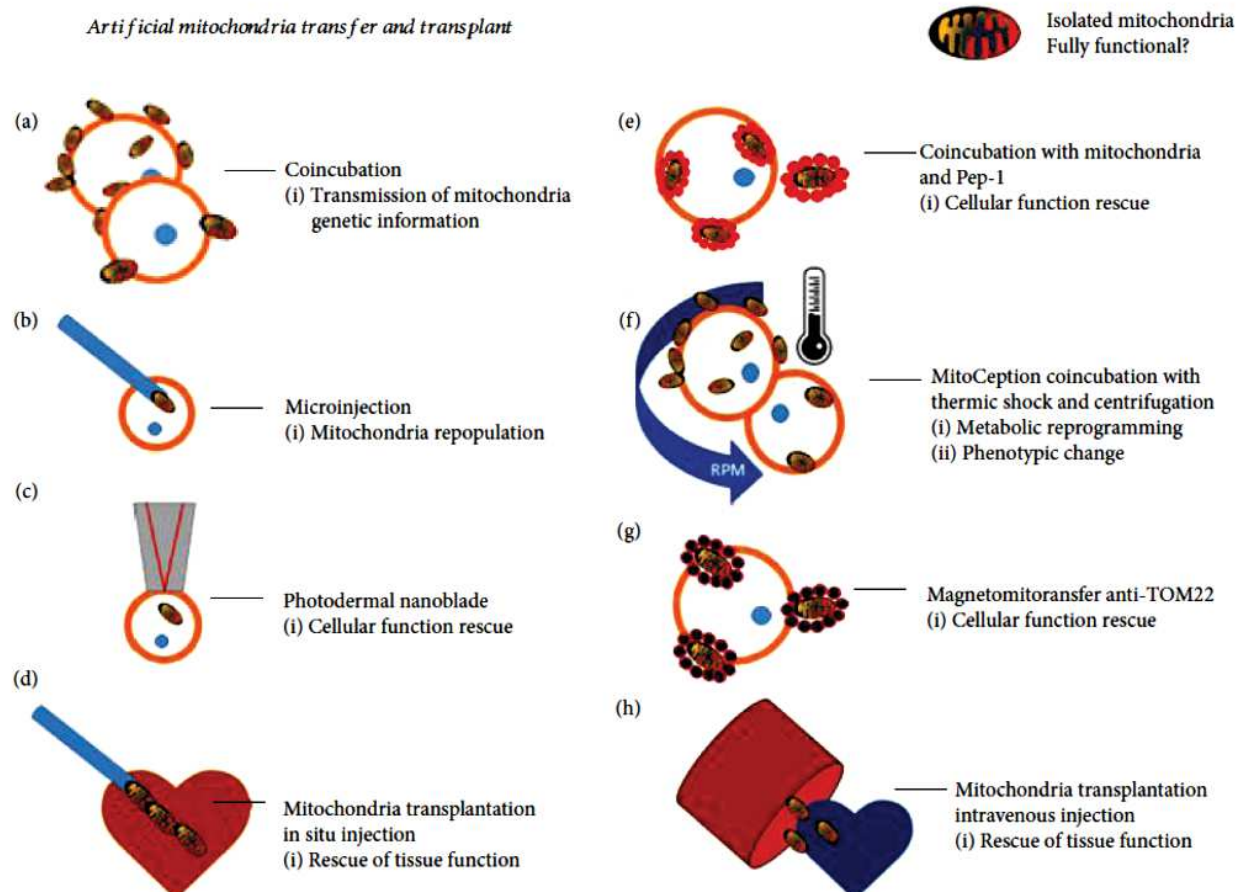
FIGURE 2: Artificial mitochondria transfer (AMT) and transplant. Different techniques emerged to mimic the natural transfer or mitochondria on its in vivo and in vitro applications. The coincubation technique was the first proposed in which the antibiotic resistance carried in the mitochondrial DNA was passed to sensitive cells [9], later after the technique was used to rescue respiratory deficient cells among other damaged cells [10, 11, 14, 63]. Microinjection of exogenous mitochondria was applied in assays to eliminate the endogenous copies of oocytes carrying mitochondrial diseases [90, 93]. The photothermal nanoblade effectively transferred isolated mitochondria inside the cell; even if they showed great effectiveness, its application is limited to small cell numbers [12]. Two different approaches were developed to facilitate the mitochondria internalization in the recipient cells, the first is by using Pep-1 and the other with magnetic beads (Magnetomitortransfer) designed to bind to TOM22 a receptor complex in the mitochondrial membrane. The MitoCeption technique uses a thermal shock and a centrifugation to improve the process of mitochondria uptake; first applied in cancer cells, this technique induces the metabolic reprogramming of these cells. The in vivo application of the mitochondria transfer applies two approaches: the first is to directly inject mitochondria to the harmed tissue and the other in the circulatory system close to the area of interest. Both of them have shown to restore tissue function but the in situ injection showed better results [16, 49, 50].
