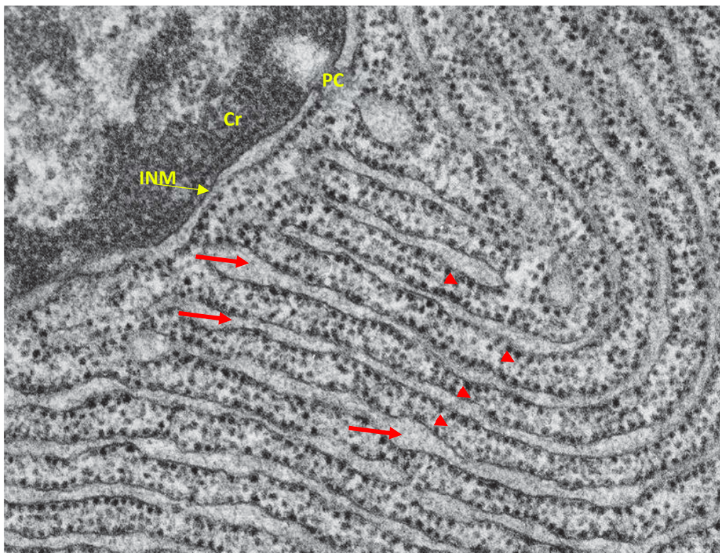
Figure 3. Nucleus and Rough Endoplasmic Reticulum. Cr, cromatin. PC, pore complex. INM, internal nuclear membrane. Red Arrows, ER cisternae. Arrows' heads, ribosomes. Modified from: (Schekman, 2004)
