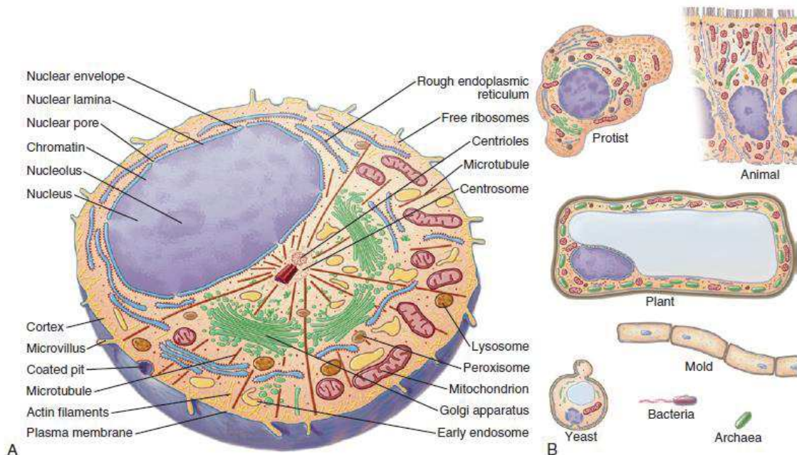
Figure 1. Basic Cellular Architecture. A , Section of a eukaryotic cell showing its internal and general components: Structures as cell wall and chloroplast are exclusive of plants, while cilia and flagella are exclusive of protist and animal cells. B , Comparison of cells from the mayor branches of the phylogenetic tree (Pollard et al., 2017).
