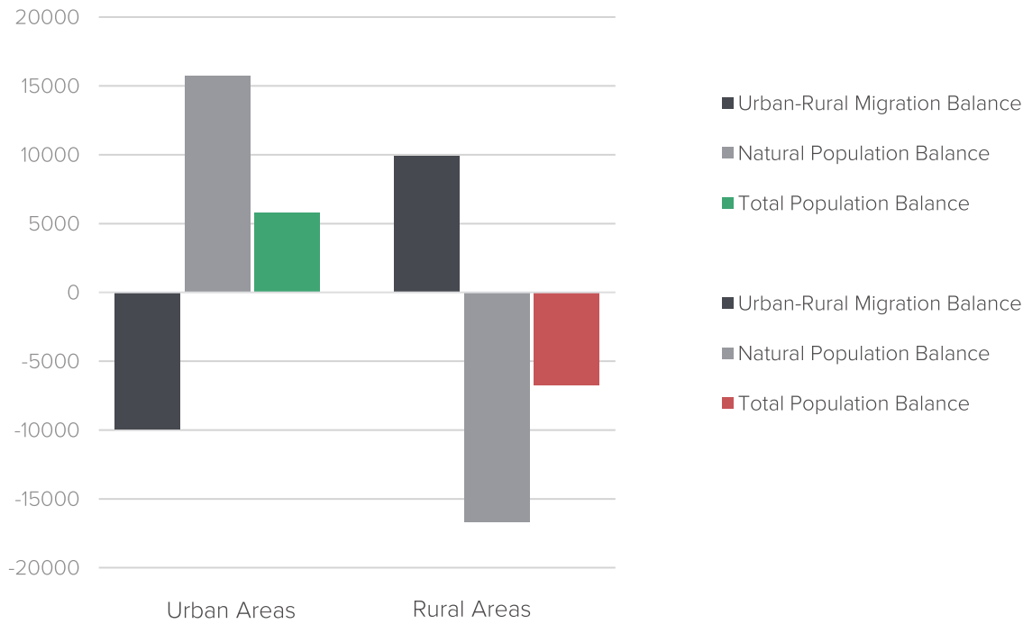
Chart 7.1 Population Balance for Urban and Rural Areas, 2000-2001
