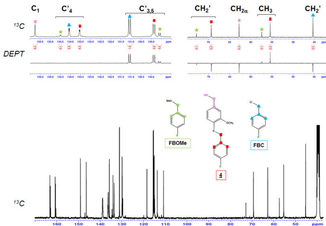
Figure 4.6. ^{13}\text{C} -NMR spectra of the mixture issued from the fluorobenylation of Vanillyl alcohol ( 4 ) in DMSO- d_6 .
