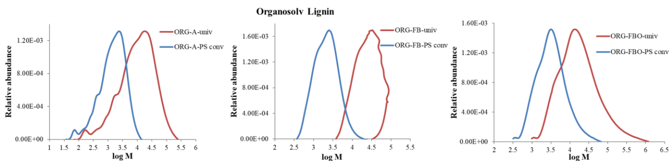
Figure 5.16. Comparison of universal and conventional SEC – MMD curves of relative abundance vs \log(M) for A - acetylated, FB - fluorobenzylated and FBO - fluorobenzoylated ORG lignin samples
