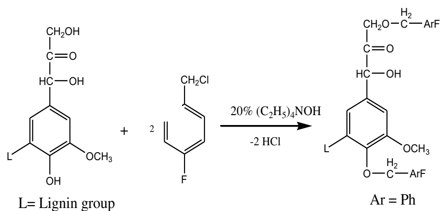
Figure 2.5. Fluorobenzoylation of lignin using 4-benzylchloride
