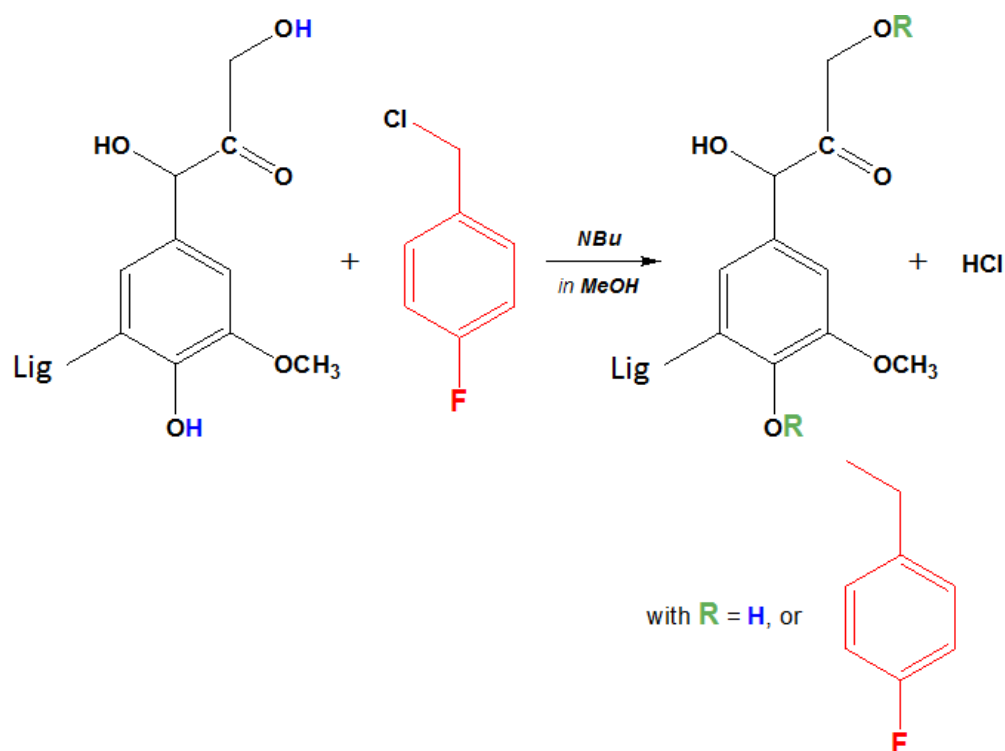
Figure 4.4. Fluorobenzylation reaction of lignin
