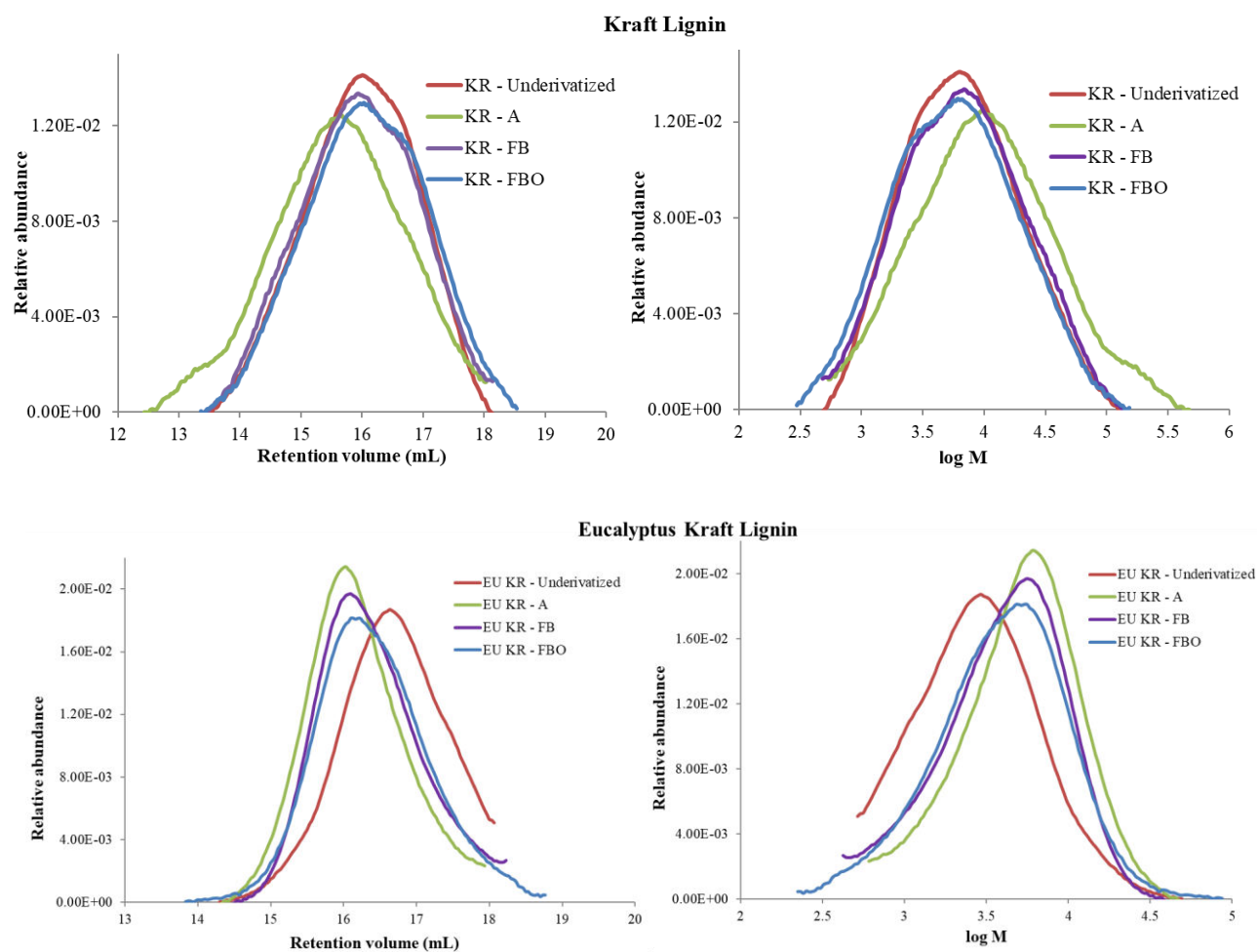
Figure 5.10. SEC chromatogram profiles of underivatized and derivatized (acetylated, fluorobenzylated and fluorobenzoylet) of all studied lignin samples. Relative abundance vs Retention volume ( left ) and Relative abundance vs log (M) ( right )
