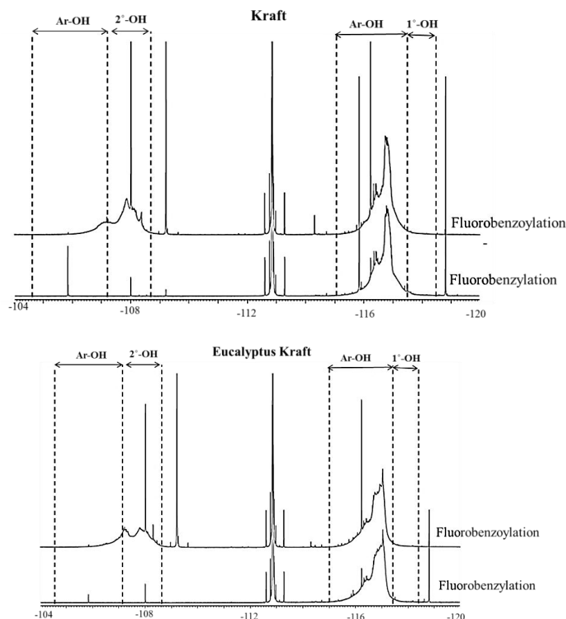
Figure 5.9. ^{19}\text{F} NMR spectra of fluorobenzylated and fluorobenzoylelated Protobind, Organosolv, Indulin, Kraft and Eucalyptus-Kraft lignins. Chemical shifts relative to \text{CFCl}_3 . Internal standard: 2-fluoroacetophenone
