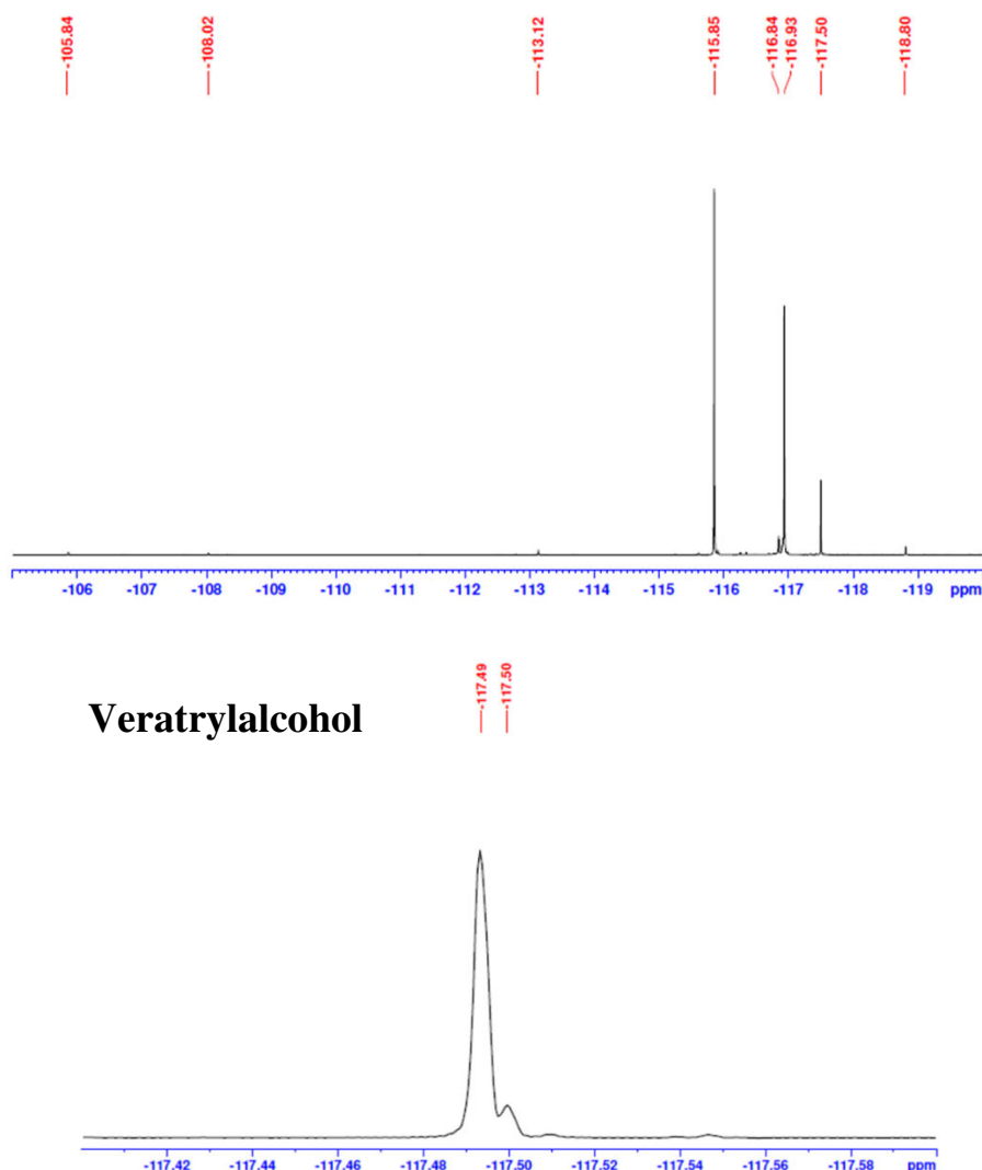
Figure 4.8. ^{19}\text{F} -NMR spectra of fluoroderivatized model compounds. From top to bottom: Vanillin, Acetovanillone, Guaiacol, Vanillyl alcohol and Veratryl alcohol.
