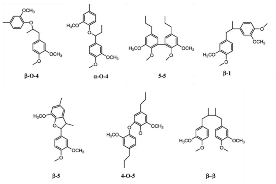
Figure 1.11. The most common unit linkages in lignin (Chakar and Ragauskas, 2004)
