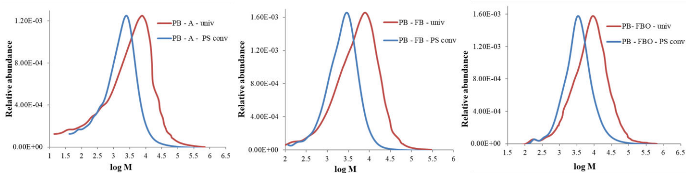
Figure 5.12. Comparison of universal and conventional SEC – MMD curves of relative abundance Vs \log(M_w) for A - acetylated, FB - fluorobenzylated and FBO - fluorobenzoylated PB lignin samples
