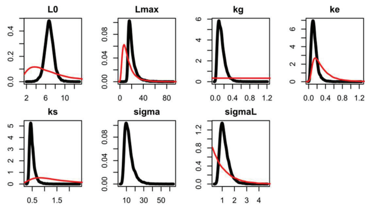
Figure S3. Prior (red curve) and posterior (black curve) marginal distributions of model parameters for chironomids (Eq. 6).
