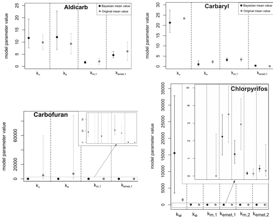
FIGURE S3 – Model parameters estimated by Bayesian inference (black) and in the original study (grey). Dots represent mean values and error bars the 95% credibility (Bayesian inference) or confidence (original studies) intervals.
