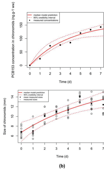
Figure S4. For the chironomid model (Eq. (4)), (a) prior (red curve) and posterior (black curve) marginal distributions, (b) measured (points) and predicted (solid and dashed curves) (top) PCB 153 concentrations (ng g -1 ww) in chironomids during the accumulation phase from day 0 to 7, and length of chironomids (mm) (bottom).
