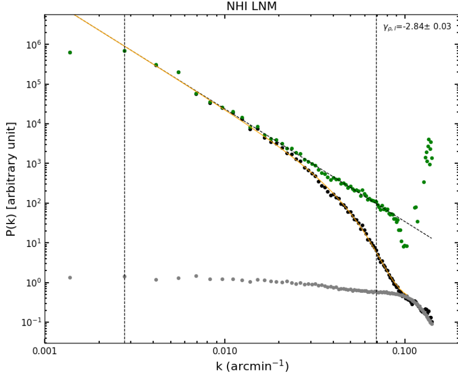
Fig. A.3.: Spatial power spectrum model of the integrated column density field of the LNM in NEP. \langle P_{N_{HI,1}} \rangle(k) is given by the black dots. Grey points represent the noise component N(k) . Green point show the corrected power spectrum (P(k) - N(k)/B(k)) . The dotted line shows the fit of the corrected power spectrum between the two vertical dashed line, and the orange line shows the result of the global modeling of Eq. A.1. The power spectrum index is \gamma_{\rho_l} = -2.84 \pm 0.03 .
