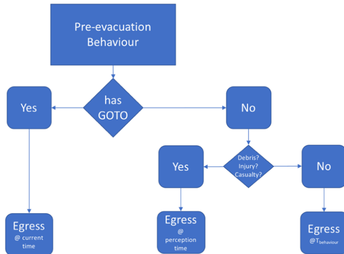
Figure 32 Model for building egress
