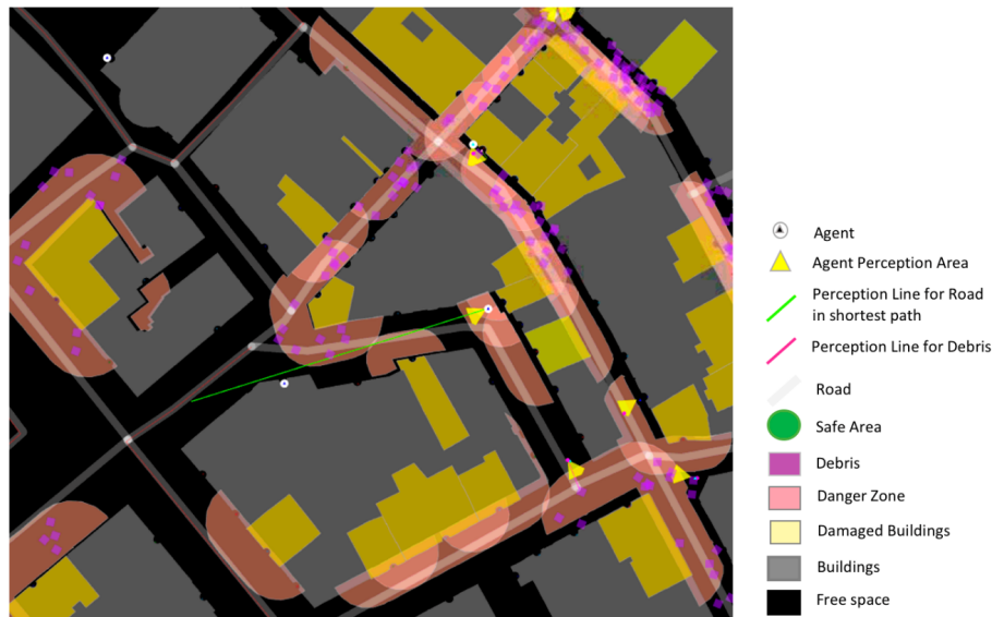
Figure 68 Agent navigation around blocked pathways. The agent with the long and green perception line has perceived a road segment which is part of the shortest route (white with thin red centreline). In its current location, the agent is able to travel freely in space as it navigates towards the portion of the shortest path towards safe zones. Buildings without damage are shown as grey polygons. Damaged buildings are yellow-orange polygons. Debris blocking roadways are shown as violet squares. Red polygons surrounding damaged buildings are danger zone.
