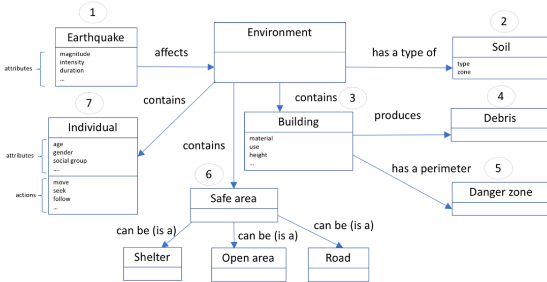
Figure 31 SOLACE simplified UML Class diagram
