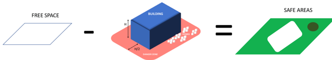
Figure 29 SOLACE Safe Areas extracted by the subtracting building footprint and danger zone from free space
