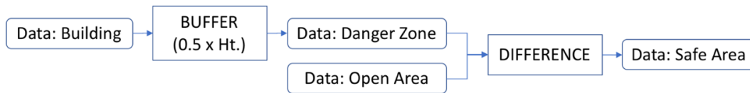
Figure 36 Geoprocessing workflow for the creation of danger zones and safe areas
