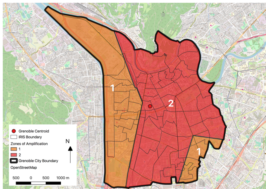
Figure 14 Grenoble zone amplification increments, zone boundaries are estimated and digitized based on a figure from Dunand & Guéguen, 2012. Map by Julius Bañgate, 2019.
