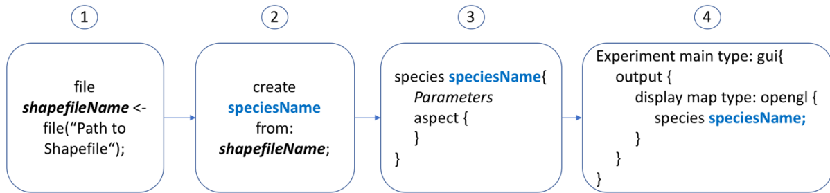
Figure 50 Creating non-human agents from shapefiles
