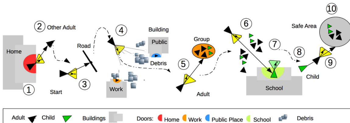
Figure 24 Example of agent movement in SOLACE model
