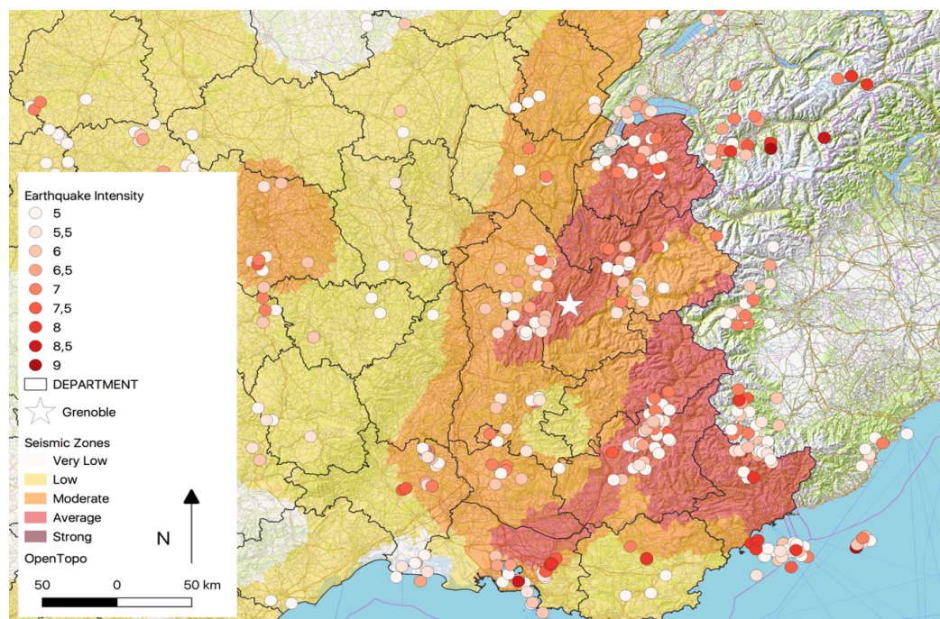
Figure 13 Location of historical earthquakes in the nearby region. Earthquakes have intensities greater than 5 around Grenoble. Earthquake data from www.sisfrance.net ( www.sisfrance.net , 2018). Map by Julius Bañgate, 2019 with data on Seismic zones and boundaries from planseisme.fr ( www.planseisme.fr , 2018). Topographic data from OpenTopo ( OpenTopography , 2018)
