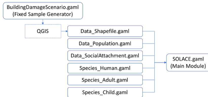
Figure 43 SOLACE Code Modules
