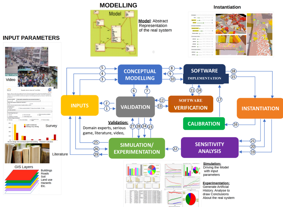
Figure 8 Detailed methodology carried out to develop a simulation of earthquake crisis
