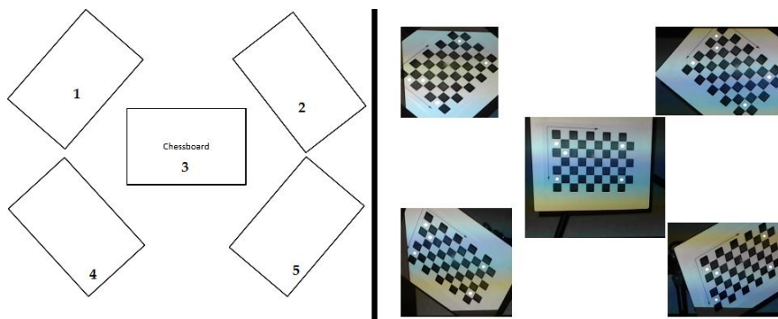
Figure 18. Projector intrinsic calibration- First Step
