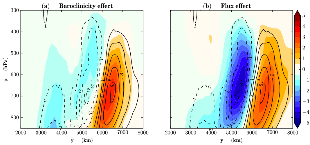
737 FIG. 11. Decomposition of the EDDY-CTRL difference between the contribution to baroclinic conversion of 738 (a) change of Eady growth rate a constant heat flux and (b) change of heat flux at constant Eady growth rate. 739 Contours represent the total baroclinic conversion in the 2-10 days band. All terms are in \text{m}^2 \text{s}^{-2} \text{day}^{-1} .
