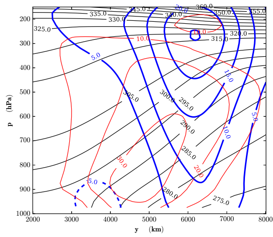
652 FIG. 2. Temporal and zonal averages of zonal wind (blue thick contours, in \text{m s}^{-1} ), potential temperature 653 (black contours, in K), and meridional flux of potential temperature (red thick contours, in \text{K m s}^{-1} ).
