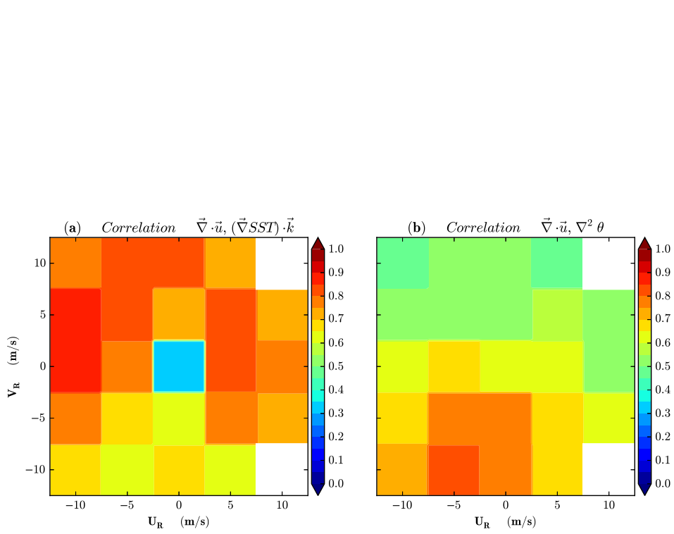
662 FIG. 7. Correlation coefficient of surface wind divergence with (a) downwind SST gradient and (b) Laplacian 663 of atmospheric boundary layer temperature, as a function of the large-scale background wind at 10 meters. 664 White squares denote insufficient number of snapshots for averaging over wind conditions.
