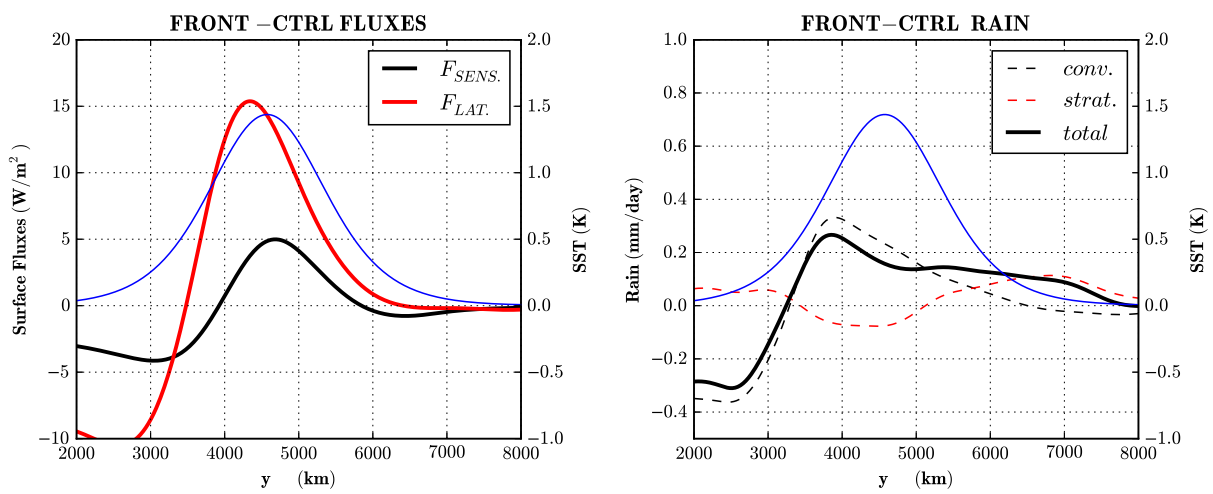
740 FIG. 12. Same as Figs. 4c-d, but for FRONT - CTRL. The blue curve shows difference of SST as a function 741 of latitude (in K).
