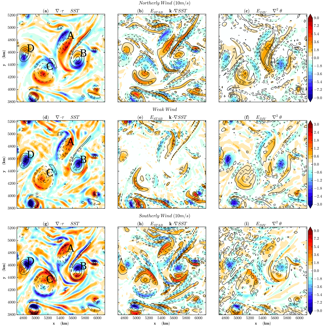
669 FIG. 9. Composites of wind-stress divergence \nabla \cdot \tau (a, d, g), stability effect on wind-stress divergence E_{stab} 670 (b, e, h) and wind divergence effect on wind-stress divergence E_{div} (c, f, i). Units are in 10^{-7} \text{ N m}^{-3} . Contours 671 in (a, d, g) correspond to SST_{eddy} (in K). Contours in (b, e, h) correspond to [\mathbf{U}_{10m}] \cdot \nabla SST (in 10^{-5} \text{ K m s}^{-1} ). 672 Contours in (c, f, i) correspond to [\nabla^2 \theta] (in 10^{-10} \text{ K m}^{-2} ). (a, b, c) strong northerly winds; (d, e, f) weak winds, 673 (g, h, i) strong southerly winds. Only anomalies computed with a Gaussian filtered are shown.
