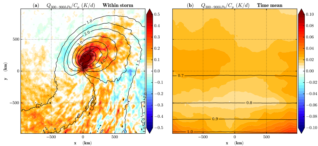
729 FIG. 9. (a) Contours: composites of diabatic heating (vertically averaged between 900 hPa and 300 hPa) 730 for low-pressure systems. (b) Same quantity but using time-mean diabatic heating instead of instantaneous 731 one. Shadings in (a, b): same quantities for the EDDY - CTRL EDDY difference. All terms are in K day^{-1} . 732 Low-pressure systems are defined as SLP minima with deviation from the zonal mean lower than -20 hPa, 733 considering only minima located in the band of latitude between 5000 km to 6000 km. Axes correspond to 734 distances from the SLP minimum.
