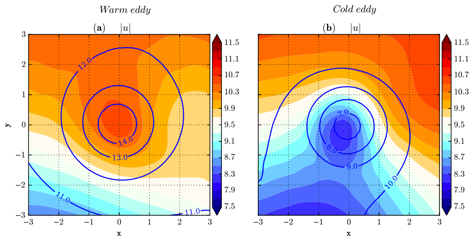
654 FIG. 3. Composites of surface wind speed \langle |\mathbf{U}_{10m}| \rangle (shading, in \text{m s}^{-1} ) and sea surface temperature \langle SST \rangle 655 (contours, in K), for (a) warm and (b) cold eddies.
