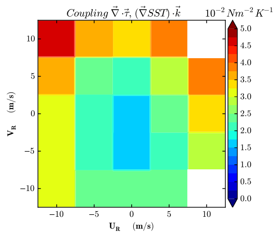
674 FIG. 10. Regression coefficient of wind stress divergence and downwind SST gradient anomalies as a function 675 of the large-scale background wind at 10 meters, in 10^{-2} N/m^2/K .
