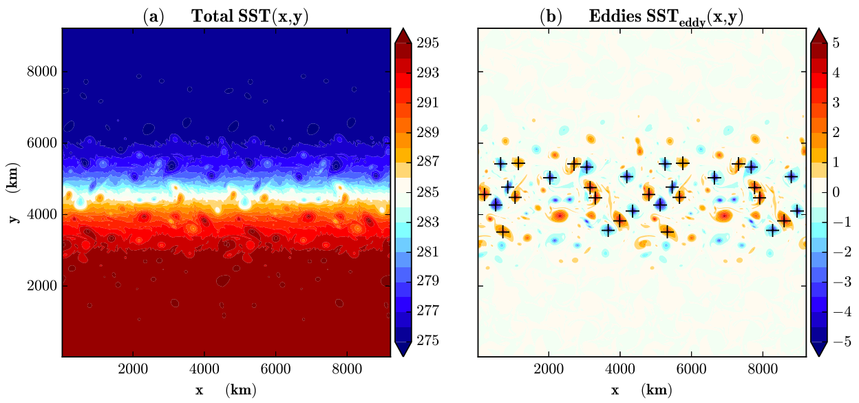
650 FIG. 1. (a) Total SST and (b) eddy SST fields, in K. In (b), black crosses mark centers of the eddies used to 651 create composites.
