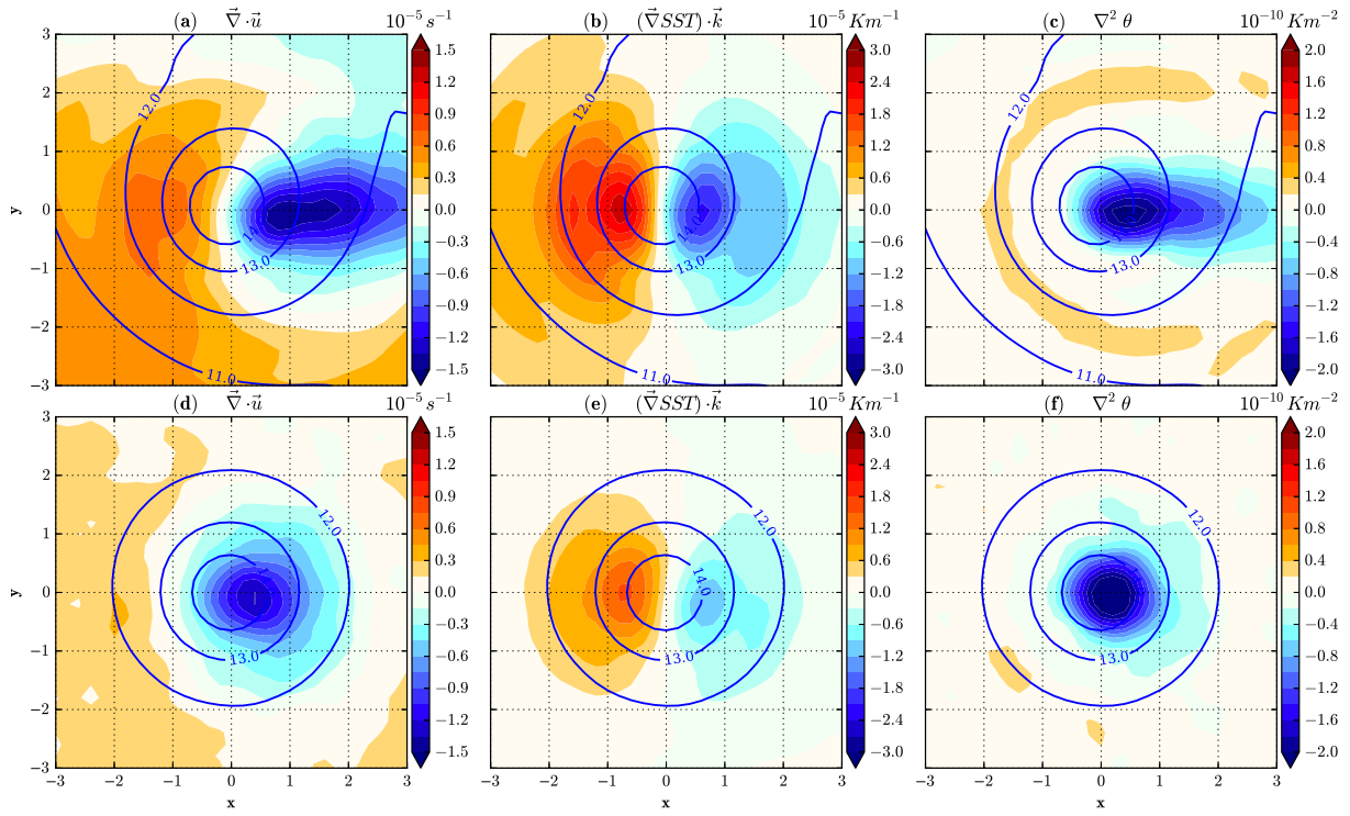
656 FIG. 4. Composites above warm eddies of (a, d) divergence of surface wind, (b, e) downwind SST gradient 657 and (c, f) Laplacian of boundary layer temperature. (a-c) strong-wind conditions and (d-f) weak-wind conditions. 658 Contours correspond to SST (in K).
