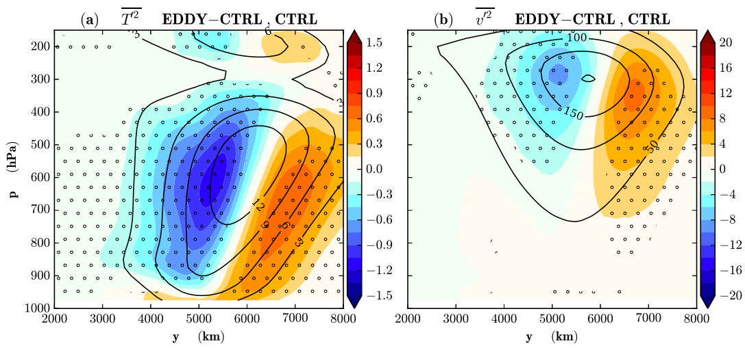
725 FIG. 7. Same as Fig. 5, but for zonal and time average of (a) \langle \overline{T'T'} \rangle (in \text{K}^2 ) and (b) \langle \overline{v'v'} \rangle (in \text{m}^2\text{s}^{-2} ). Regions 726 with significant variance differences are shaded with black dots.
