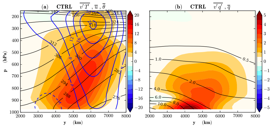
708 FIG. 3. Storm-track properties of the CTRL experiment. (a) Zonal wind (blue contours, in \text{m s}^{-1} ), 2-10 days 709 filtered meridional flux of temperature (shadings, in \text{K m s}^{-1} ) and potential temperature (black contours, in 710 K). (b) Specific humidity (contours, in \text{g kg}^{-1} ) and (2-10 days filtered) meridional flux of specific humidity 711 (shadings, in \text{g kg}^{-1} \text{ m s}^{-1} ).
