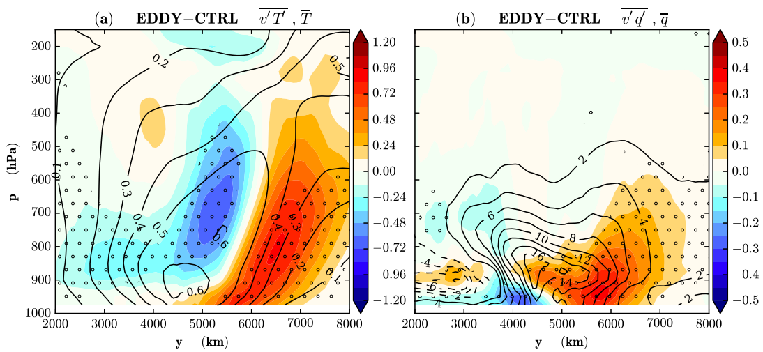
721 FIG. 6. In shadings, differences between EDDY and CTRL, for the zonal and time average of (a) \langle \overline{v'T'} \rangle (in 722 \text{K m s}^{-1} ) and (b) \langle \overline{v'q'} \rangle (in \text{g kg}^{-1} \text{ m s}^{-1} ). In contours, zonal and time average of EDDY-CTRL difference (a) 723 temperature (in K), (b) specific humidity (in 10^{-2} \text{ g kg}^{-1} ). Regions with significant differences in \langle \overline{v'T'} \rangle or 724 \langle \overline{v'q'} \rangle are shaded with black dots.
