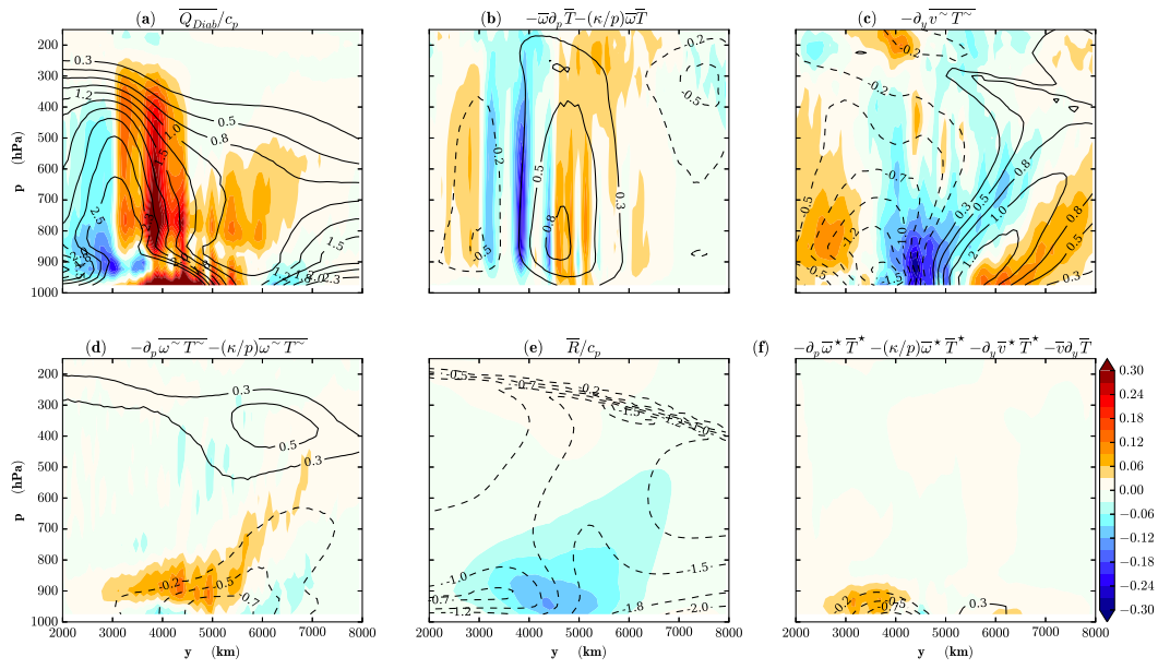
727 FIG. 8. Zonal and time average of terms in the temperature budget (Eq. 2), in \text{K day}^{-1} . Shadings: Differences 728 between EDDY and CTRL . Contours: CTRL.
