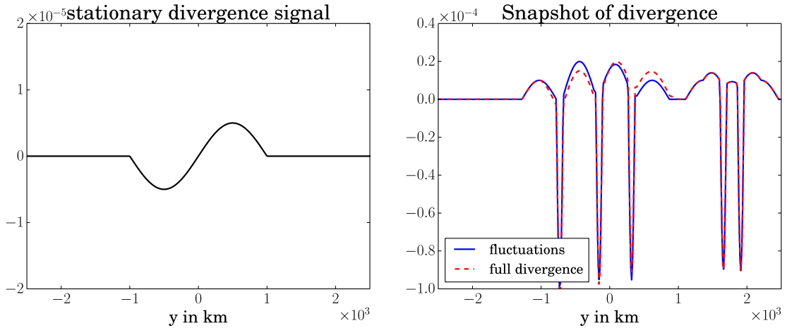
FIG. 1. (left) The stationary divergence d_p(y) ( s^{-1} ). (right) Snapshot of the fluctuating component d_s(y, t) (blue line; s^{-1} ) and of the resulting full divergence signal d(y, t) (red dashed line; s^{-1} ). Note the different vertical scale relative to (left).
