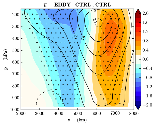
718 FIG. 5. Zonal and time average of zonal wind (in \text{m s}^{-1} ). In contours, CTRL experiment. In shadings, 719 differences between EDDY and CTRL. Zonal wind differences which are significant at the 95% level are shaded 720 by black dots.
