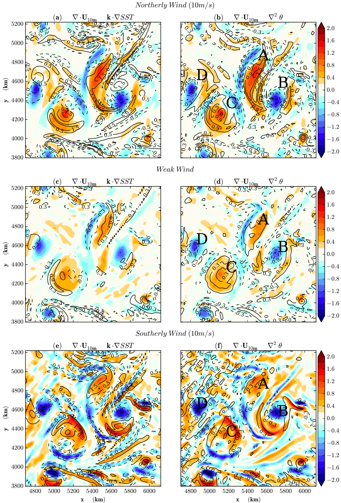
659 FIG. 6. Composites of surface divergence (in 10^{-5} \text{ s}^{-1} ) for days with (a-b) northerly winds, (c-d) weak winds, 660 and (e, f) southerly winds. In (a, c, e), contours correspond to downwind SST gradient (in 10^{-5} \text{ K m}^{-1} ). In (b, 661 d, f), contours correspond to Laplacian of atmospheric boundary layer temperature (in 10^{-10} \text{ K m}^{-2} ) (b,d,f).
