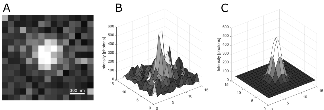
Figure 4.2: Gaussian fitting of the intensity profile of a single emitter. (A) Single molecule detected on an EMCCD camera during a PALM experiment. (B) Surface representation of the intensity profile of the single molecule. (C) Gaussian fit to the intensity profile, from which the position of the molecule can be determined with \sim 20 nm accuracy.
