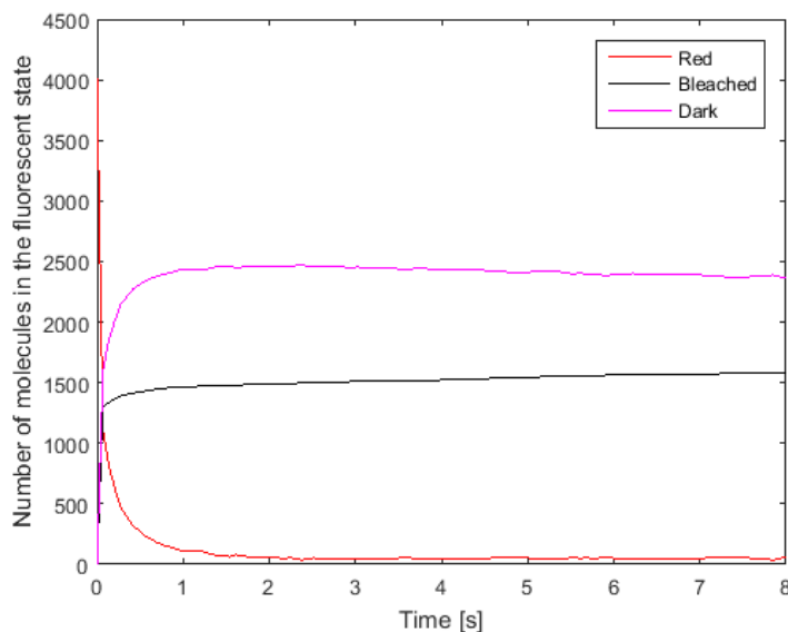
Figure 8.6: Ensemble fluorescence decay and population of dark and bleached states reconstituted from single-molecule data.
