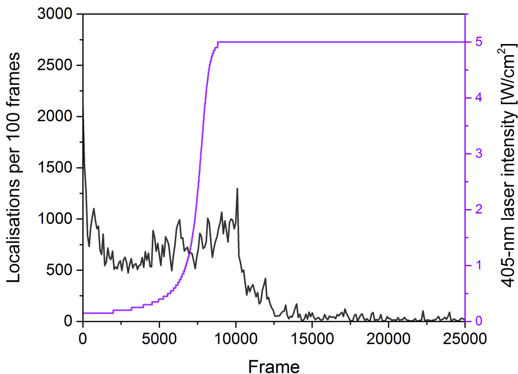
Figure 12.7: Application of a Fermi activation profile on LdcI-mEos4b fusion proteins. The maximum 405-nm laser intensity at the sample (reached after \sim 10000 frames) was 5 \text{ W/cm}^2 .
