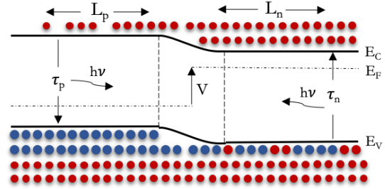
Figure 19. a) pn homojunction band diagram without bias. b) pn homojunction band diagram under forward bias V_{bias} .
