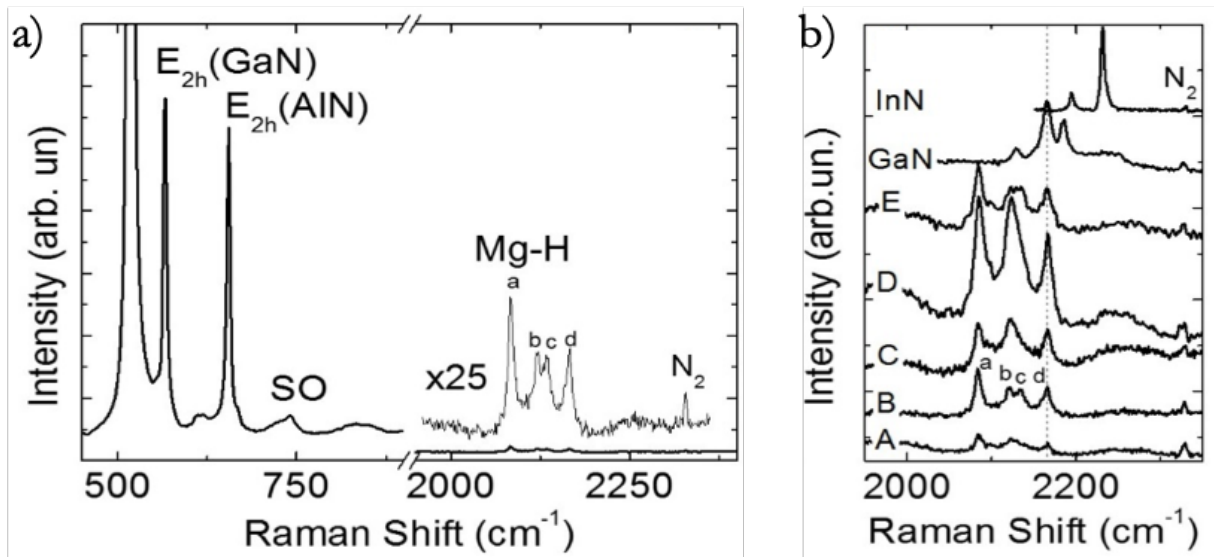
Figure 69. a) Raman spectrum of sample B (N3048) showing the spectral range corresponding to E_{2h} and Mg-H modes. The intensity of the Mg-H modes has been multiplied by 25 for clarity. b) Detail of the spectral range corresponding to the Mg-H modes of samples A to E. GaN NW and InN bulk Mg doped references have also been included.
