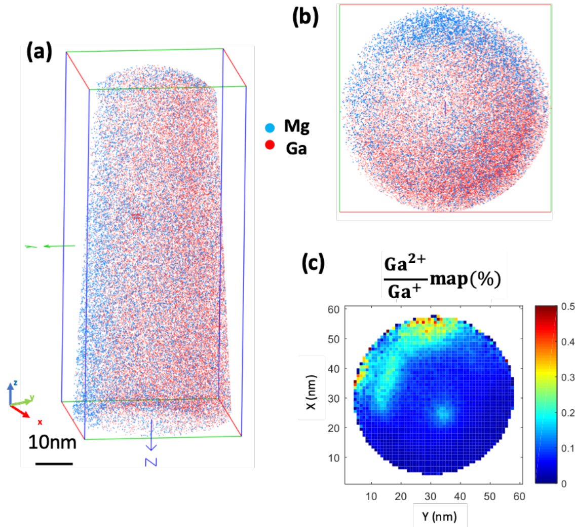
Figure 48. a) 3D volume and b) top view of atom probe tomography of Mg (blue) and Ga (red) atoms in sample #2 (without rotation) showing an inhomogeneous distribution. c) Ga^{2+}/Ga^+ map ratio showing spatial variations in the evaporation field partially corresponding to the spatial inhomogeneity in the Mg distribution.
