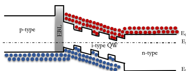
Figure 21. a) Heterojunction under forward bias and b) pin multi-quantum well structure with an EBL.
