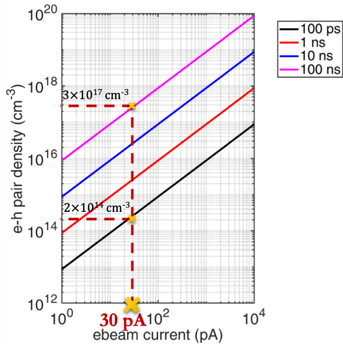
Figure 64. Injection conditions for the \text{Al}_{0.6}\text{Ga}_{0.4}\text{N} sample for 6\text{keV} acceleration voltage depending on the lifetime.
