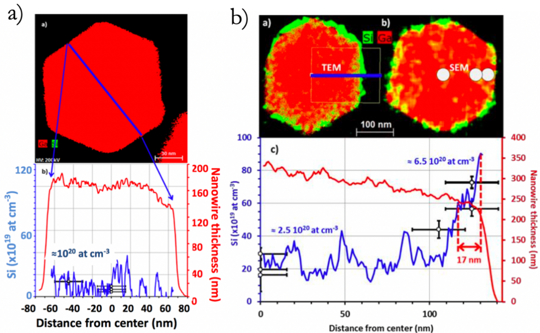
Figure 42. a) Top view cross section HR-EDX on individual Si-doped GaN nanowire doped at a doping cell temperature of 938^{\circ}\text{C} and diametral Si concentration profiling corresponding to Si concentration of 10^{20} at \text{cm}^{-3} . b) Top view cross section HR-EDX in TEM and SEM on individual Si-doped GaN nanowire doped at a doping cell temperature of 950^{\circ}\text{C} and diametral Si concentration profiling showing a Si segregation (Fang et al. 2015).
