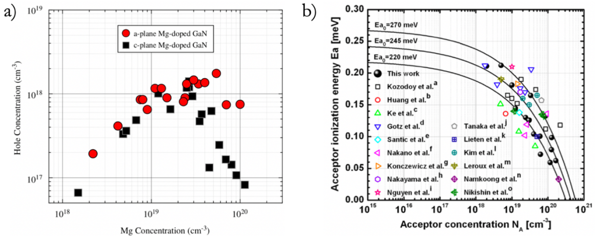
Figure 41. a) Hole concentration variation as a function of Mg concentration on a-plane (red) and c-plane (black) Mg-doped GaN epilayers (Iida et al. 2010). b) Acceptor ionization energy decreasing with acceptor concentration on MBE grown c-plane GaN (Brochen et al. 2013).
