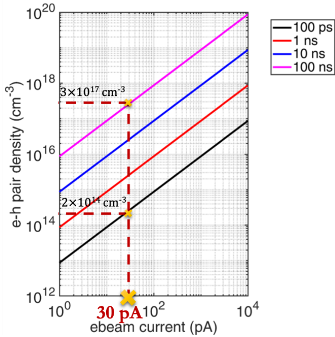
Figure 64. Injection conditions for the Al_{0.6}Ga_{0.4}N sample for 6kV acceleration voltage depending on the lifetime.
