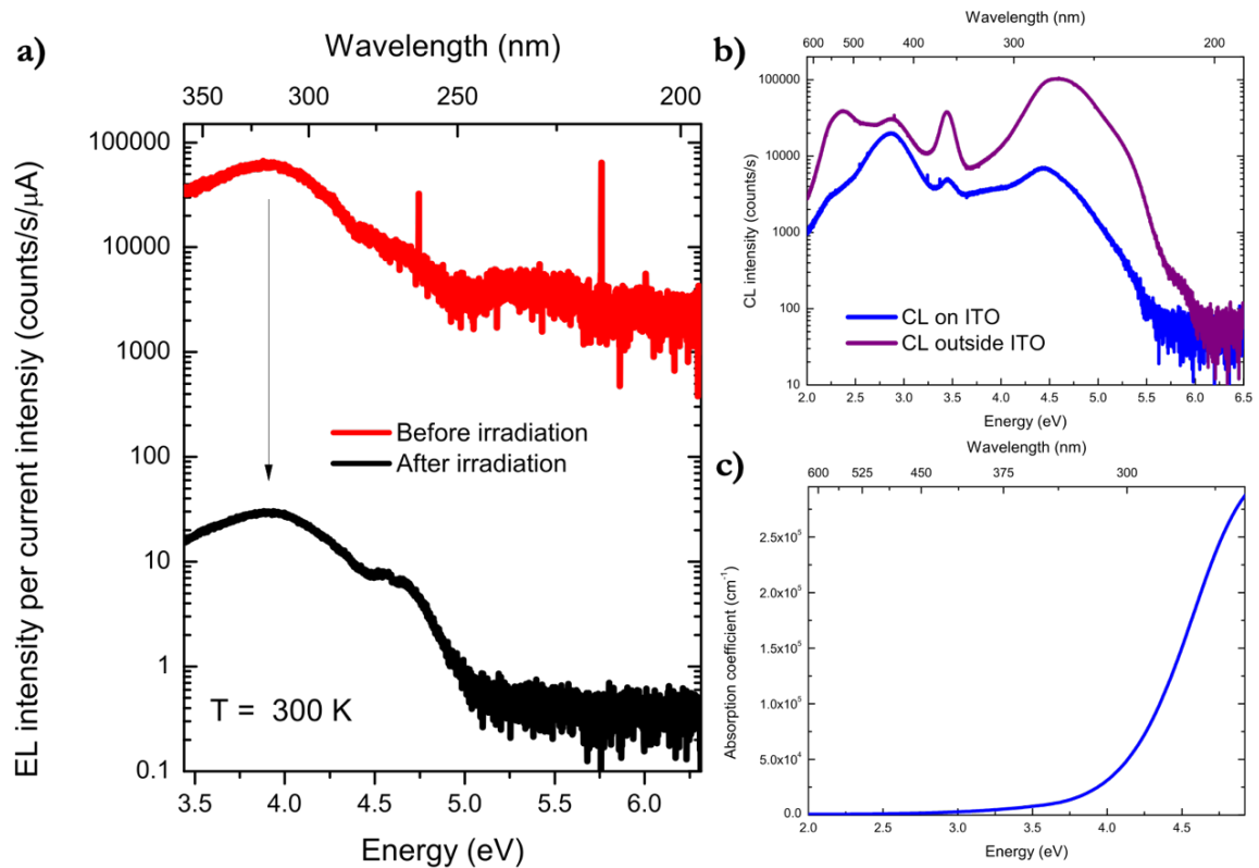
Figure 89. a) Electroluminescence spectrum of sample E recorded before and after irradiation showing deep-defect emission within p -type AlN. b) Cathodoluminescence on ITO (blue) and outside ITO (purple) explaining the lost in EL intensity for energies above 3.5 eV. c) ITO absorption coefficient variation as a function of energy.
