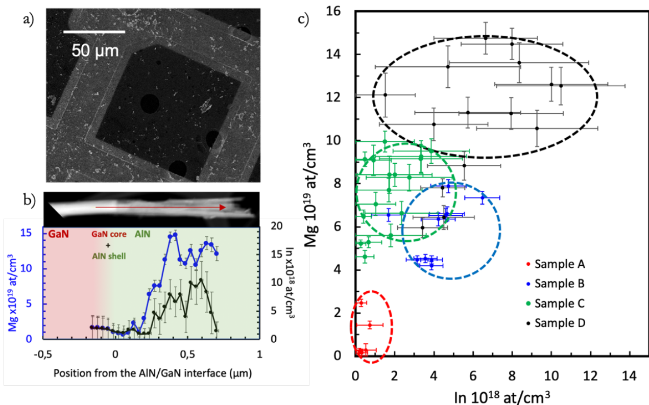
Figure 67. a) TEM grid NW dispersion b) TEM picture of dispersed nanowires from sample D (N3068) and corresponding Mg (blue axis to the left) and In (black axis to the right) profiles along the growth axis. Mg and In profiles follow the same tendency, associated to incorporation of Mg in presence of In atoms. Note that the axis is expressed in 10^{19} at. cm^{-3} for Mg and 10^{18} at. cm^{-3} for In, respectively. c) Mg and In concentration in samples A to D.
