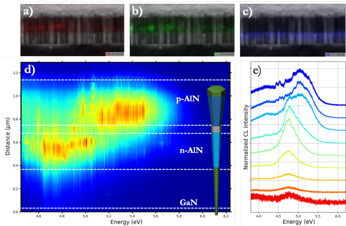
Figure 73. Optical characteristics of the AlN pin junction sample N3209 at T=300 K. a-c) Monochromatic cathodoluminescence mapping at different energies a) 5 eV, b) 4.75 eV, c) 3.45 eV. d) Cathodoluminescence mapping along the pn junction at T=5 K and nanowire schematic delimiting the different regions. e) Normalized cathodoluminescence spectra for different position along a nanowire (spectra have been shifted for clarity).
