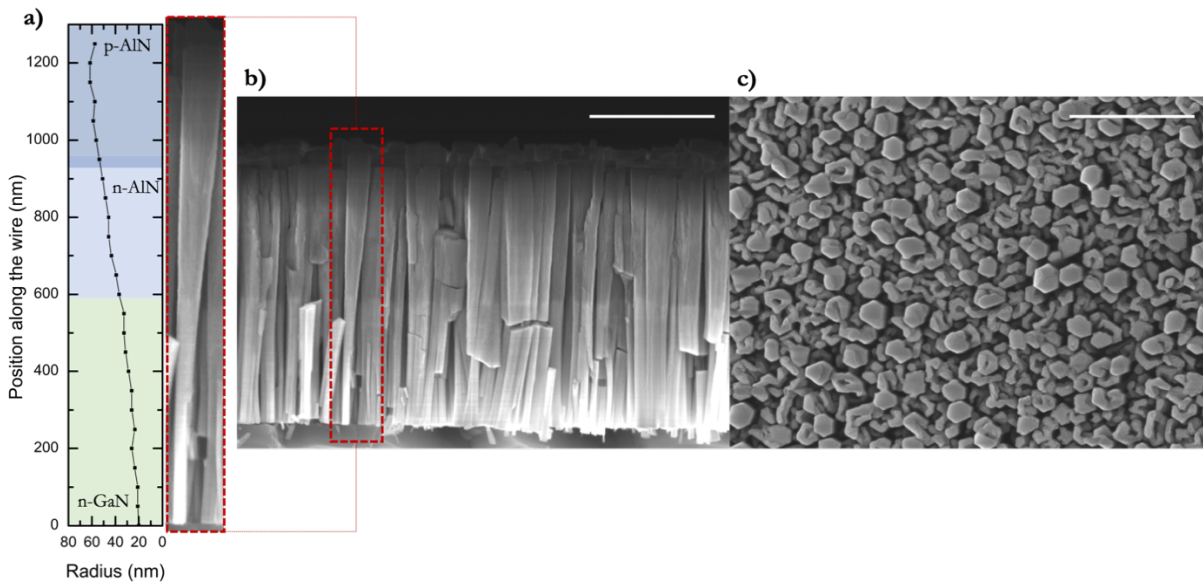
Figure 72. a) Radius dimension of an individual nanowire of sample N3209. SEM images of sample N3209 in b) side view and c) top view. The scale is of 500 nm.
