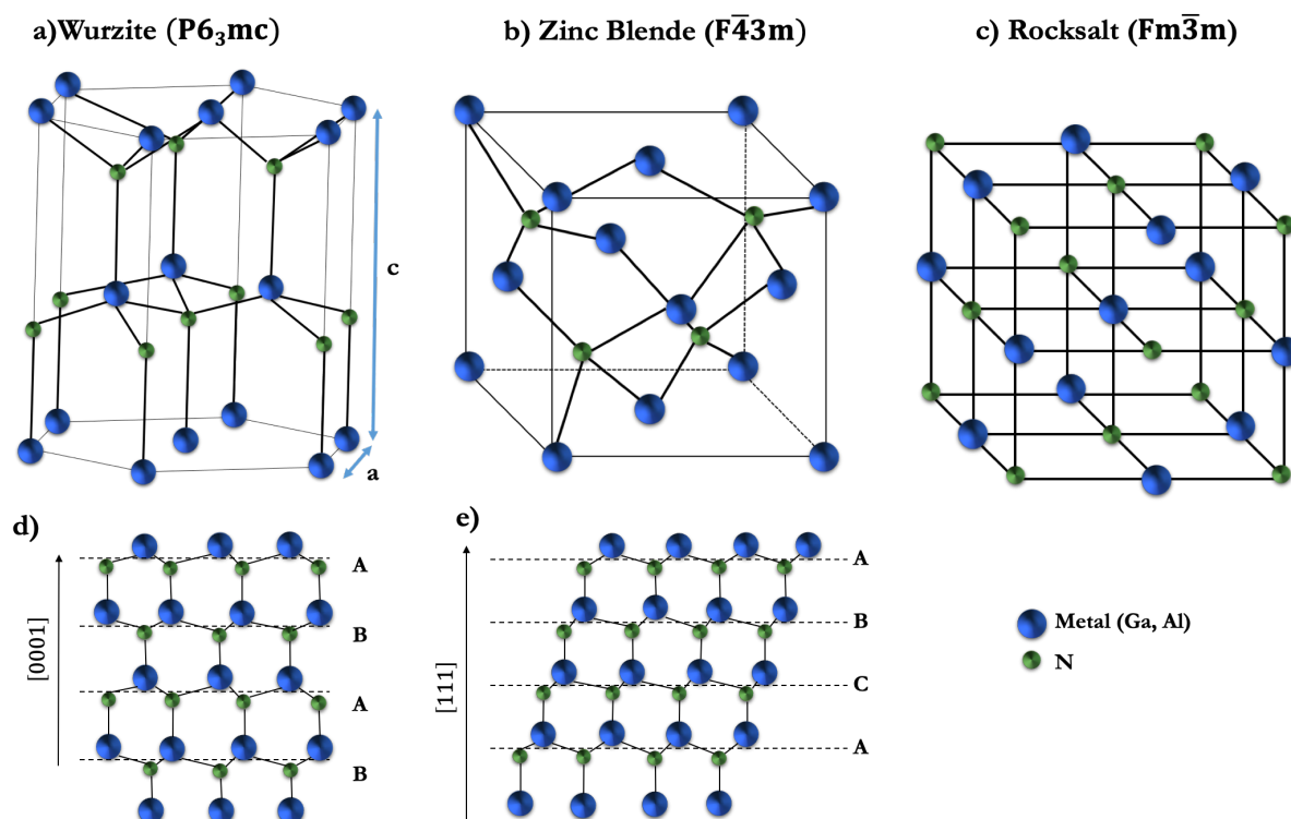
Figure 8. Crystal structure of III-N materials: a) Wurzite, b) Zinc-blende, c) Rocksalt structure d) Plane stacking in wurzite structure, e) Plane stacking in zinc-blende structure. Nitrogen atoms are represented in green and metal atoms in blue.
