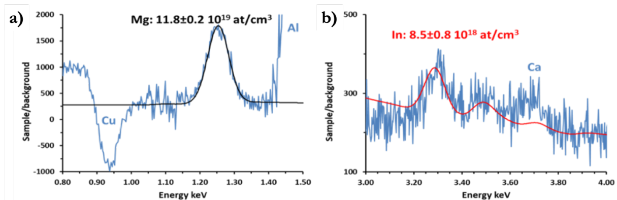
Figure 68. Normalized spectrum of sample D. a) Mg peak intensity is clearly depicted from noise level and can be quantified to a level of around 1 \times 10^{20} at.cm -3 . b) In peak intensity can be quantified to a level of around 9 \times 10^{18} at.cm -3 .
