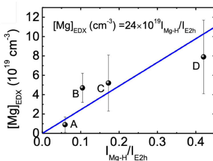
Figure 70. [\text{Mg}] content of samples A, B, C and D determined by EDX compared with the normalized Mg-H Raman mode intensities. The full line is a linear fit to the data.
