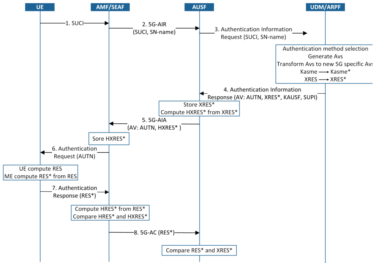
Figure 2.7– The 5G-AKA procedure. The computation of the RES * in the ME (Mobile Equipment) is in the same way as the computation of the XRES * in the ARPF. The computation of the HRES * in the SEAF is in the same way as the computation of the HXRES * in the AUSF.
