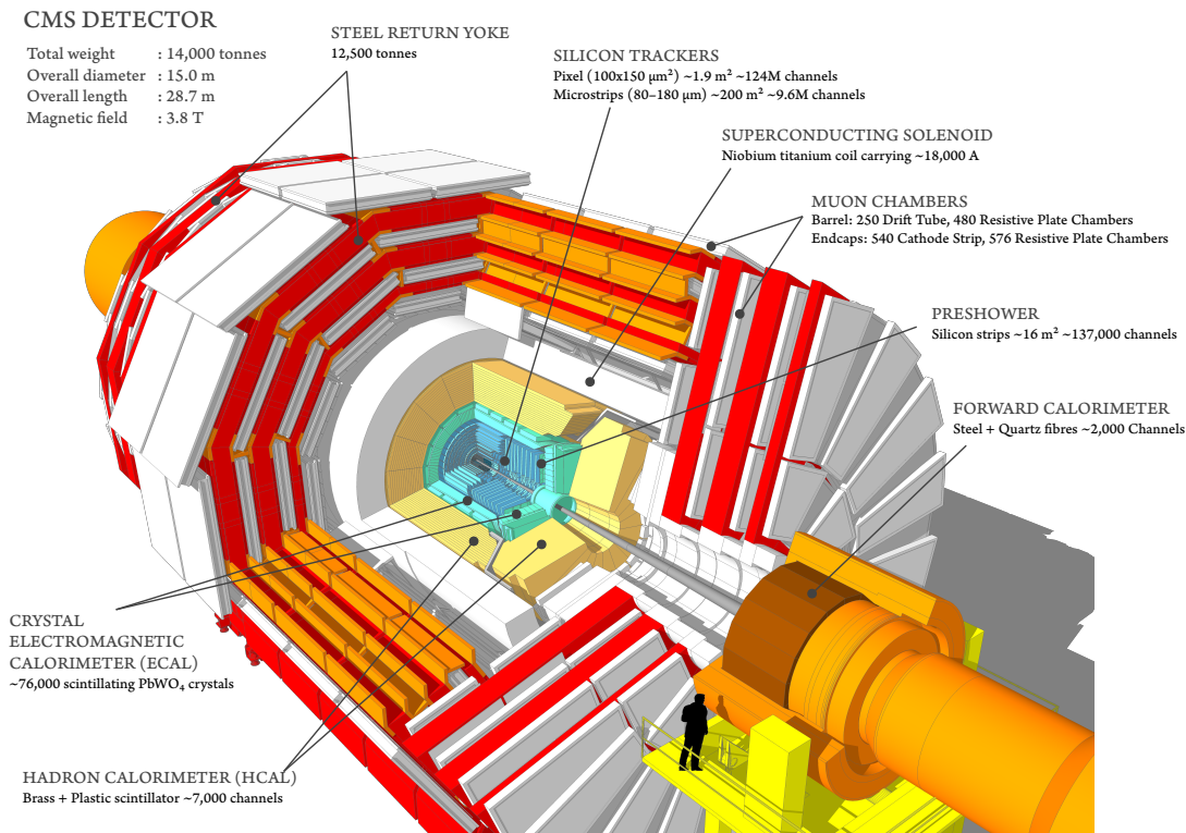
Figure 2.7 – Schematic view of the CMS detector [62].
