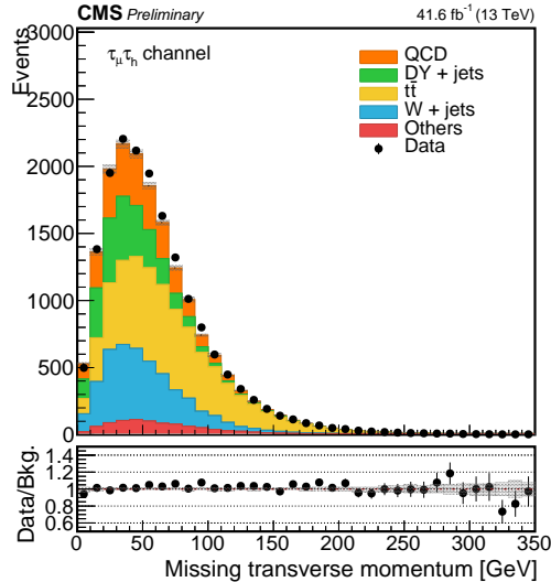
Figure 4.15 – Missing transverse momentum in \tau_\mu\tau_h events. The error bars along y for the data distribution and for the data-over-background ratio are too small to be appreciated.
