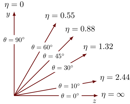
Figure 2.6 – Illustration of the relation between the pseudorapidity \eta and the polar angle \theta [61].
