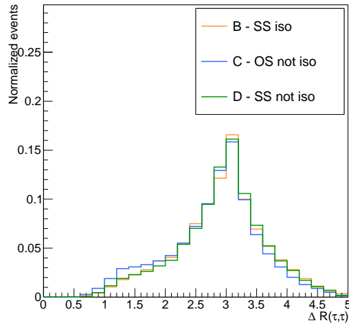
Figure A.9 – Normalised h_{data} - h_{MC} distributions as a function of \Delta R(\tau_h, \tau_h) in the B, C and D regions of the ABCD method (Sec. 5.3). The events are required to pass the baseline selection, i.e. to pass the \tau_h \tau_h selection and to have two b jet candidates.
