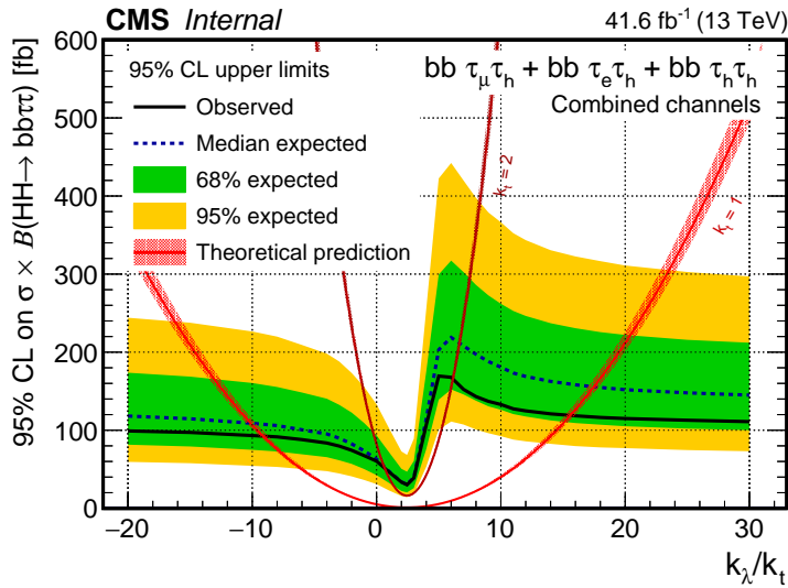
Figure 6.2 – 95% CL upper limits for on \sigma(\text{gg} \rightarrow \text{HH}) \cdot \text{BR}(\text{HH} \rightarrow \text{bb}\tau\tau) as a function of the ratio k_\lambda/k_t . The signal ( \sigma \cdot \text{BR} ) is normalised to 1 fb. The \pm 1\sigma and \pm 2\sigma deviations from the expected value are represented by green and yellow bands; the red curves represent the theoretical predictions for k_t = 1 and k_t = 2 .
