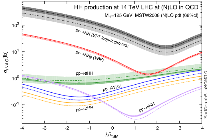
Figure 1.14 – Total cross sections at NLO precision for the six largest HH production mechanisms at proton-proton colliders as a function of the variation from the \lambda_{\text{HHH}} prediction. The thickness of the lines corresponds to the scale and PDF uncertainties added linearly [29].
