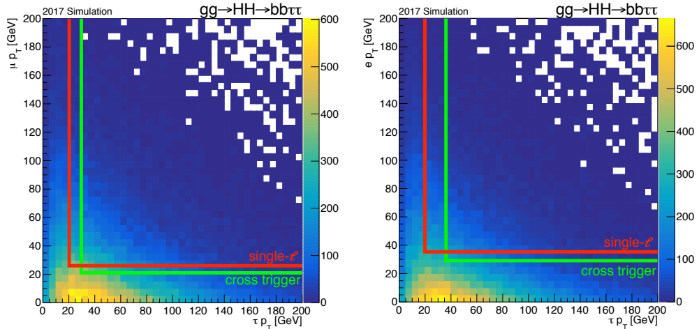
Figure 4.3 – Distribution of events from a gg \rightarrow HH \rightarrow bb\tau\tau signal sample as a function of the p_T of the muon (left) or electron (right) and the hadronic tau originated by an Higgs boson, retrieved from the generator event information. The offline thresholds allowed by the use of the single-lepton triggers are indicated in red, while those corresponding to the cross triggers are indicated in green. The number of events, expressed on the z -axis, is given in arbitrary units.
