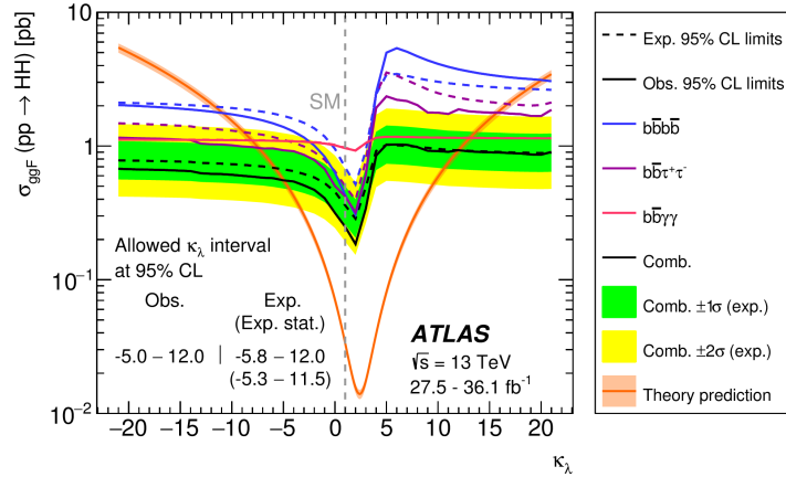
Figure 1.20 – Observed and expected upper limit at 95% CL on \sigma(\text{gg} \rightarrow \text{HH}) as a function of k_\lambda obtained in each ATLAS analysis performed with 2016 data and with their combination [48]. The \pm 1\sigma and \pm 2\sigma deviations from the expected value are shown only for the combined expected limit; they are represented by green and yellow bands.
