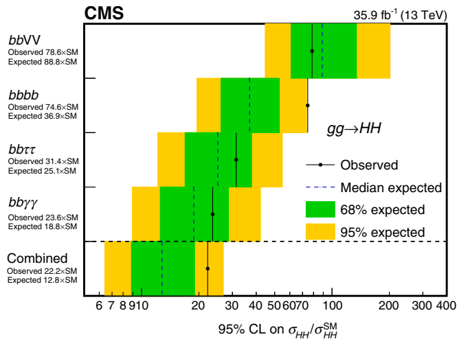
Figure 1.21 – Observed and expected upper limit at 95% CL on \sigma(\text{gg} \rightarrow \text{HH}) \cdot \text{BR} obtained in each CMS analysis performed with 2016 data and with their combination [50]. The \pm 1\sigma and \pm 2\sigma deviations from the expected value are represented by green and yellow bands.
