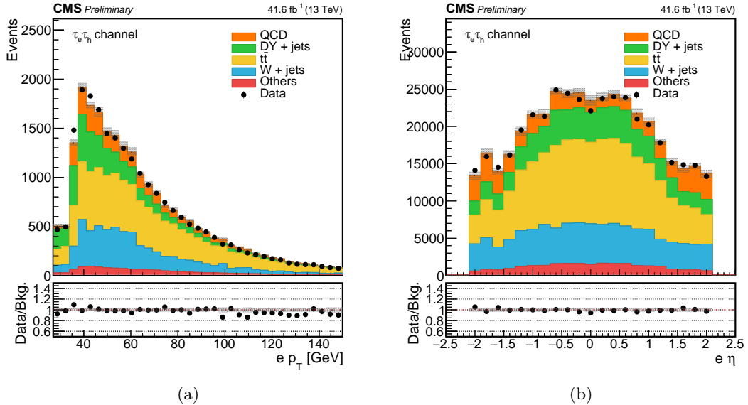
Figure 4.10 – Transverse momentum (left) and pseudorapidity (right) distributions of electrons selected in the \tau_e\tau_h final state. The error bars along y for the data distribution and for the data-over-background ratio are too small to be appreciated.
