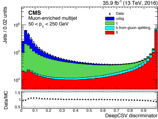
Figure 4.18 – Distribution of the DeepCSV P(b)+P(bb) discriminator value for jets of different flavours in muon enriched QCD events.[111]
