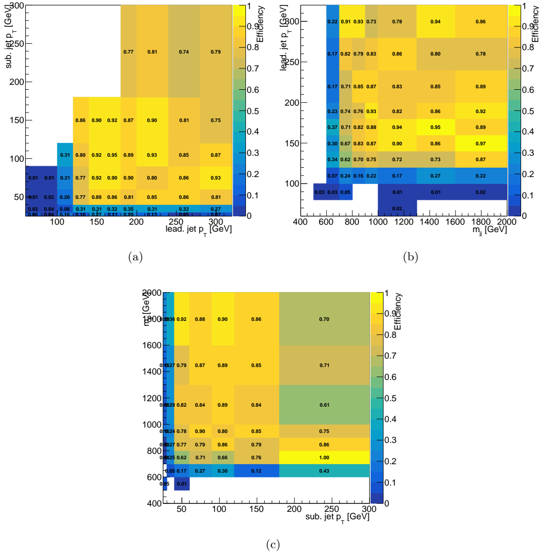
Figure 3.29 – 2D efficiencies as a function of the leading and subleading jet p_T (a), of the highest invariant mass pair m_{jj} and the leading jet p_T (b), and of the subleading p_T and the highest invariant mass pair m_{jj} (c) computed on events firing the classic di- \tau_h triggers in a 2017 VBF H \rightarrow \tau\tau simulation.
